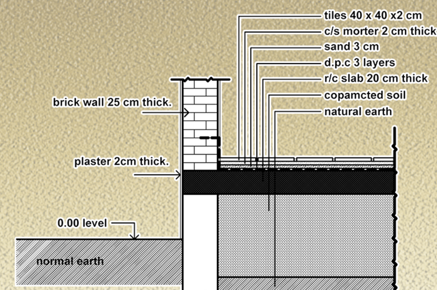
D2: SUSPENDED FLOOR DETAIL
