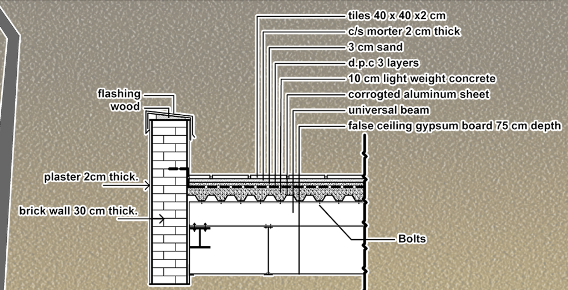
D1: ROOF DETAIL
