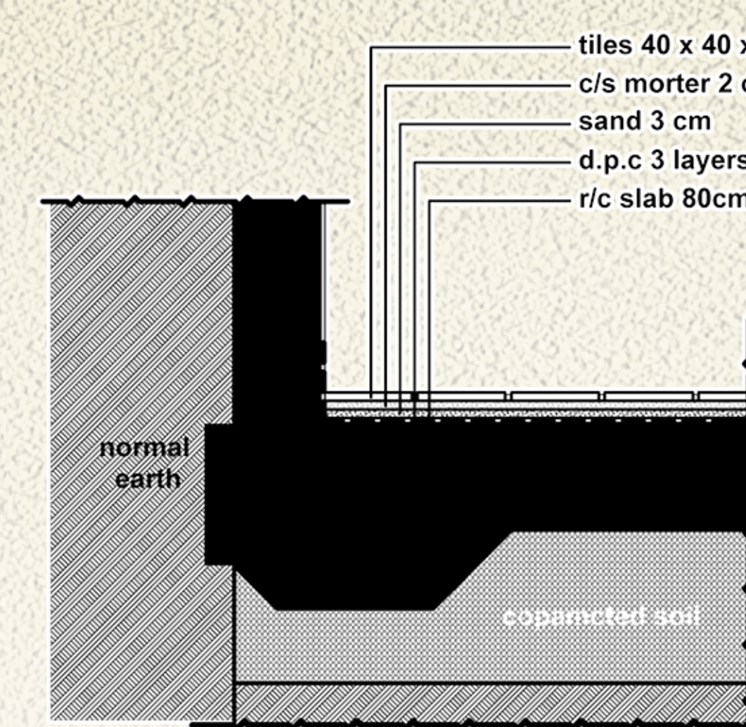
D3: RAFT FOUNDATION DETAIL
