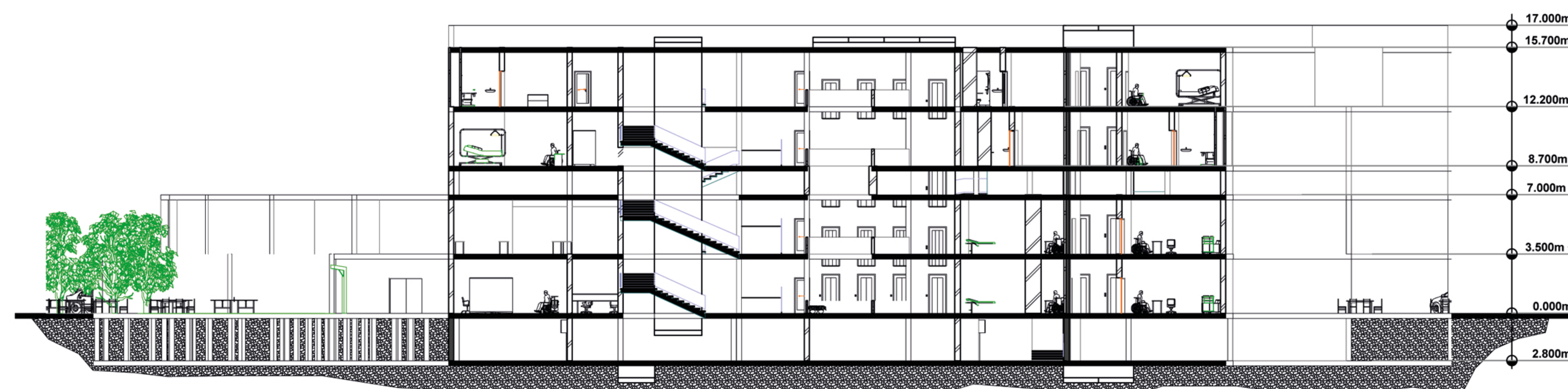
Section C-C
