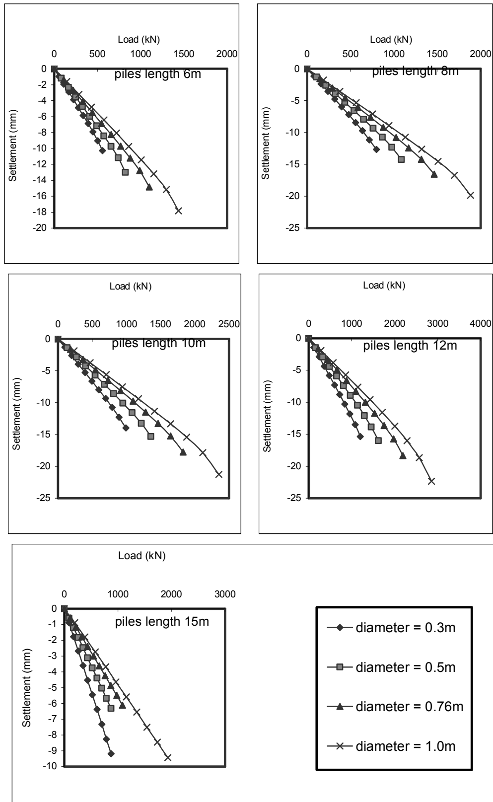
Figure B.23. Settlement-Load Relationship for Mary Cathedral Site ( Piles Lengths 6, 8, 10, 12 and 15m ).
