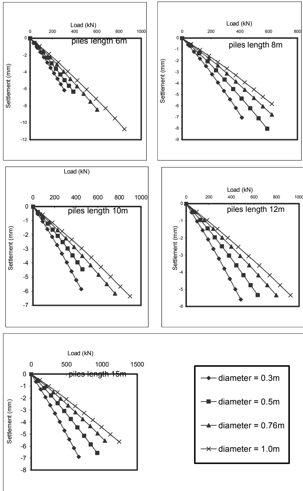
Figure B.15. Settlement-Load Relationship for White Nile Bridge Site ( Piles Lengths 6, 8, 10, 12 and 15m ).
