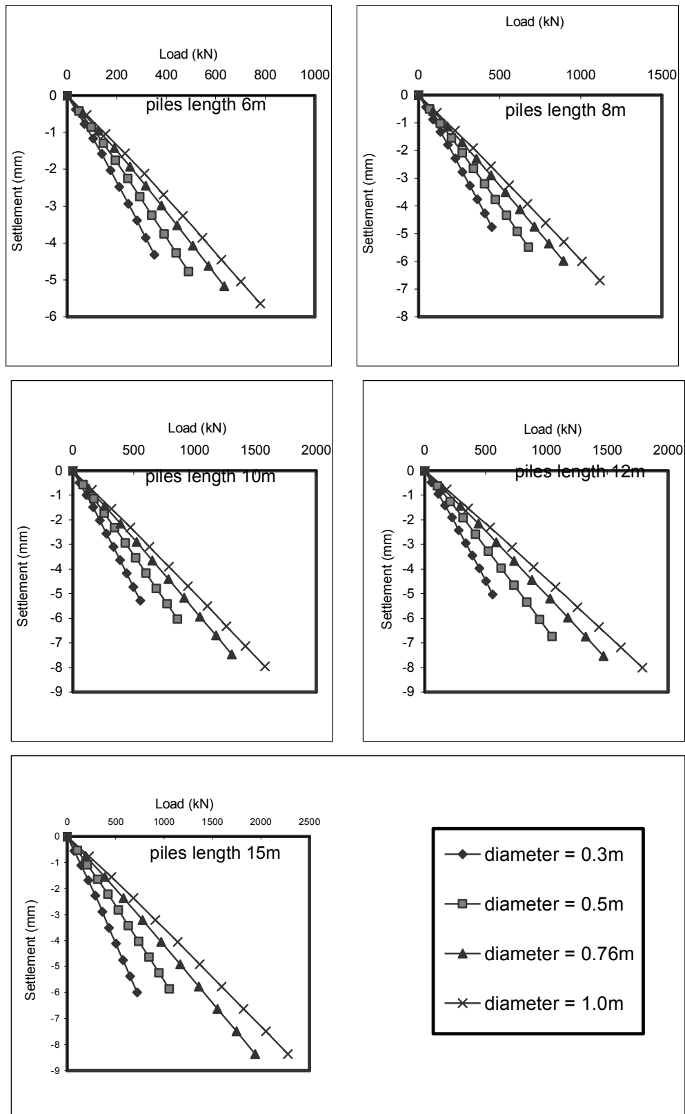
Figure B.24. Settlement-Load Relationship for Saha Alkhadra Housing Site ( Piles Lengths 6, 8, 10, 12 and 15m ).
