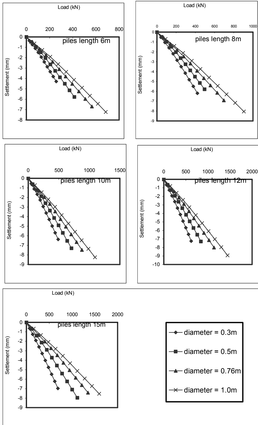
Figure B.8. Settlement-Load Relationship for Building of Custom Institute Site ( Piles Lengths 6, 8, 10, 12 and 15m ).
