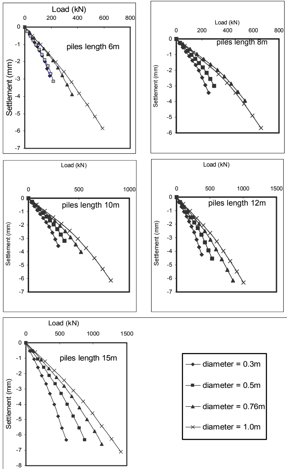
Figure B.1. Settlement-Load Relationship for Khartoum Airport Site ( Piles Lengths 6, 8, 10, 12 and 15m ).
