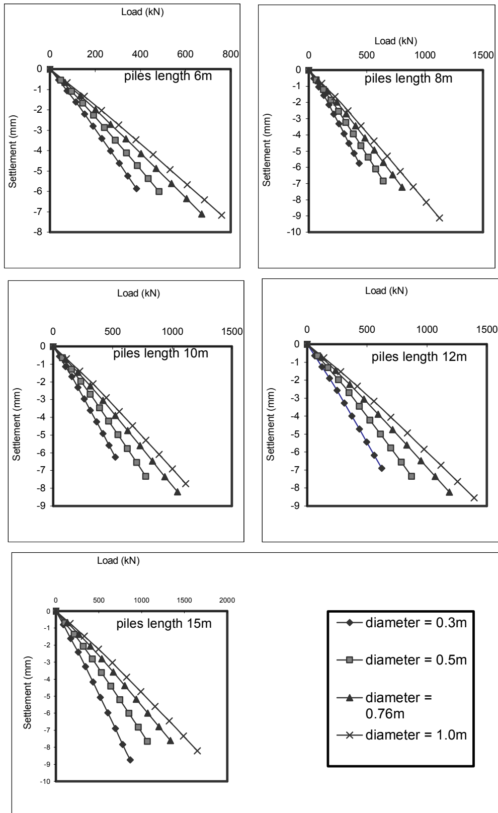
Figure B.19. Settlement-Load Relationship for Fedail Building Site ( Piles Lengths 6, 8, 10, 12 and 15m ).
