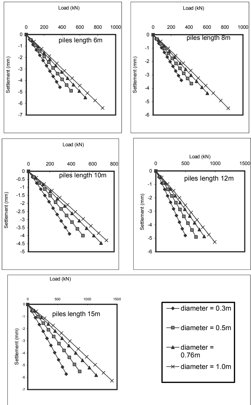
Figure B.20. Settlement-Load Relationship for Animal Resources Bank Site ( Piles Lengths 6, 8, 10, 12 and 15m ).
