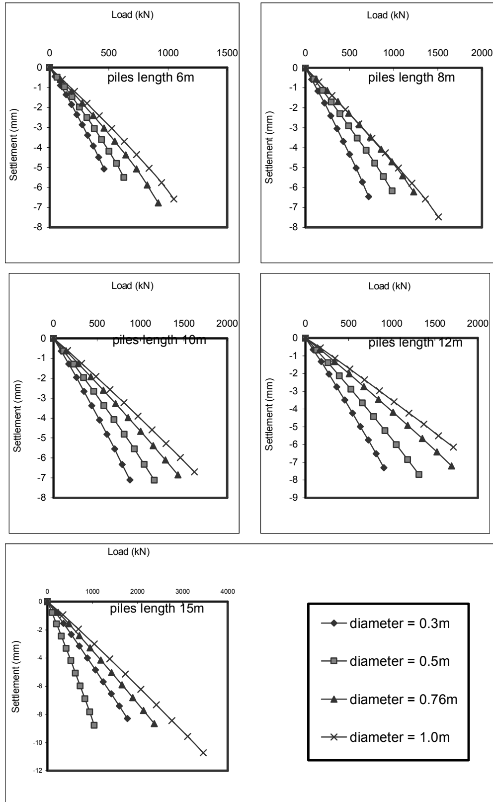
Figure B.12. Settlement-Load Relationship for Dental Hospital Khartoum Site ( Piles Lengths 6, 8, 10, 12 and 15m ).
