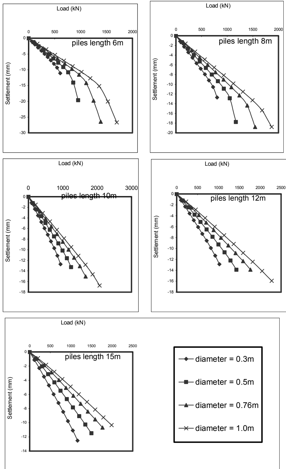
Figure B.11. Settlement-Load Relationship for N.E.C. Burri Power Station Site ( Piles Lengths 6, 8, 10, 12 and 15m ).
