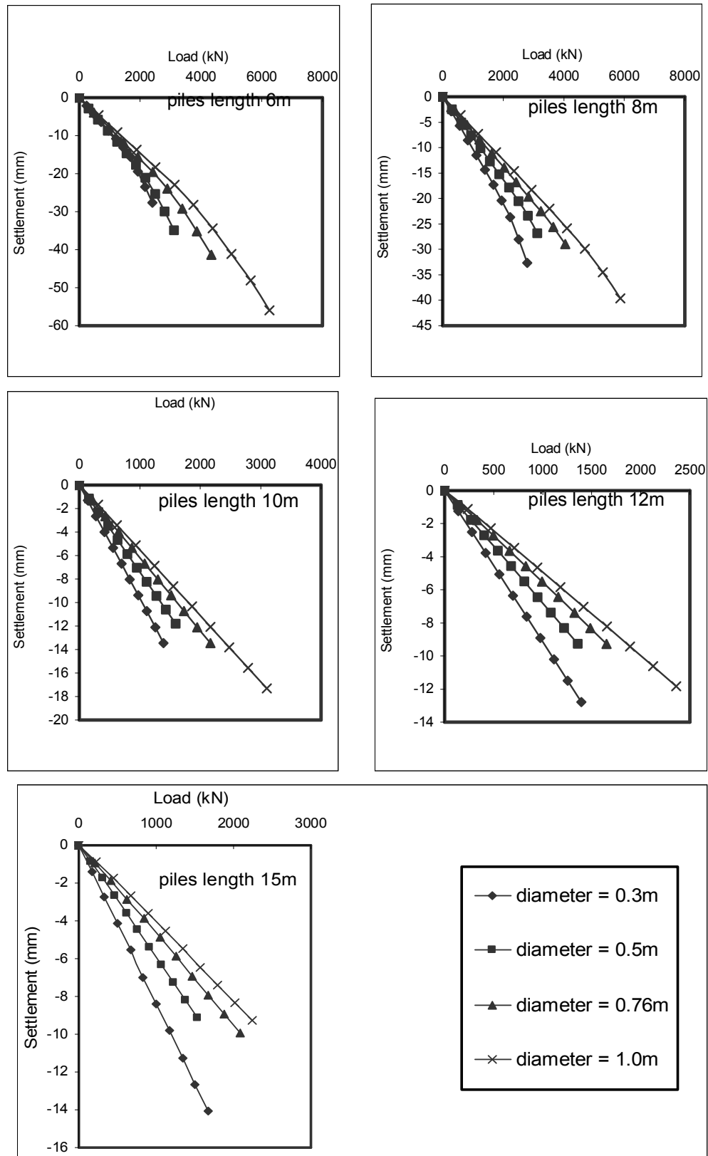
Figure B.22. Settlement-Load Relationship for Arab Company Building Site ( Piles Lengths 6, 8, 10, 12 and 15m ).
