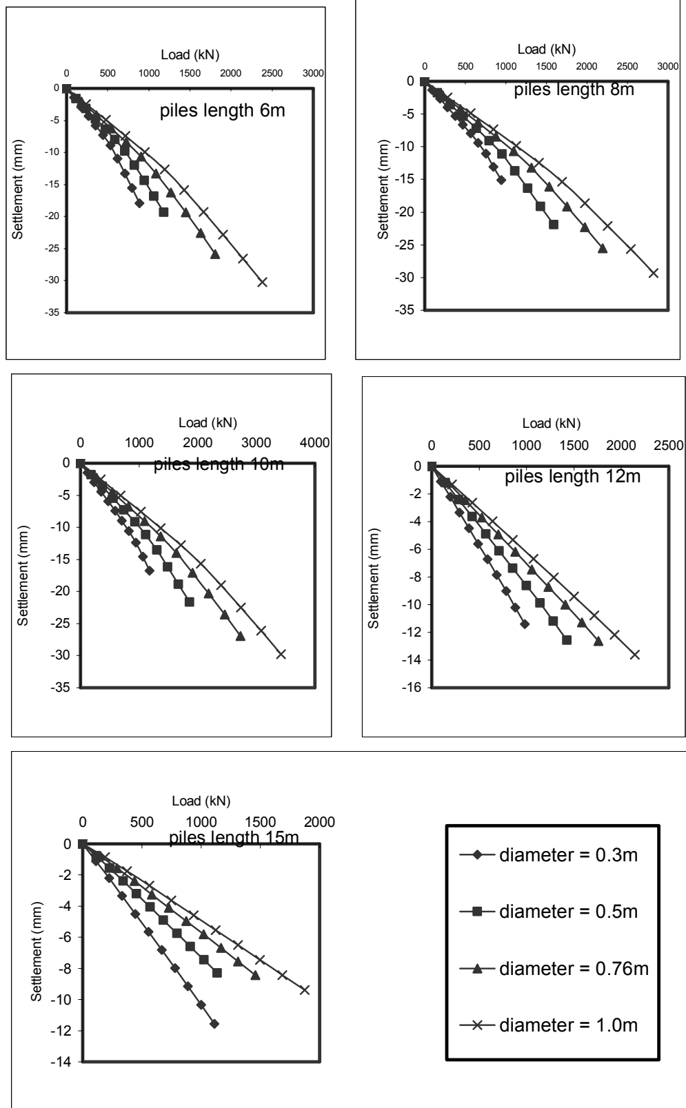
Figure B.17. Settlement-Load Relationship for Wahat Al-Khartoum Building Site ( Piles Lengths 6, 8, 10, 12 and 15m ).
