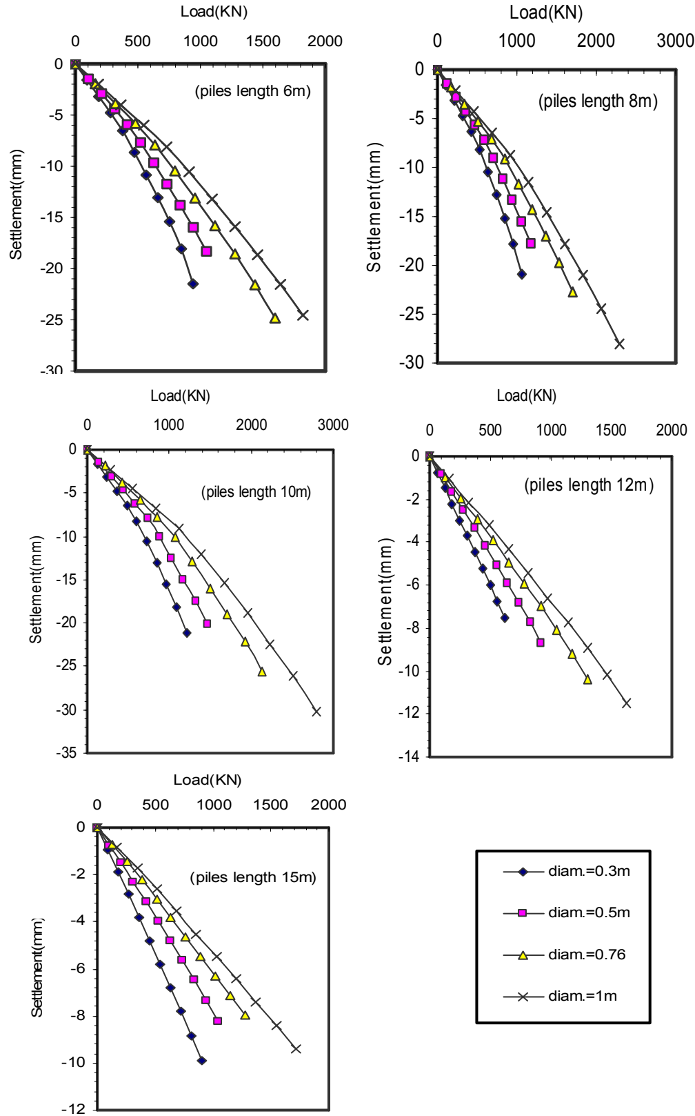
Figure B.10. Settlement-Load Relationship for N.E.C. Head Quarters Khartoum Site ( Piles Lengths 6, 8, 10, 12 and 15m ).
