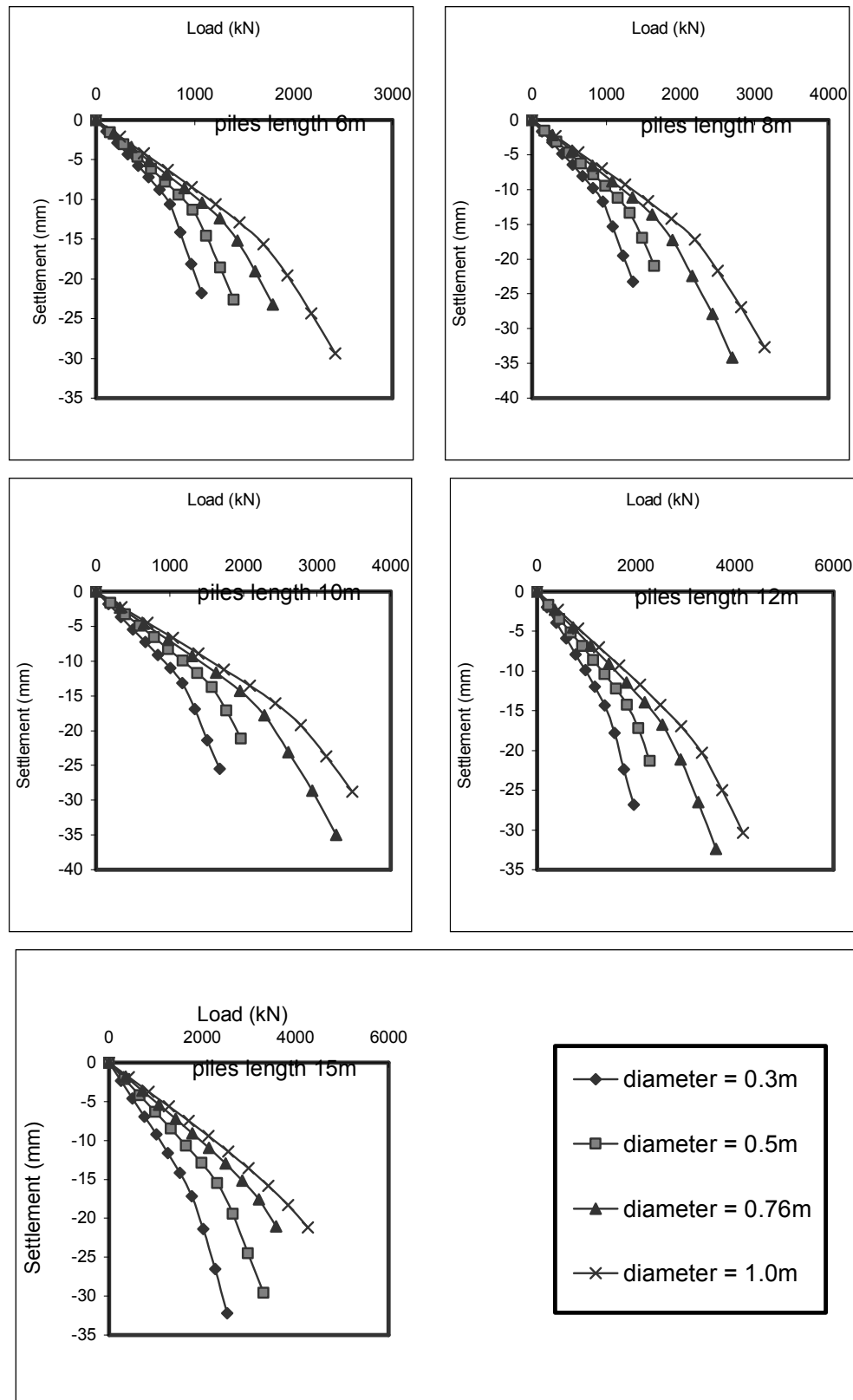
Figure B.21 Settlement-Load Relationship for Hotel & Commercial Development Site ( Piles Lengths 6, 8, 10, 12 and 15m ).
