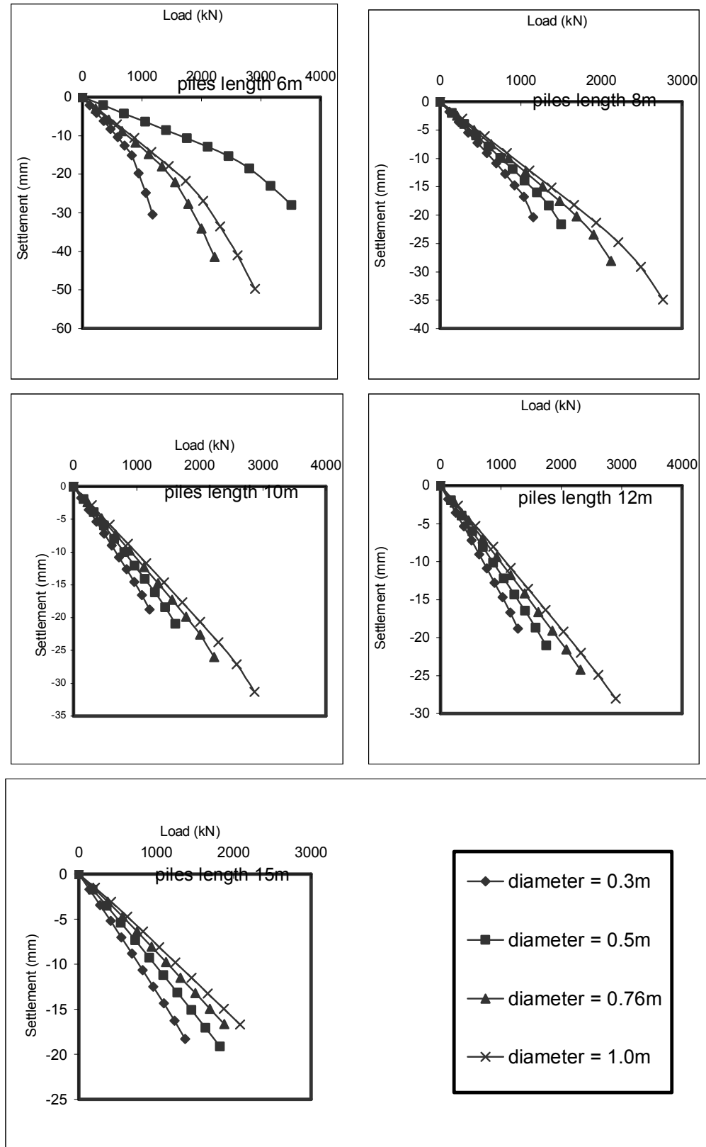
Figure B.18. Settlement-Load Relationship for Kamal Hamza Building Site ( Piles Lengths 6, 8, 10, 12 and 15m ).
