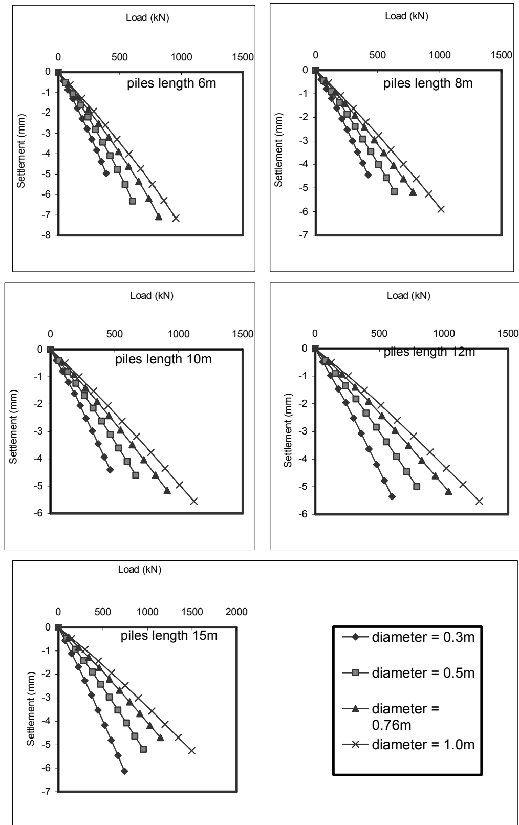
Figure B.5. Settlement-Load Relationship for Record Office at Khartoum Site ( Piles Lengths 6, 8, 10, 12 and 15m ).
