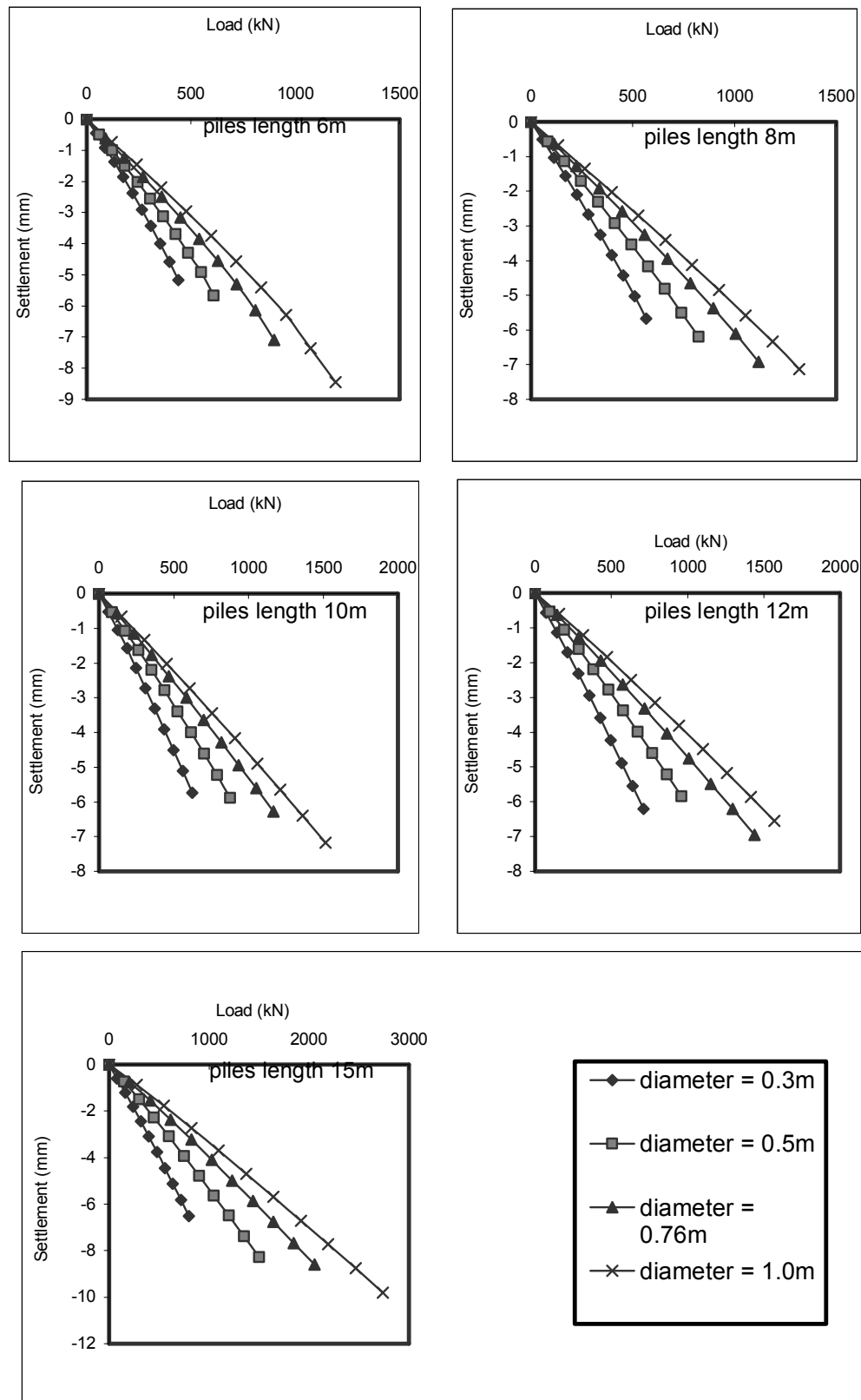
Figure B.4. Settlement-Load Relationship for Security Office at Khartoum Site ( Piles Lengths 6, 8, 10, 12 and 15m ).
