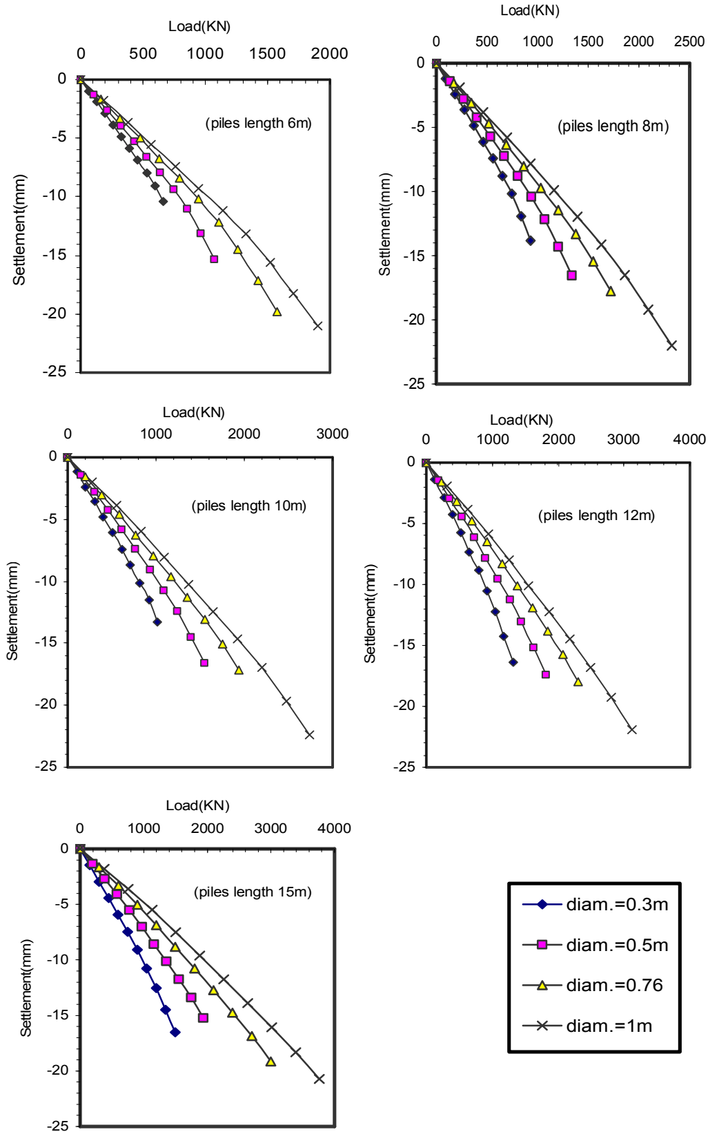
Figure 6.2. Settlement-Load Relationship for Sudanese Company Site ( Piles Lengths 6, 8, 10, 12 and 15m ).
