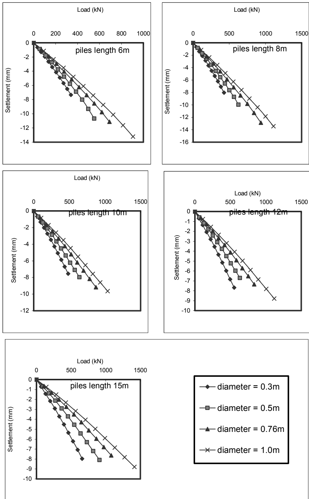
Figure B.7. Settlement-Load Relationship for Slamic Co-Operation Bank Site ( Piles Lengths 6, 8, 10, 12 and 15m ).
