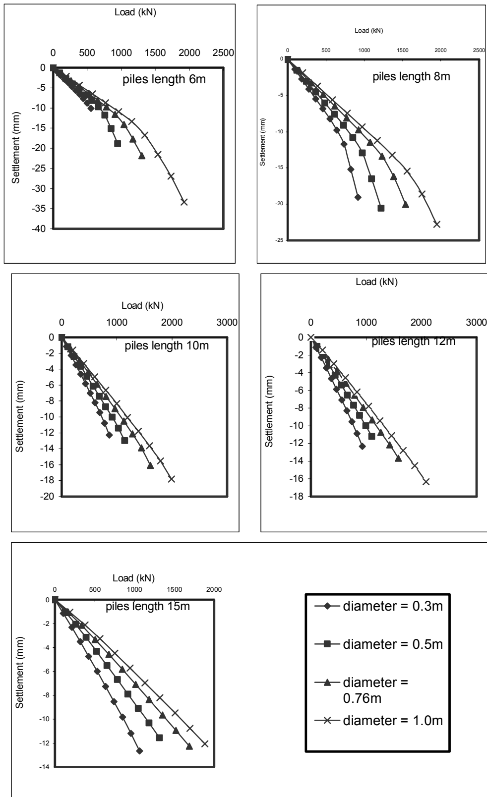
Figure B.3. Settlement-Load Relationship for Derwish Building Site ( Piles Lengths 6, 8, 10, 12 and 15m ).
