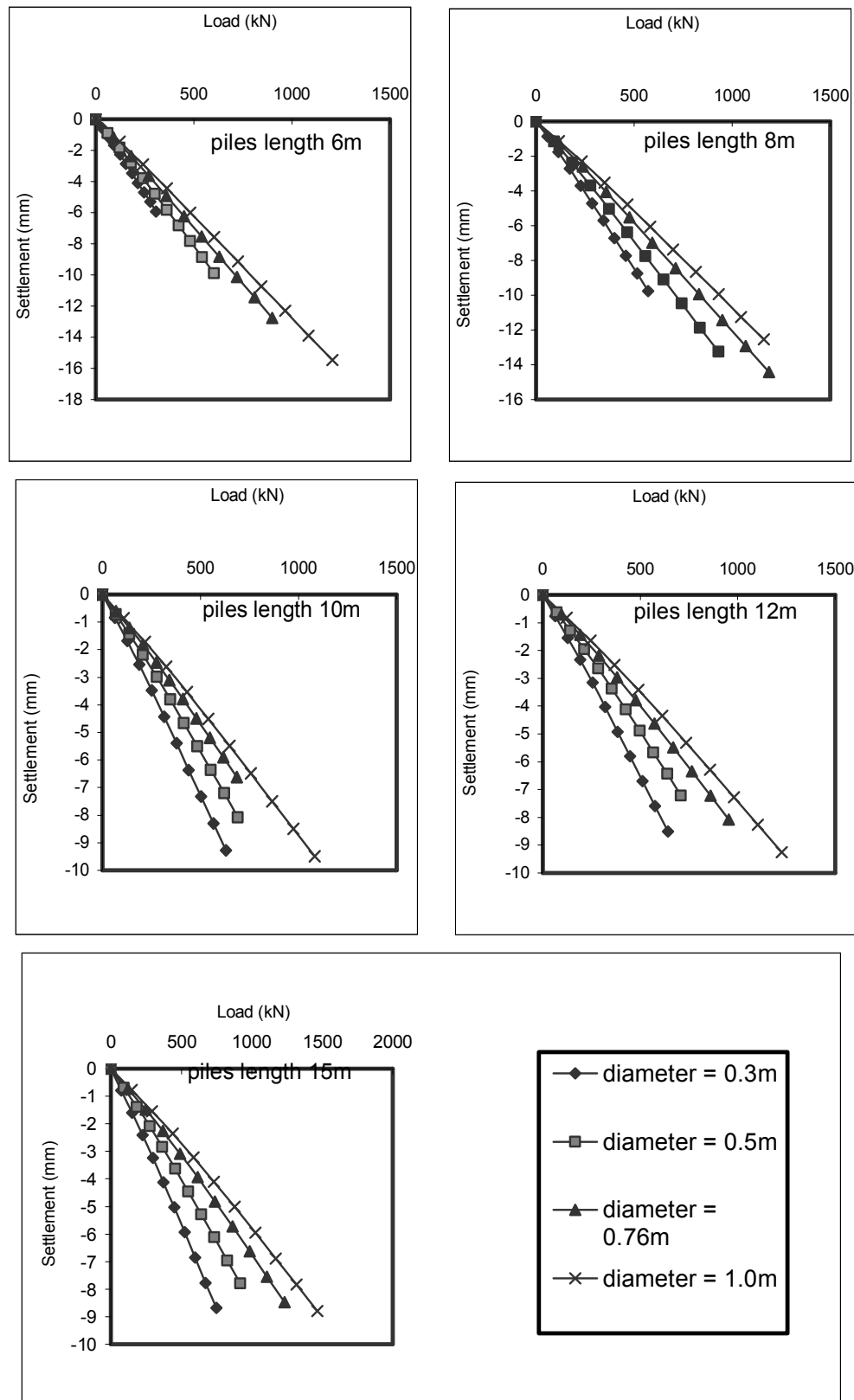
Figure B.9. Settlement-Load Relationship for Petroleum Laboratory at 61 Street Site ( Piles Lengths 6, 8, 10, 12 and 15m ).
