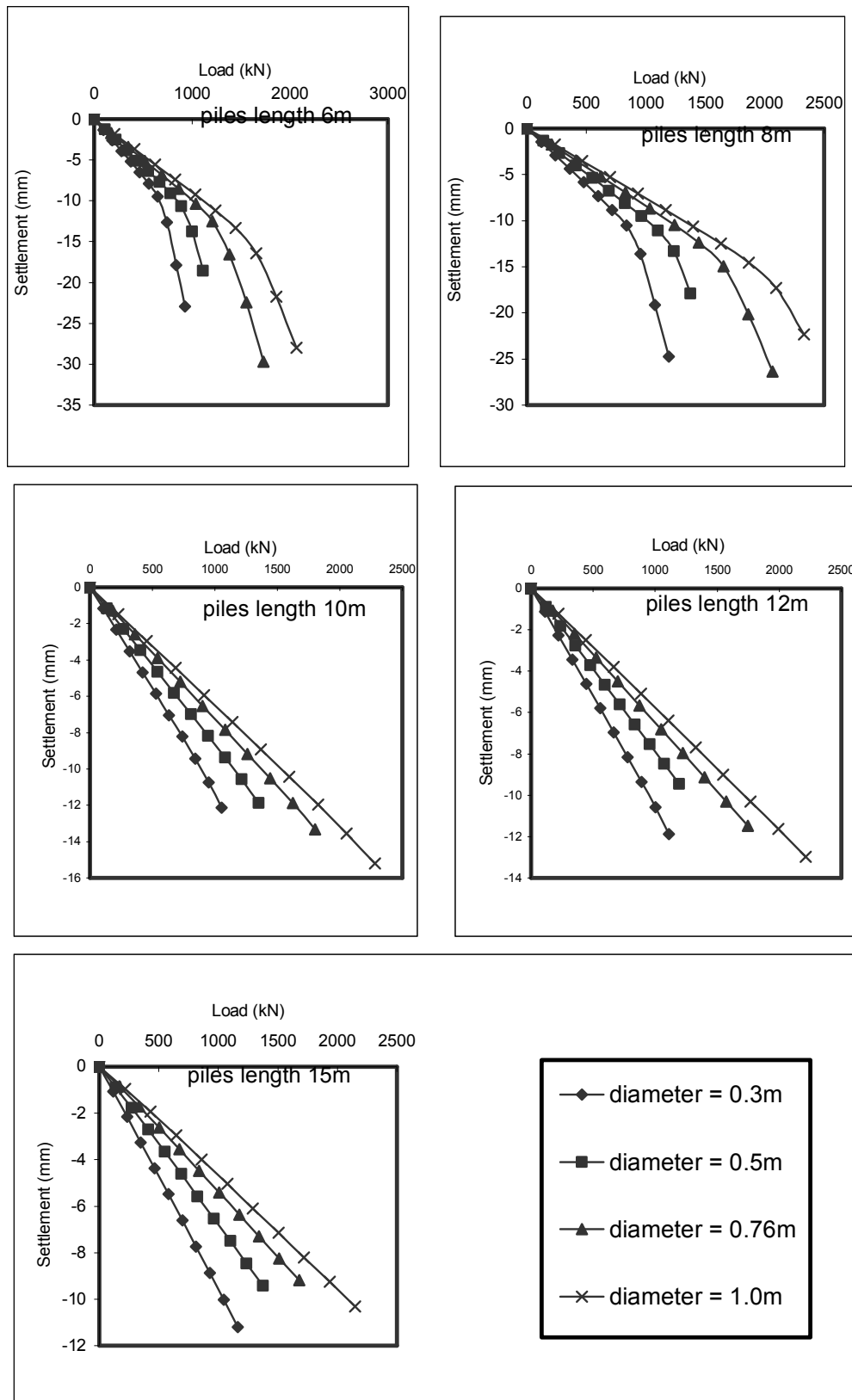
Figure B.16. Settlement-Load Relationship for French Bank Building Site ( Piles Lengths 6, 8, 10, 12 and 15m ).
