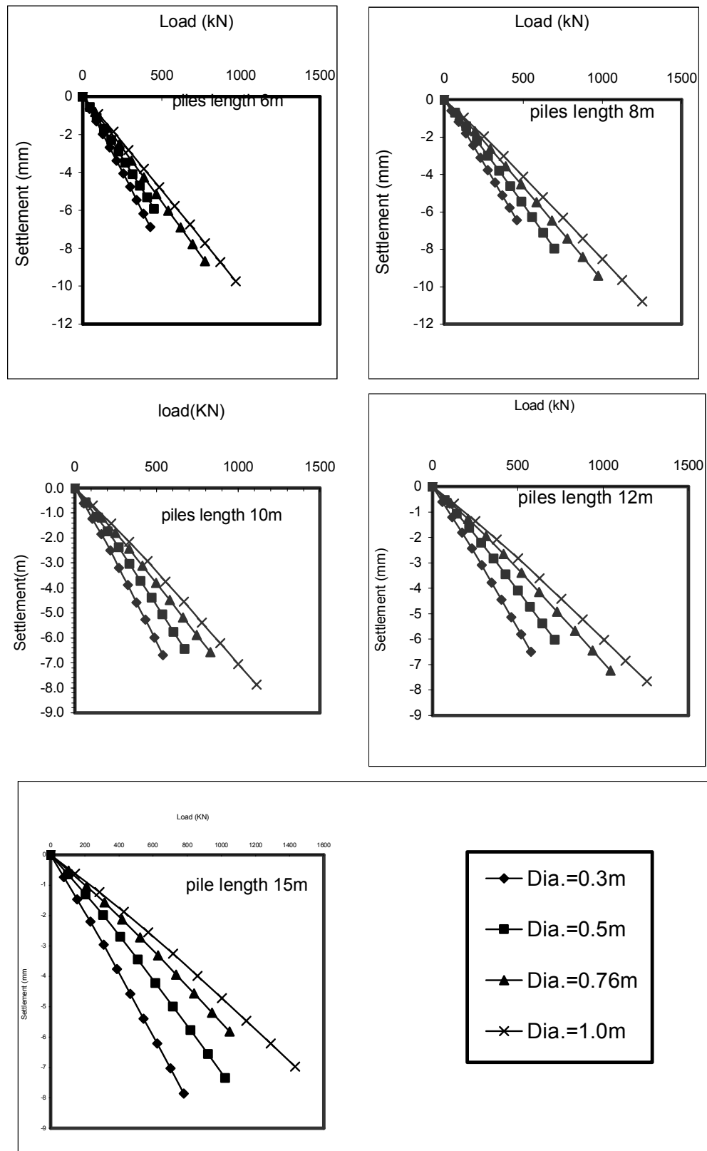
Figure B.6. Settlement-Load Relationship for Mak-Nimir Bridge Site ( Piles Lengths 6, 8, 10, 12 and 15m ).
