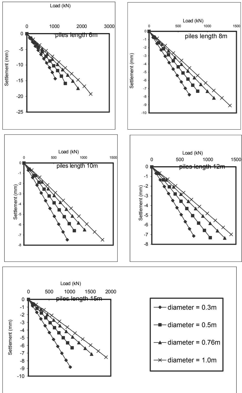
Figure B.14. Settlement-Load Relationship for Chinese Embassy Building Site ( Piles Lengths 6, 8, 10, 12 and 15m ).
