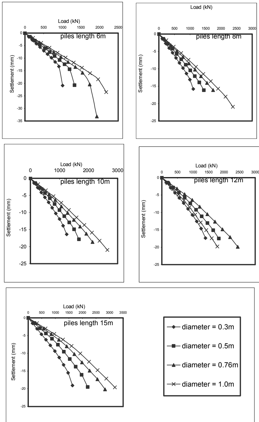
Figure B.13. Settlement-Load Relationship for Tuti Island Bridge Site ( Piles Lengths 6, 8, 10, 12 and 15m ).
