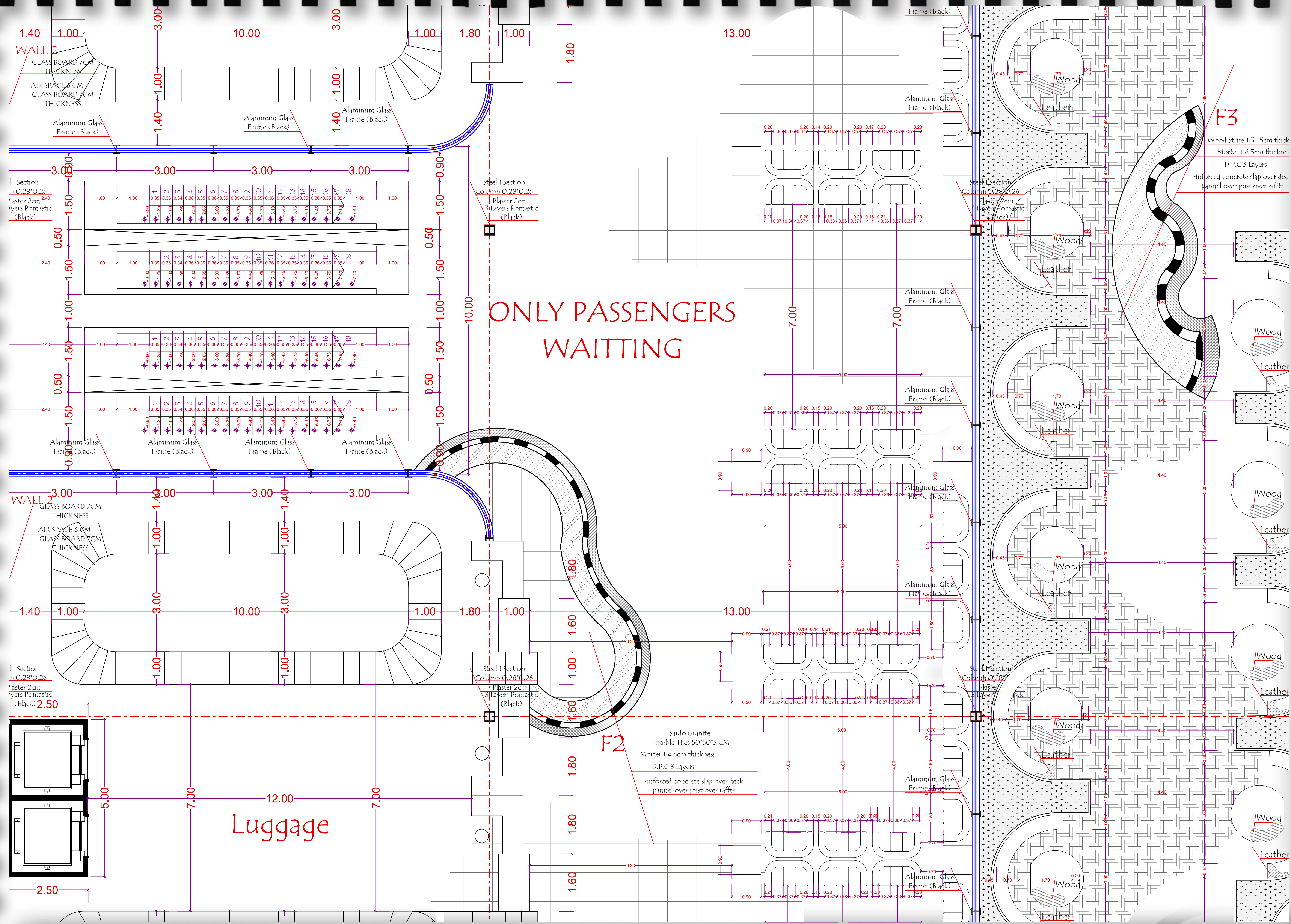
Passengers Waitting Part PLAN Scale 1:50
