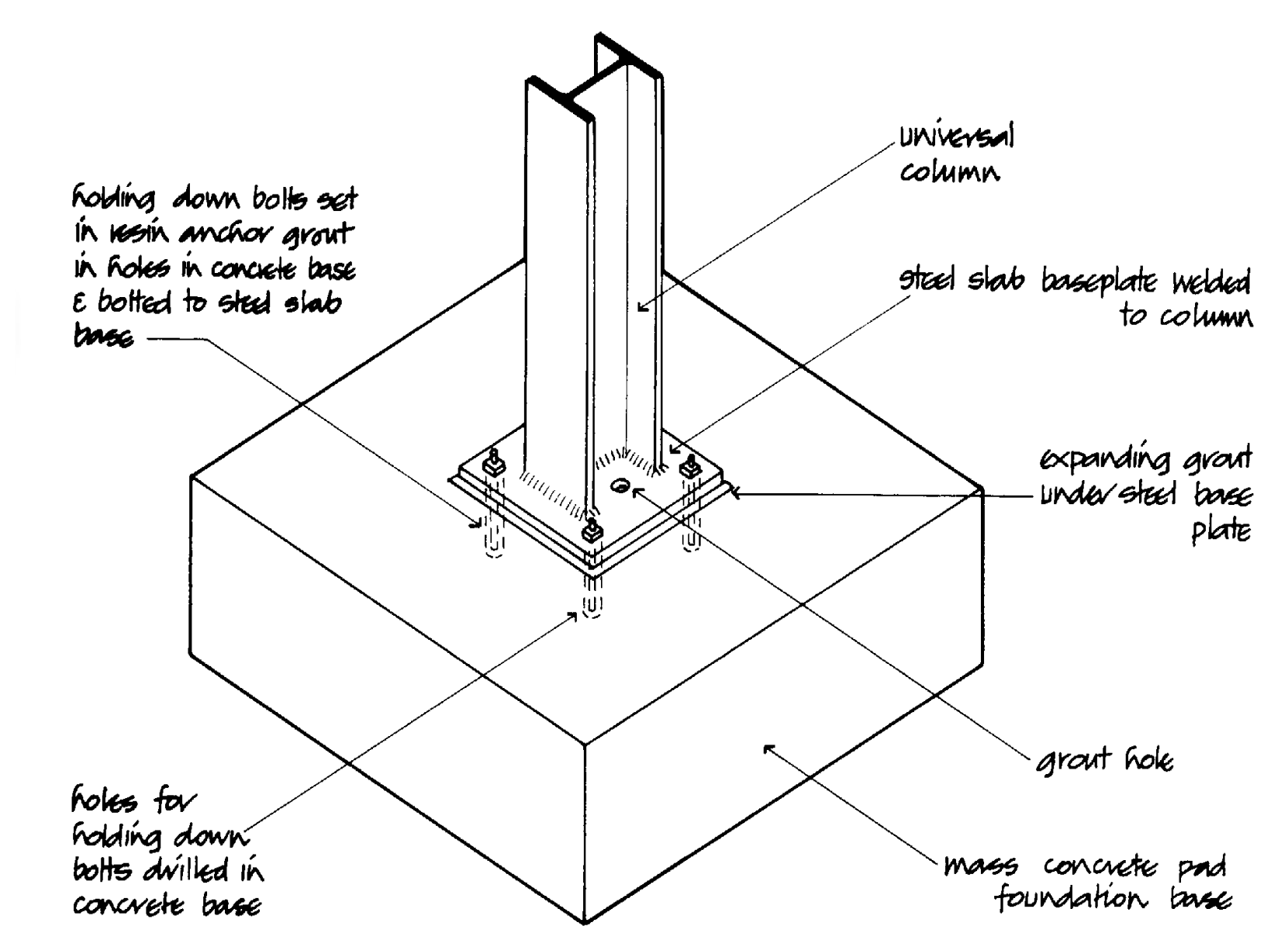
Steel slab base on concrete pad foundation.
