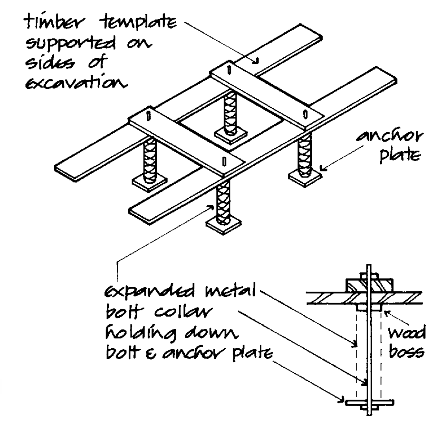
Expanded metal foundation bolt boxes
