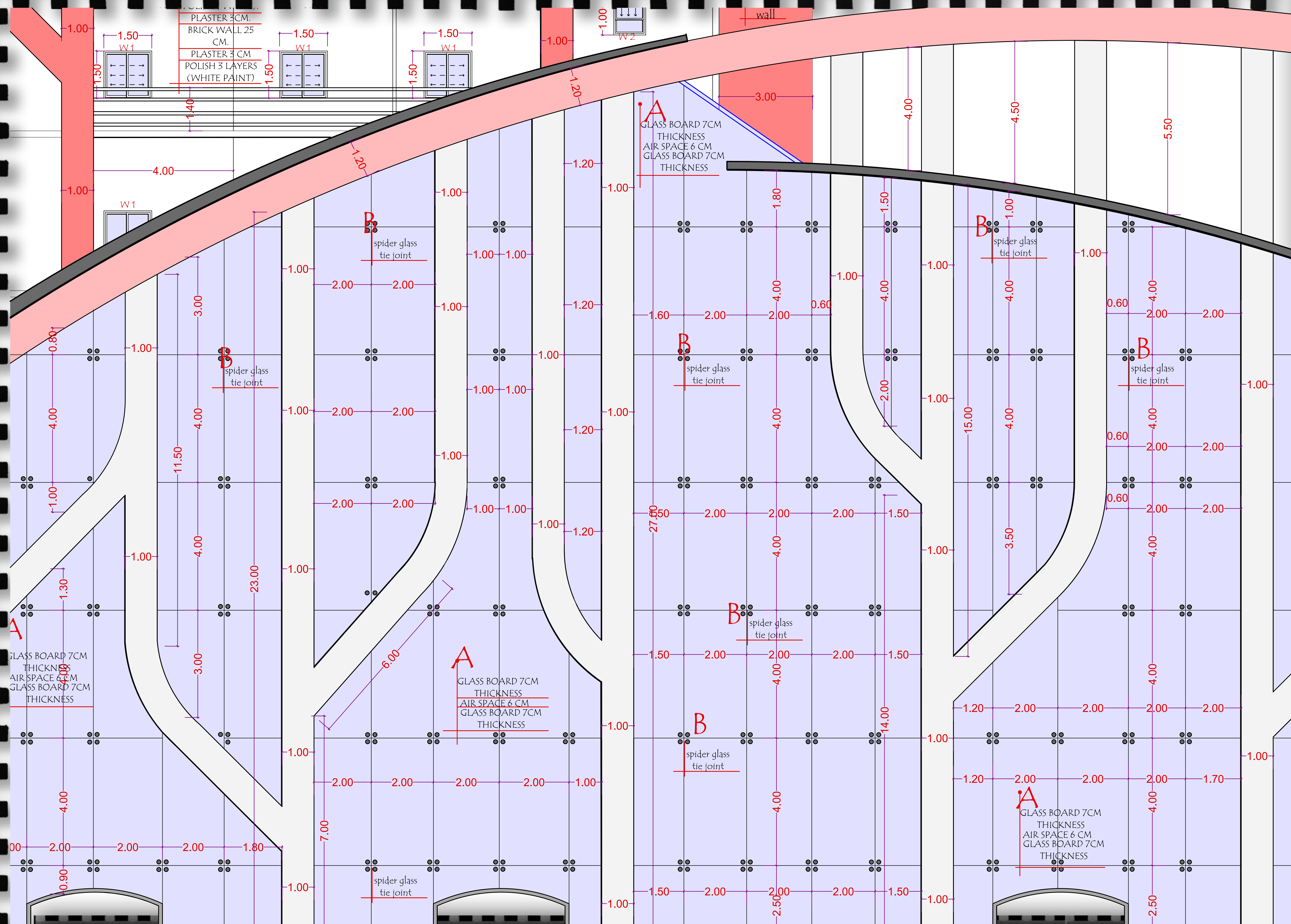
PART ELEVATION Scale 1:50
