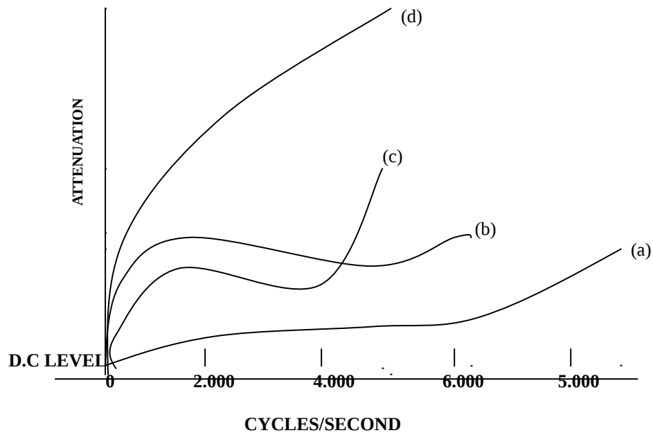
Figure.2. Cable attenuation frequency characteristics
