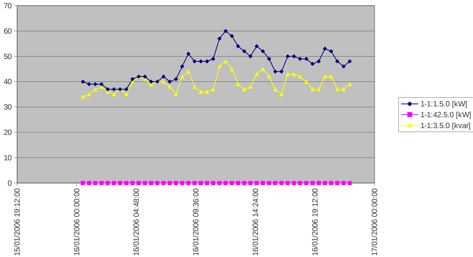
Load Profile
