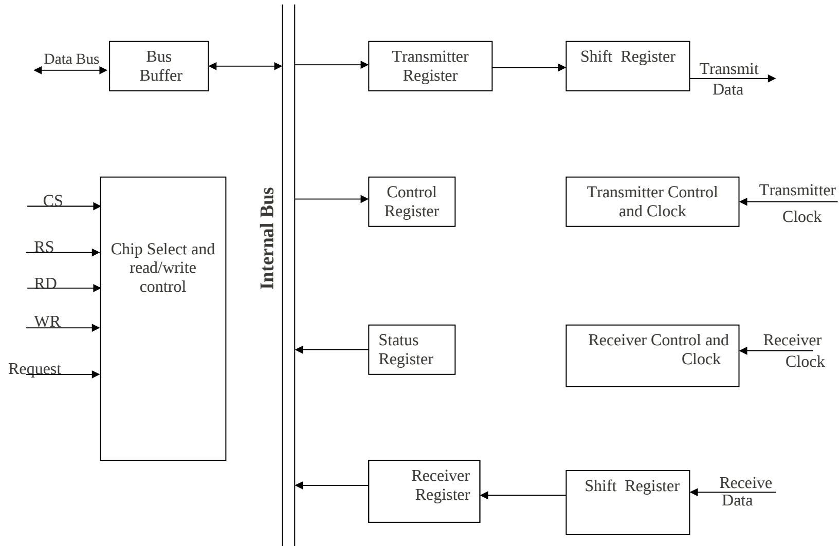
Figure (3.3) Block diagram of serial communication interface
