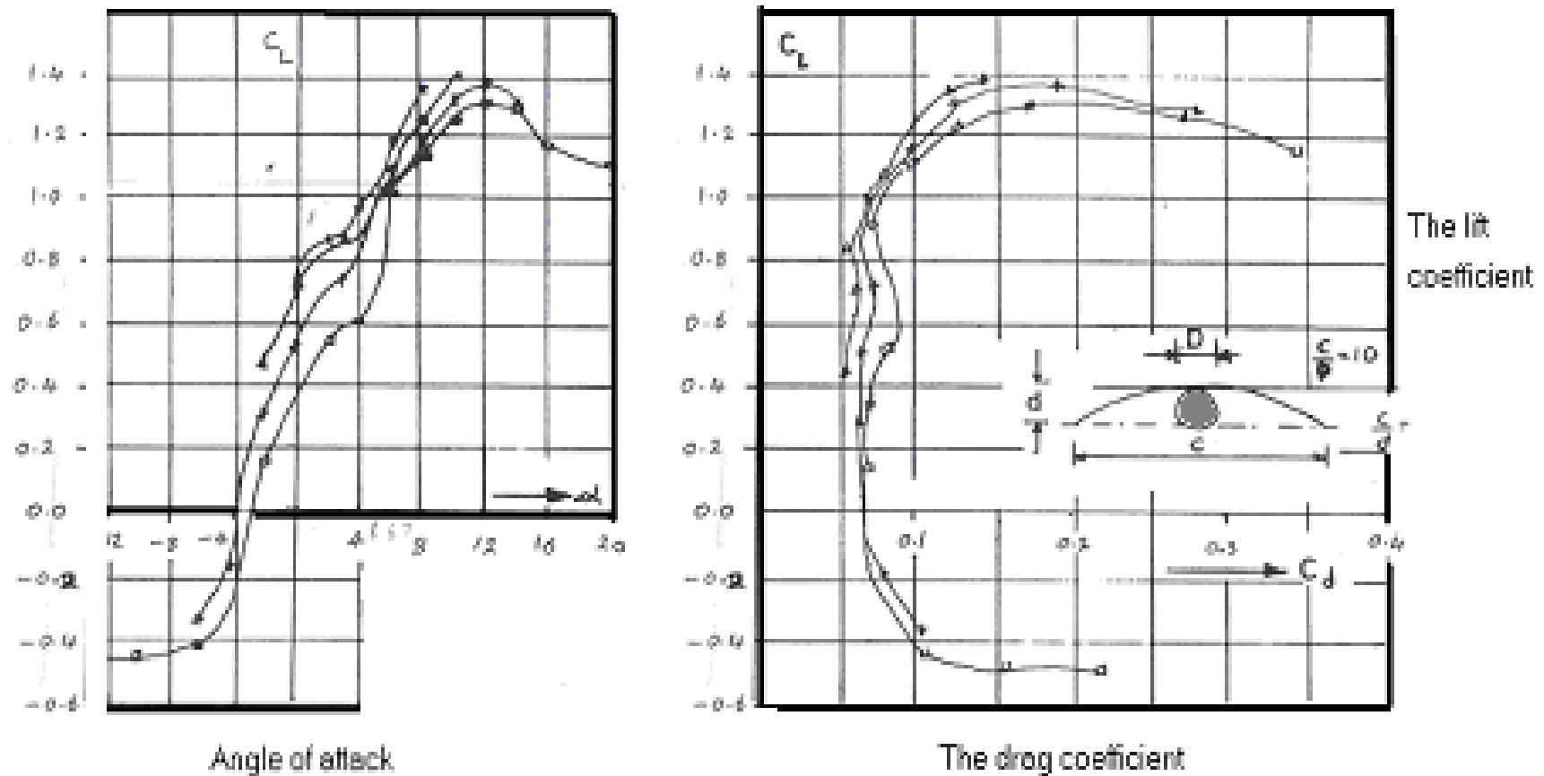
[Figure (4.1) graph of lift coefficient versus the angle of attack and drag coefficient [1
