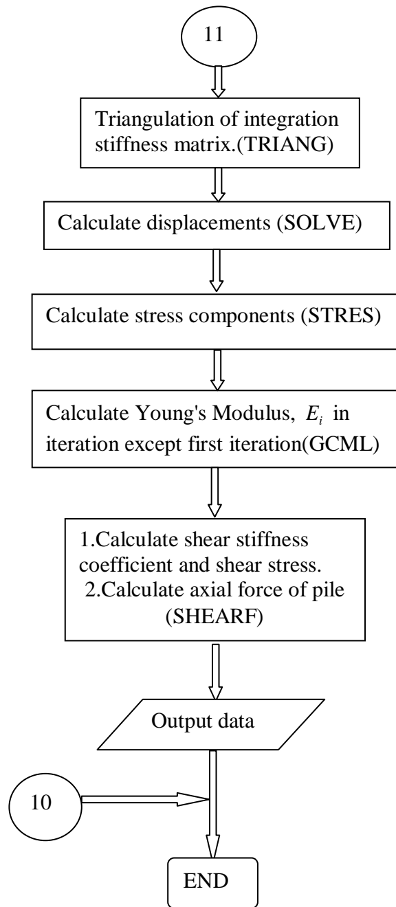
Fig(A-1) Program flow chart(continued2)
