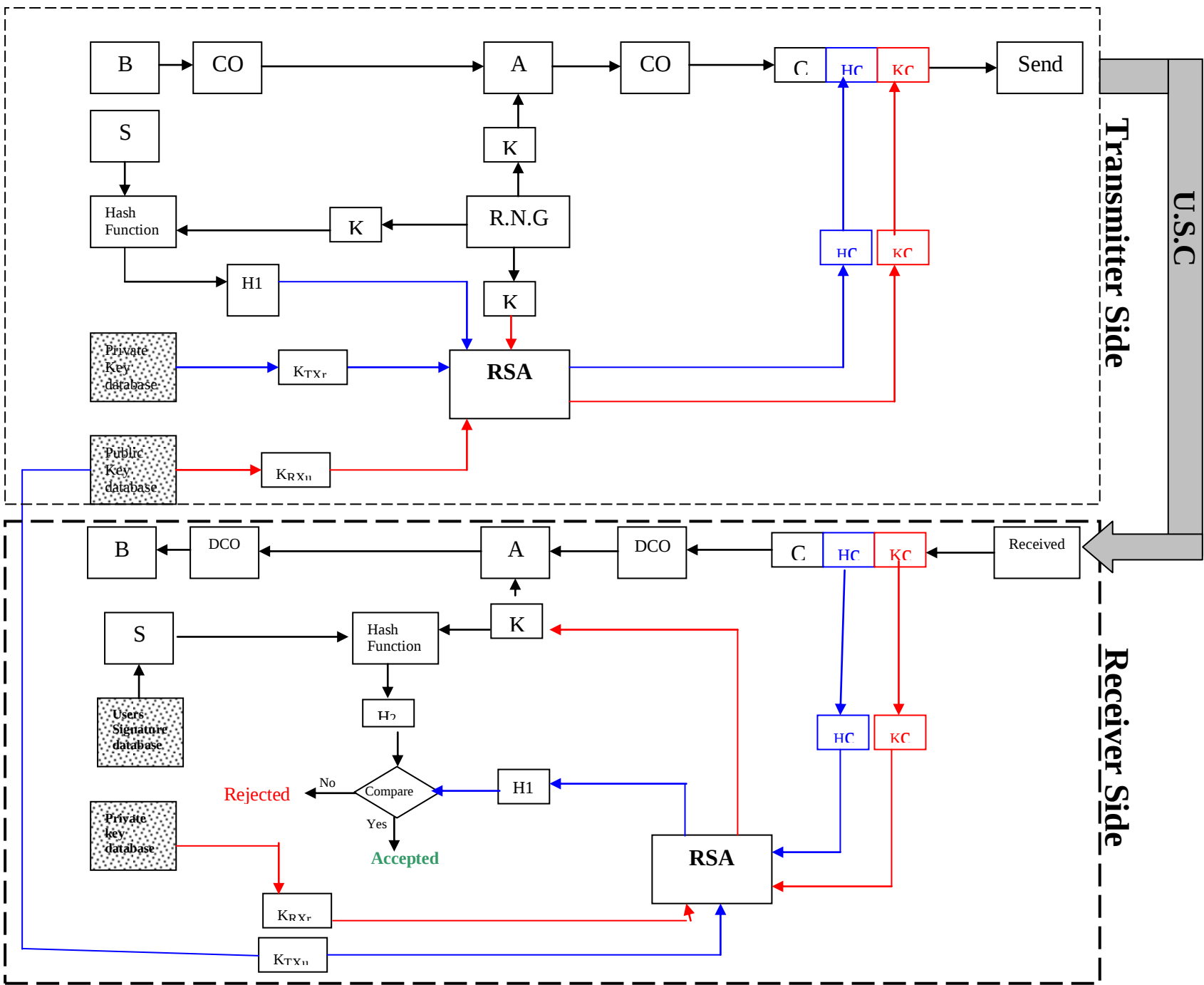
Fig (4.0) :Scheme of The Hole Security System
