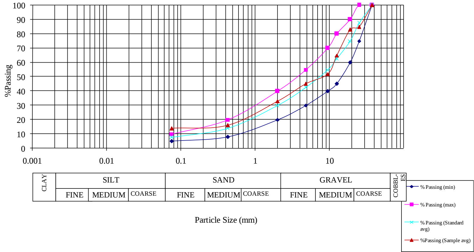
Figure 3.4 - Sample (1) Grain Size Sieve Analysis Treatment Trial (3): 12% Crushed Stone & 10% Sand
