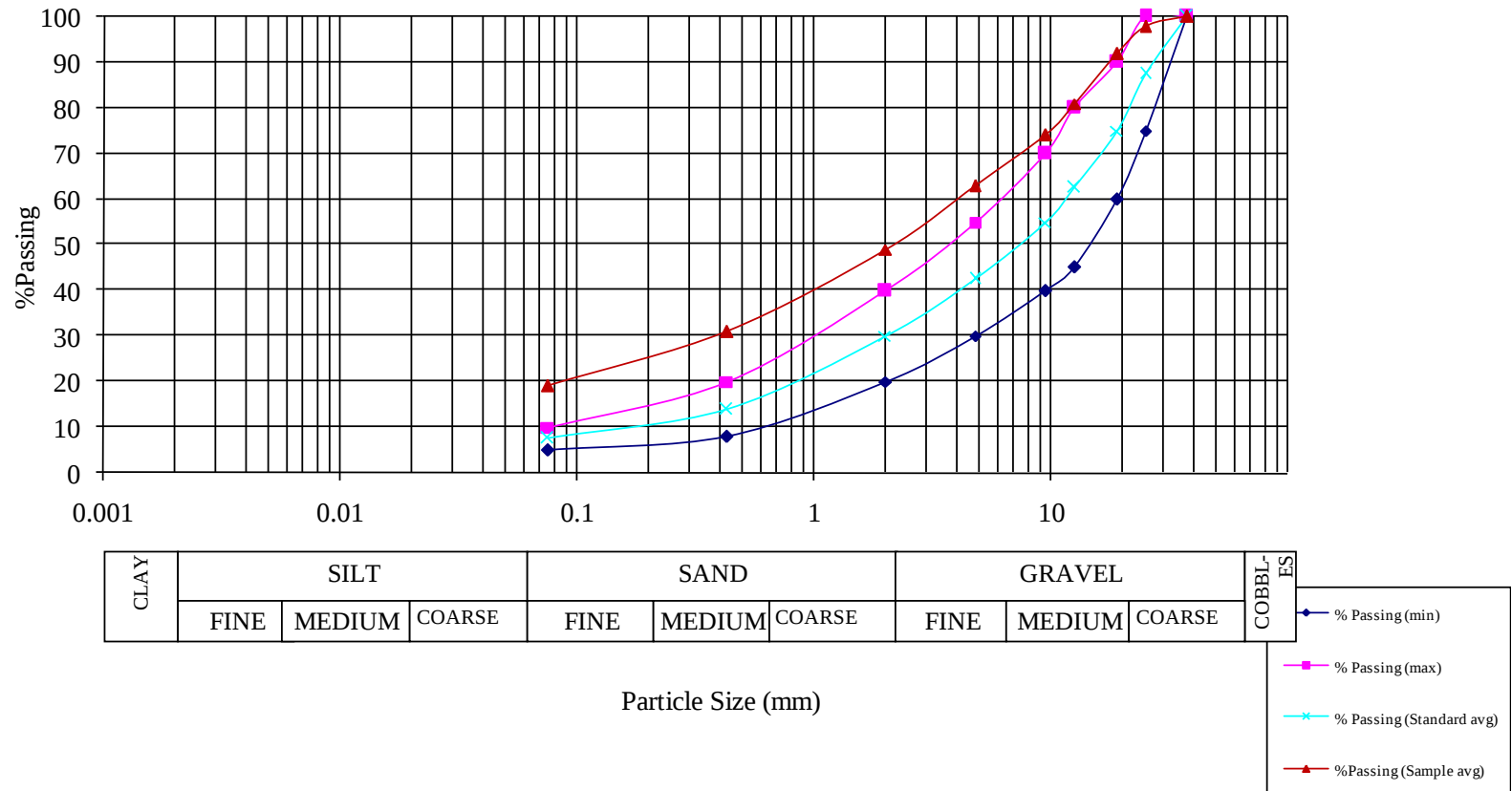
Figure 3.8 - Sample (3) Grain Size Sieve Analysis
