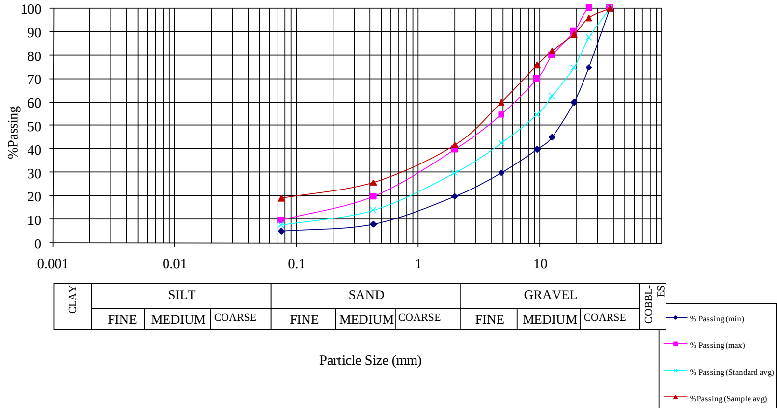
Figure 3.5 - Sample (2) Grain Size Sieve Analysis
