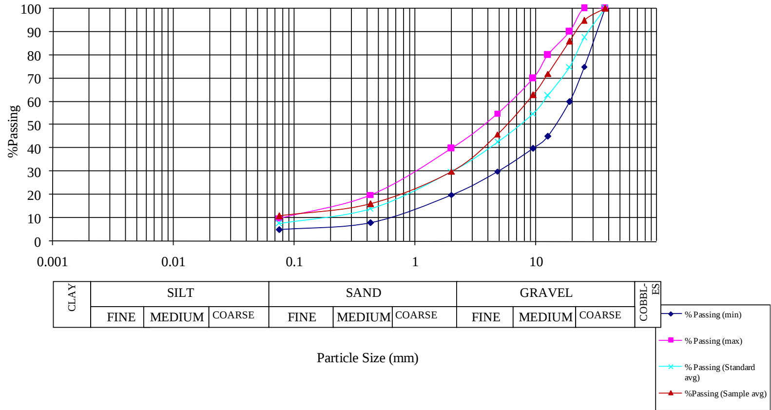
Figure 3.9 - Sample (3) Grain Size Sieve Analysis Treatment Trial (1):17% Gravel & 10% Sand
