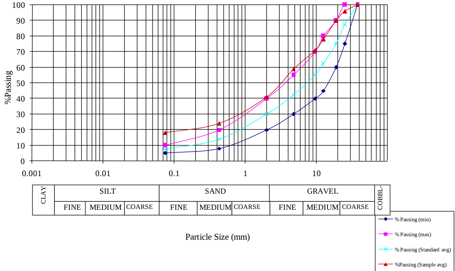
Figure 3.1 - Sample (1) Grain Size Sieve Analysis
