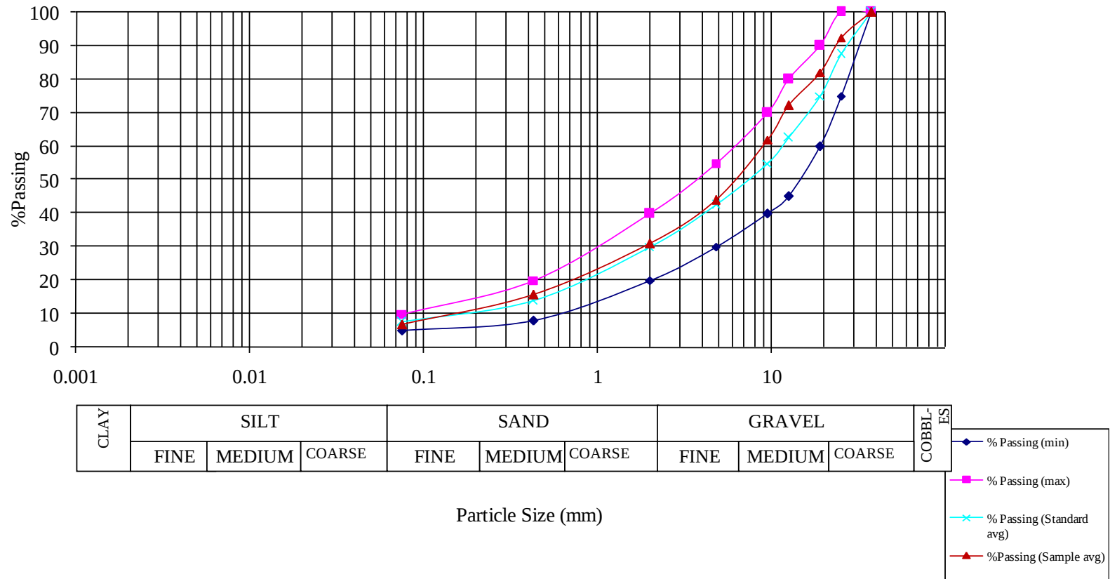
Figure 3.7 - Sample (2) Grain Size Sieve Analysis Treatment Trial (2): 12% Crushed Stone & 10% Sand
