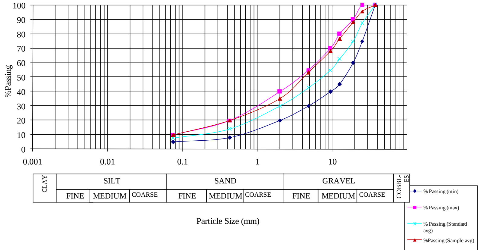
Figure 3.3 - Sample (1) Grain Size Sieve Analysis Treatment Trial (2): 15% Gravel & 10% Sand
