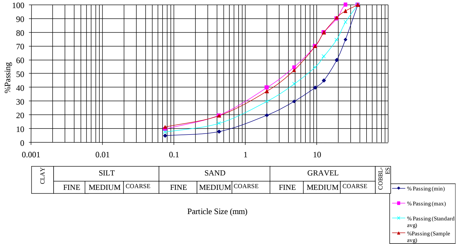
Figure 3.2 - Sample (1) Grain Size Sieve Analysis Treatment Trial (1): 15% Gravel & 10% Sand
