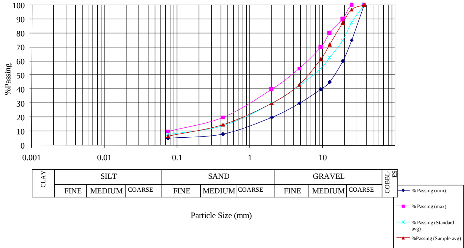
Figure 3.6 - Sample (2) Grain Size Sieve Analysis Treatment Trial (1):17% Gravel & 10% Sand
