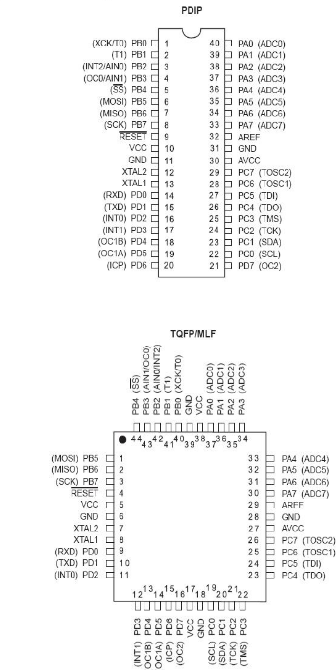
Figure 1. Pinouts ATmega32
