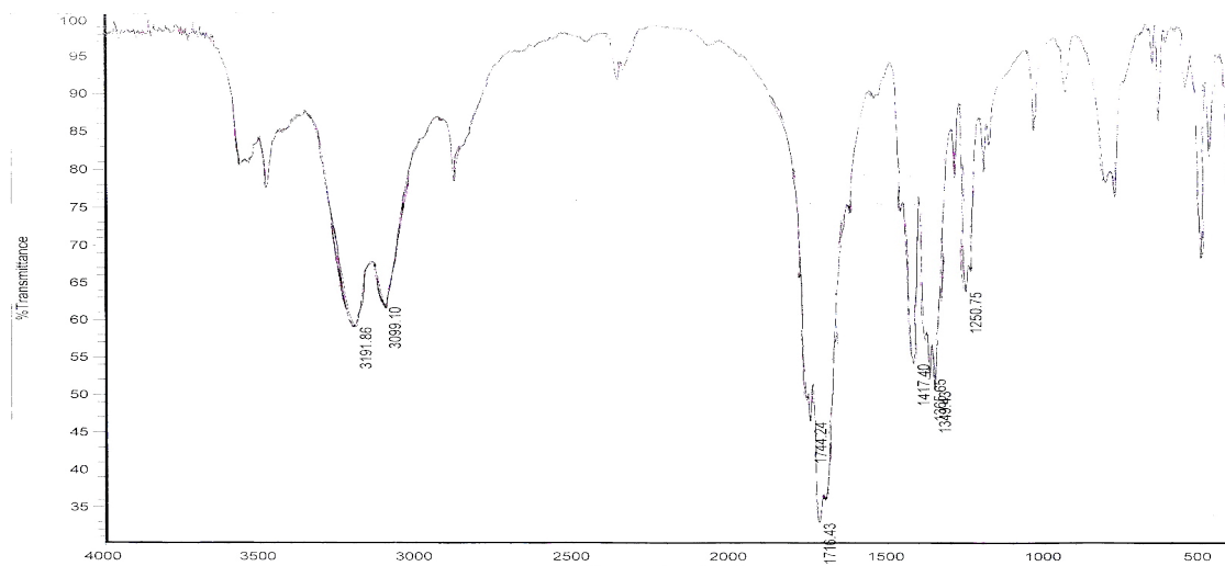
Fig 2.11.C.IR spectra of pyrimidine-2,4,6- trione (Vf)(1µg/100mg)
