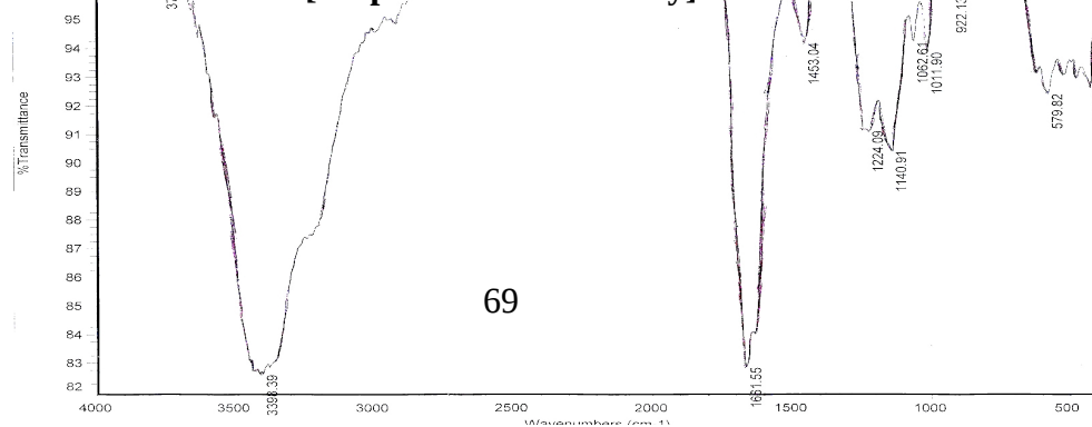
Fig.2.13.IR spectra of 5-phenyl pyrimidine-2,4,6- trione (Vc) [Prepared mechanically]
