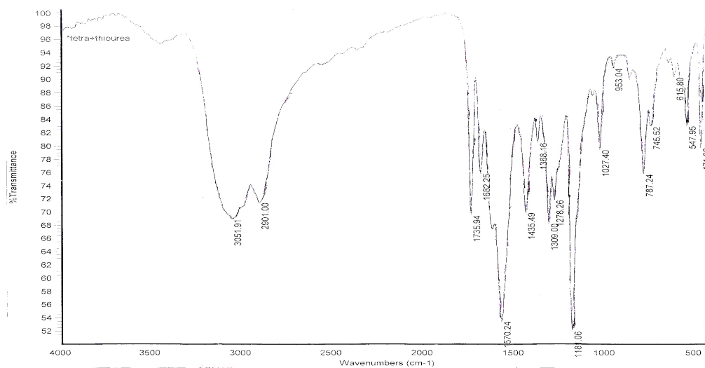
Fig.2.18.IR spectra of 5- diethyl malonylpyrimidine-2- thio-4,6- dione (VIId)
