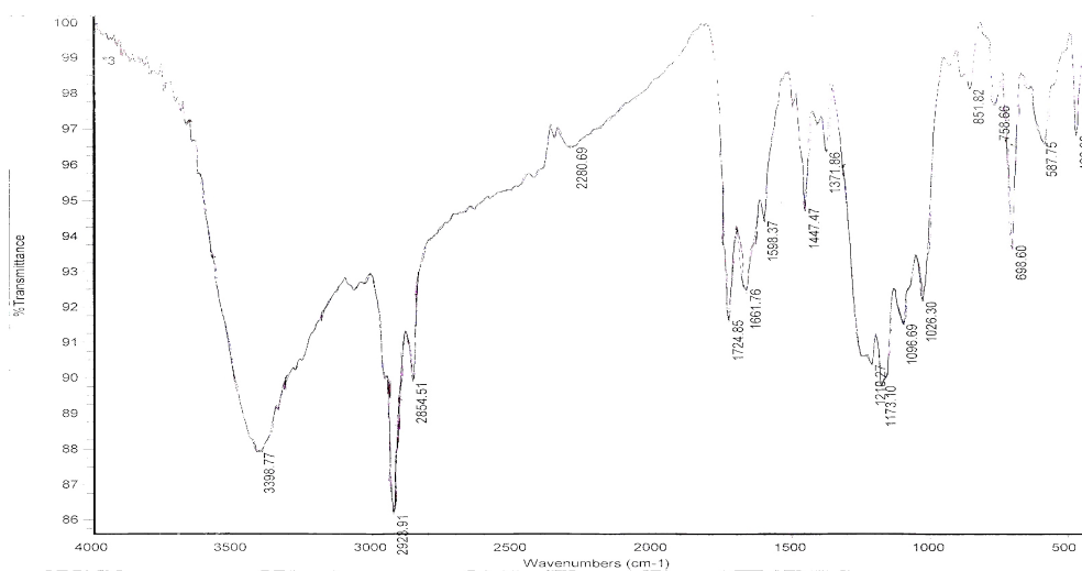
Fig.2.17.IR spectra of 5- benzoyl pyrimidine-2- thio-4,6- dione (VIg)
