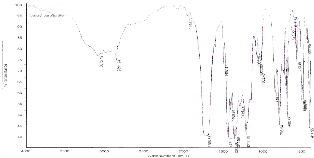
Fig.2.14.IR spectra of 5-benzyl pyrimidine-2,4,6- trione (Vb)
