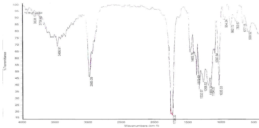
Fig.2.5. IR spectra of diethyl ethyl malonate (Ia)
