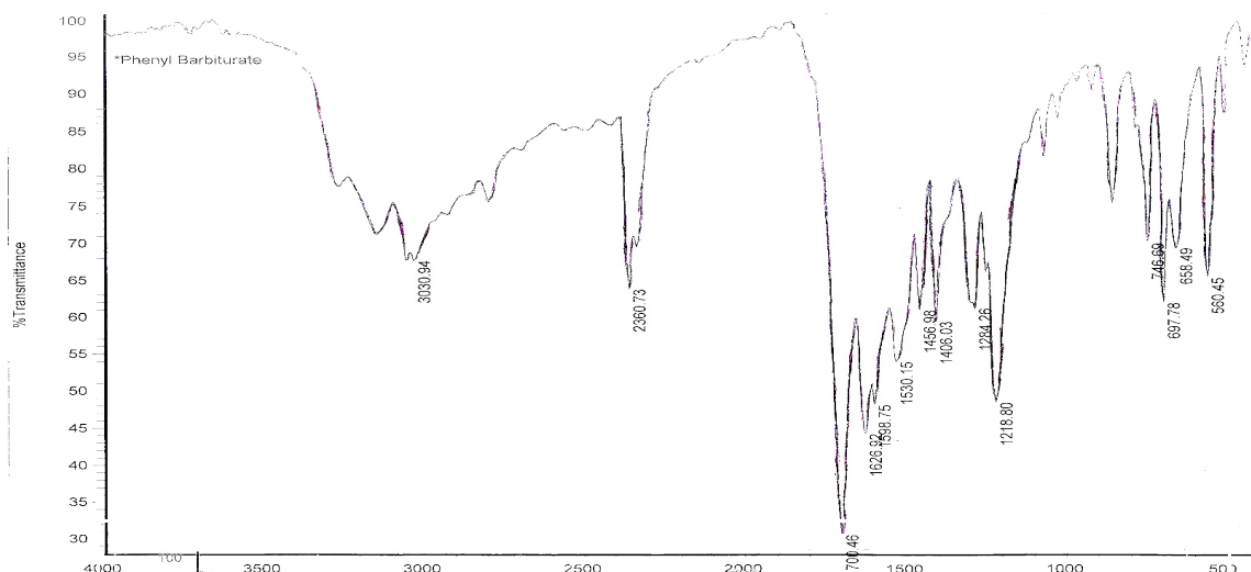
Fig.2.13.IR spectra of 5-phenyl pyrimidine-2,4,6- trione (Vc) [Prepared mechanically]
