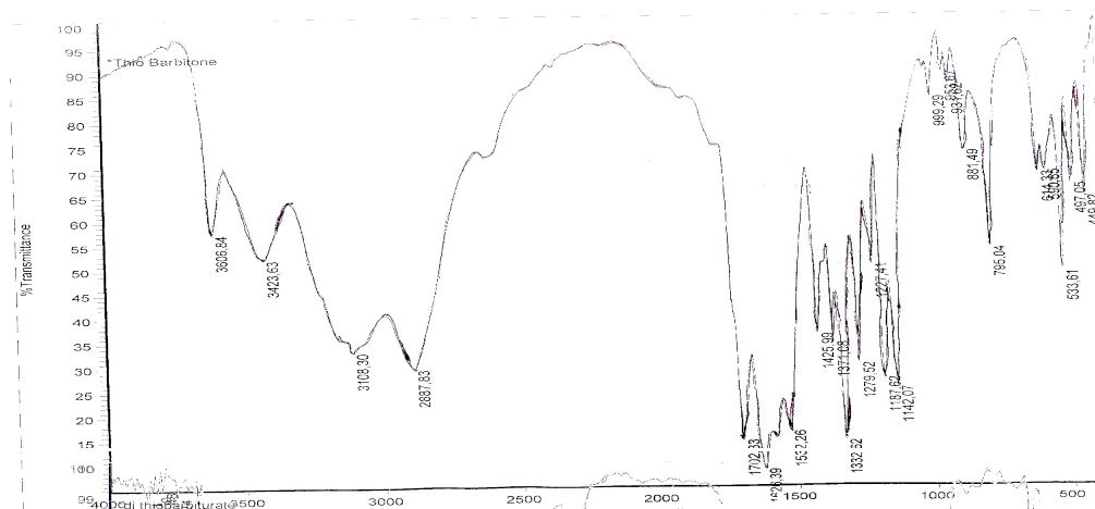
Fig.2.15 IR spectra of pyrimidine-2- thio-4,6- dione (VIh)
