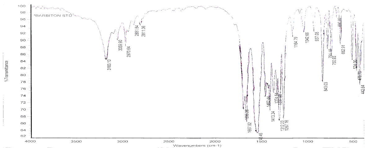
Fig.2.10.IR spectra of 5- ethyl -5- phenyl pyrimidine-2,4,6- trione (Standard sample)
