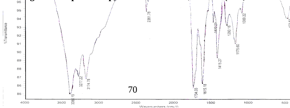
Fig.2.15 IR spectra of pyrimidine-2- thio-4,6- dione (VIh)
