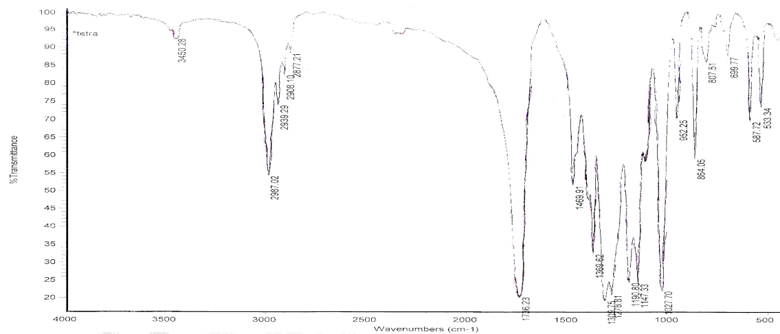
Fig.2.8.IR spectra of ethane tetra ethyl carboxylic acid (III)
