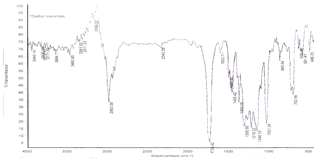
Fig.2.7.a.IR spectra of diethyl phenyl malonate (II)
