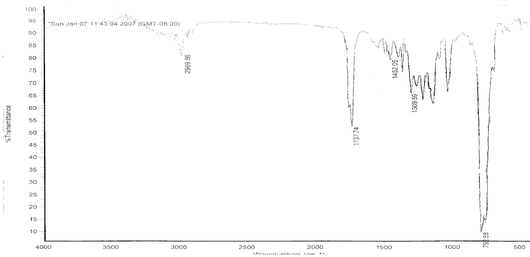
Fig.2.7.b.IR spectra of diethyl phenyl malonate (II) (in CCl 4 )
