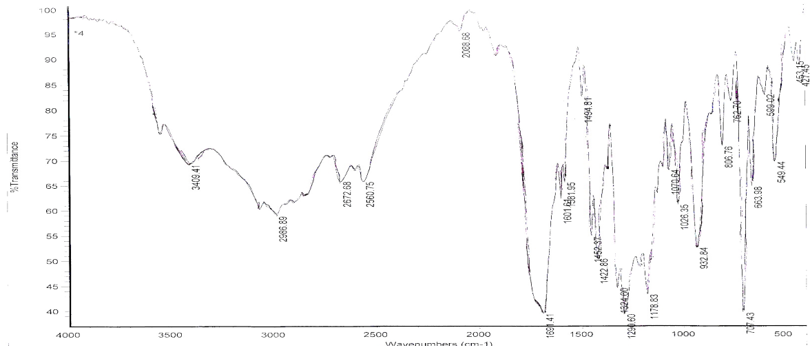
Fig.2.9.IR spectra of diethyl benzoyl malonate (IV)
