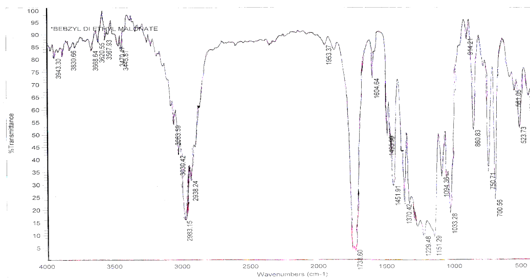
Fig.2.6. IR spectra of diethyl benzyl malonate (Ib)
