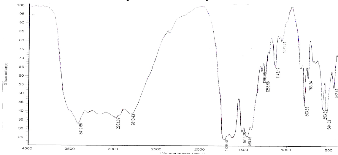
Fig.2.12.IR spectra of 5-ethyl pyrimidine-2,4,6- trione (Va) [Prepared mechanically]
