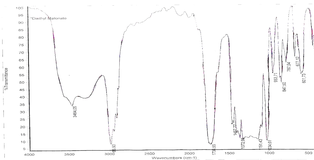
Fig.2.4. IR spectra of diethyl malonate
