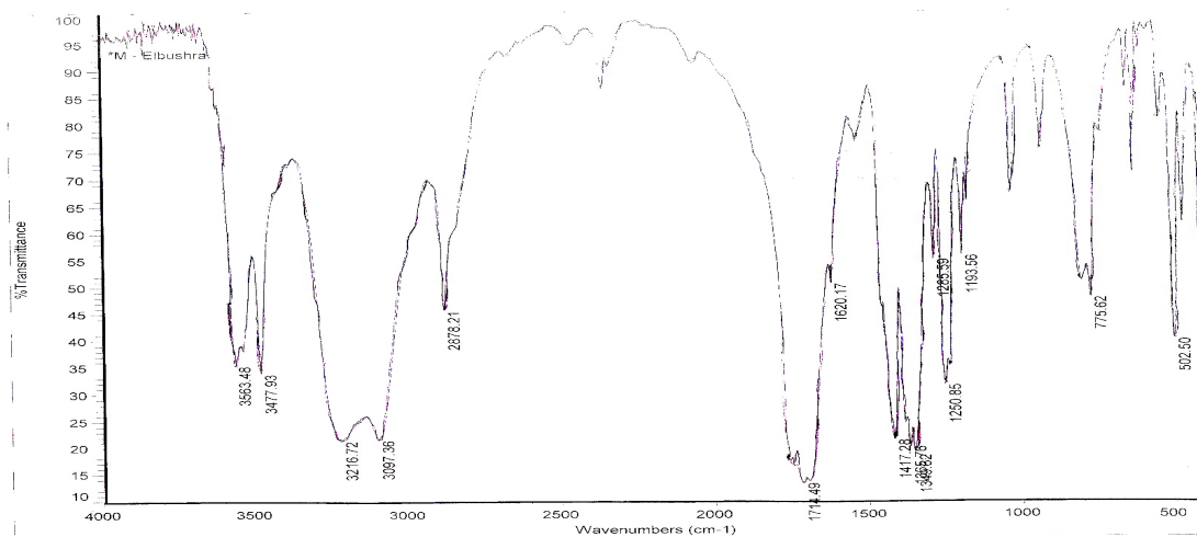
Fig.2.11.b.IR spectra of pyrimidine-2,4,6- trione (Vf)(10µg/100mg)
