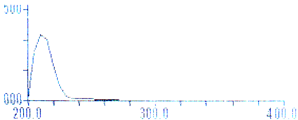
Fig.2.21.UV spectra of 5- benzyl pyrimidine-2,4,6-trione (Vb) (in ether)
