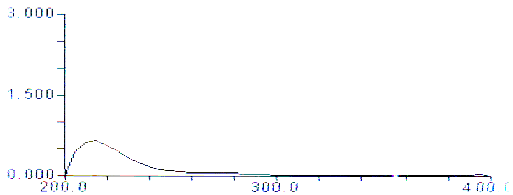
Fig.2.19.UV spectra of diethyl phenyl malonate (II)
