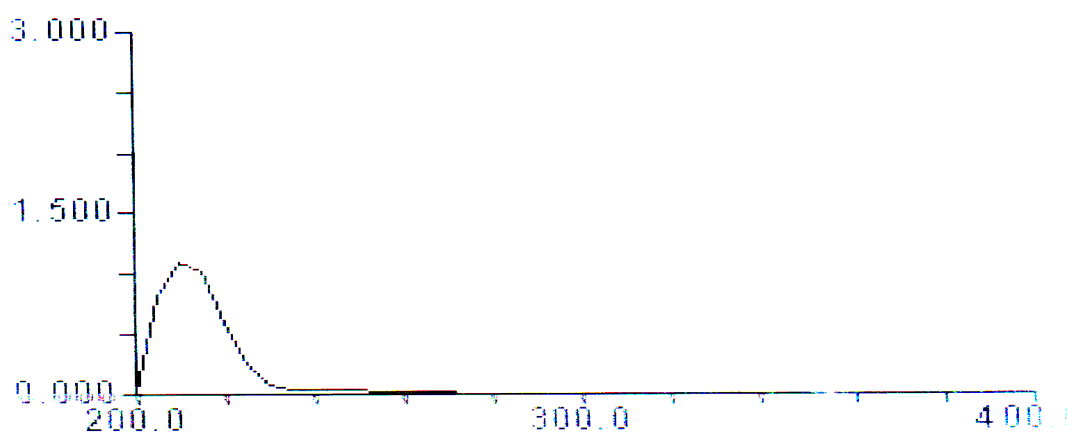
Fig.2.20.UV spectra of diethyl benzyl malonate (Ib)
