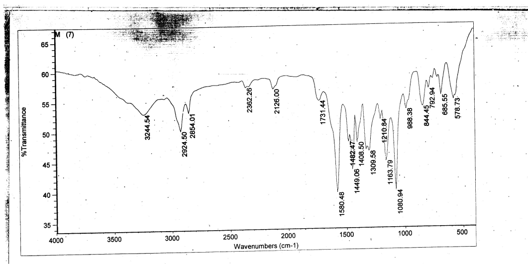
Appendix 3- 11: IR spectrum of 5-barbitric acid azo-4-aminosalicylic acid XIII
