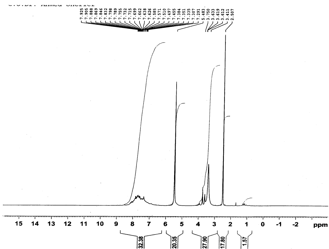
Appendix 3-23: NMR spectrum of 5-barbitric acid azo-4-sulphadoxine VII
