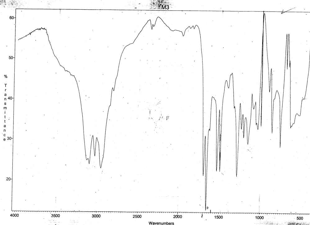
Appendix 3-9: IR spectrum of 1-(2,4-dinitrobenzene pyrazol-3,5-dione) azo-aminosalicylic acid XI
