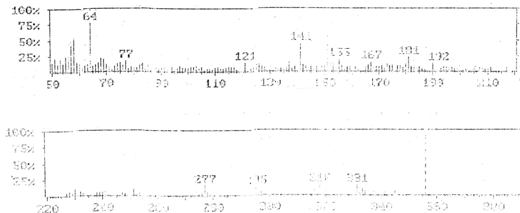
Appendix 29: MS spectrum of 2-(4-carboxypyridine pyrazol-3,5-dione) azo-4-sulphadoxine VI .
