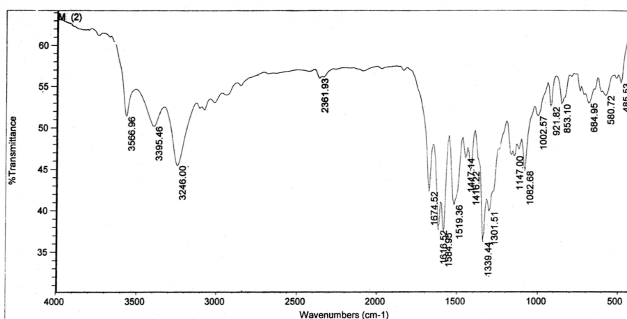
Appendix 3-3: IR spectrum of 2-diethylmalonate azo-4-amino salicylic acid X
