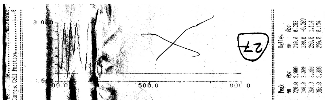
Appendix 3- 27: UV spectrum of 5-1-thiobarbitric acid azo-4-aminosalicylic acid XIV
