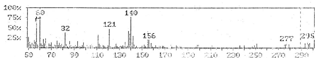
Appendix 32: MS spectrum of 5-barbitric acid azo -4-aminobenzoic acid XVIII
