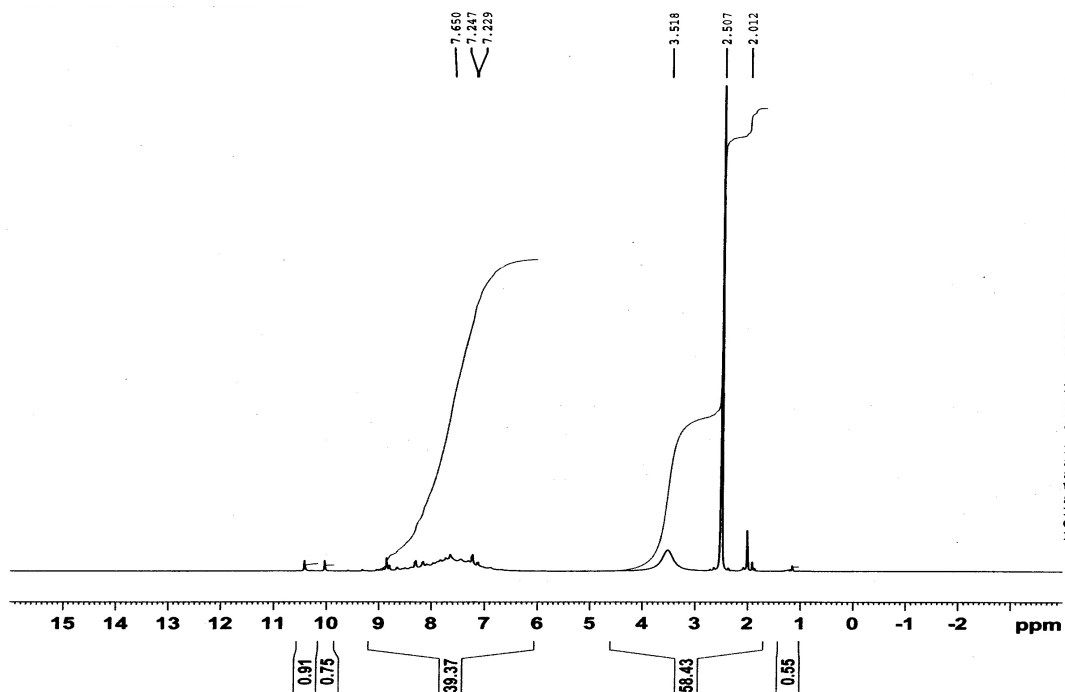
Appendix 3-15: NMR spectrum of 2-diethylmalonateazo-4-amino salicylic acid X
