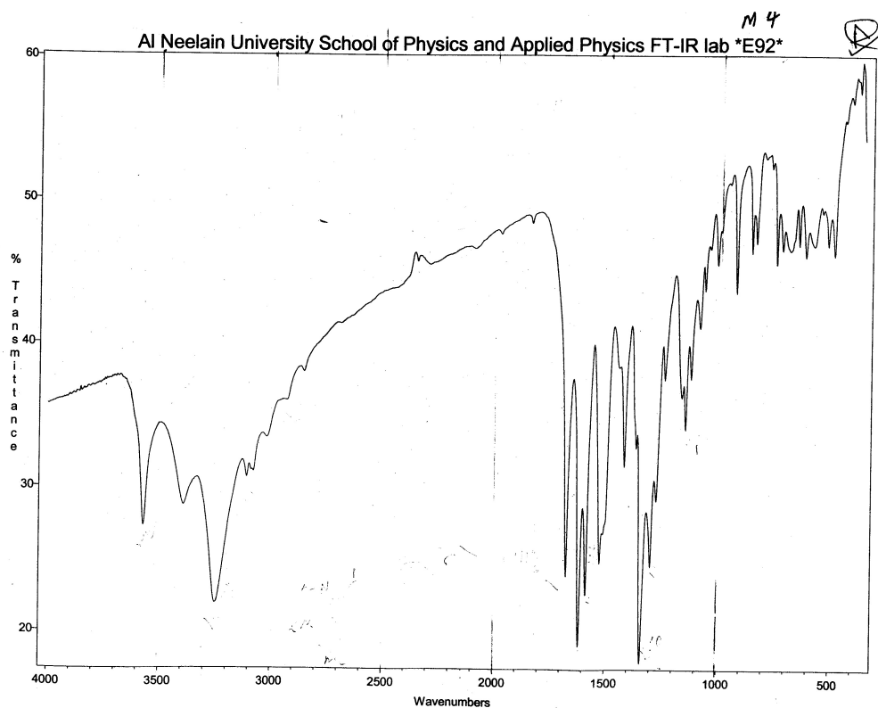
Appendix 3- 7: IR spectrum of 1-(2,4-dinitrobenzene pyrazol-3,5-dione) azo-4-sulphadoxine IV
