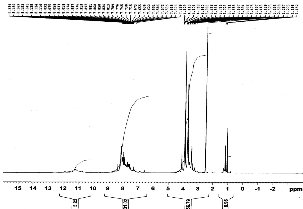
Appendix 3-14: NMR spectrum of 2-diethylmalonateazo-sulphadoxine V
