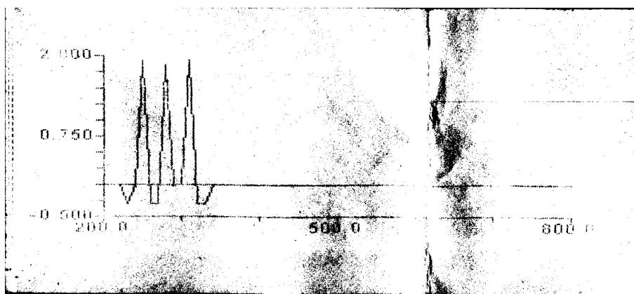
Appendix 3- 28: UV spectrum of 5-1-thiobarbitric acid azo-4-sulphanilamide XXV
