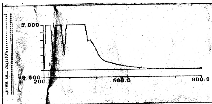
Appendix 3- 25: UV spectrum of 2-diethylmalonateazo-sulphadoxine V
