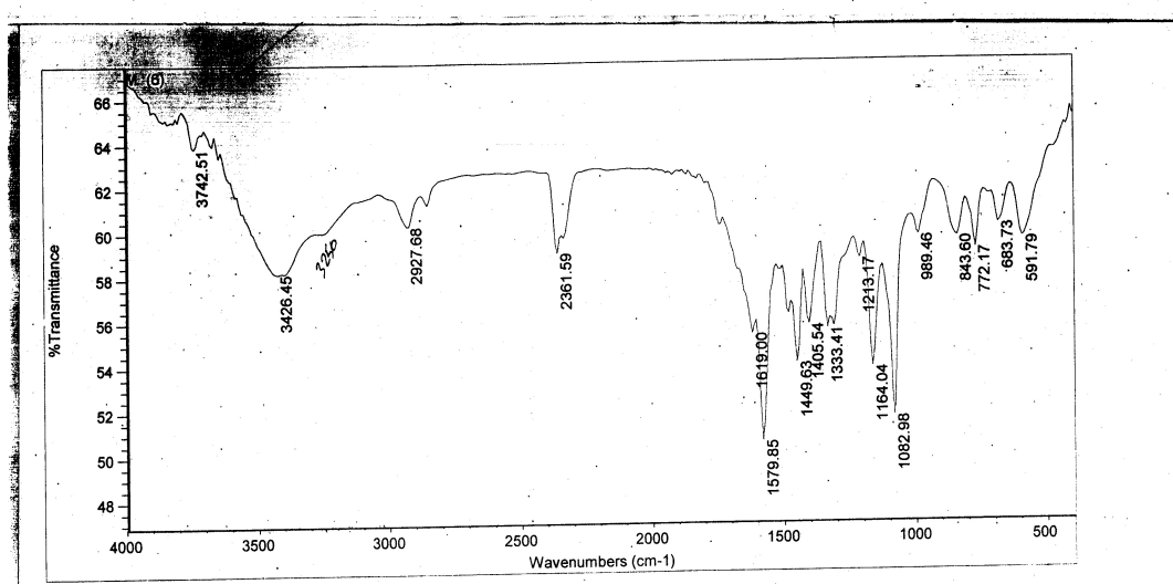
Appendix 3-5: IR spectrum of 2-(4-carboxypyridine pyrazol-3,5-dione) azo-sulphadoxine VI
