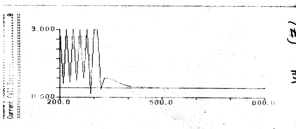
Appendix 3- 26: UV spectrum of 5-barbitric acid azo-4-sulphadoxine VII
