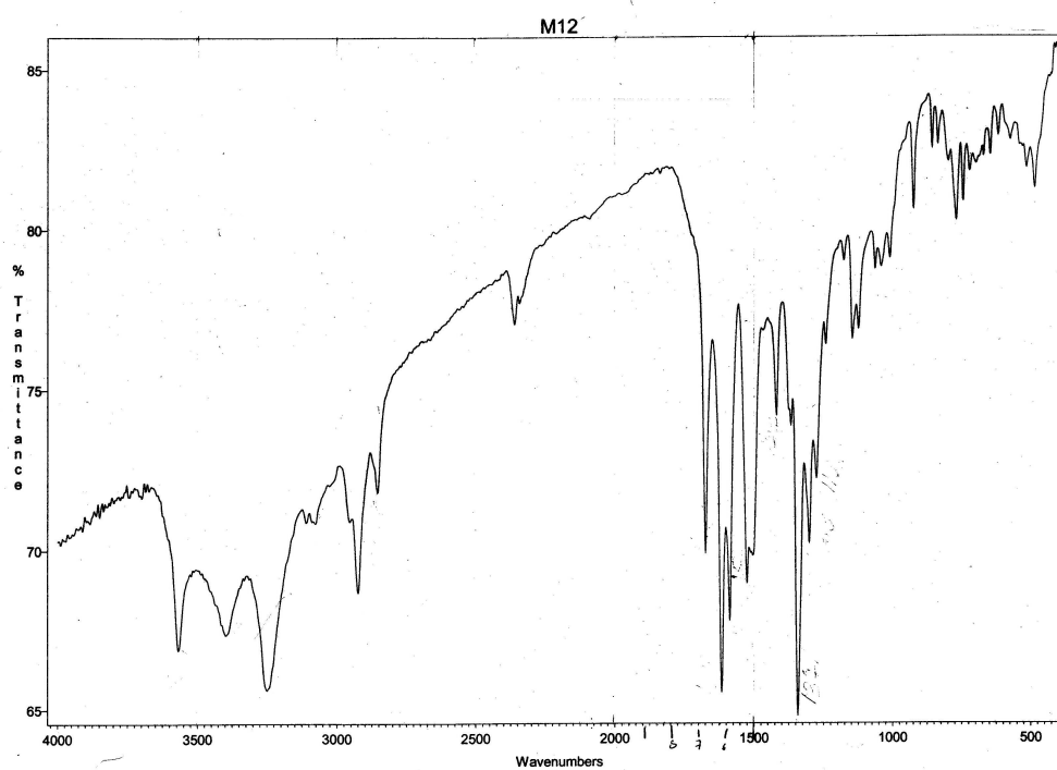
Appendix 3-5: IR spectrum of 2-(4-carboxypyridine pyrazol-3,5-dione) azo-sulphadoxine VI
