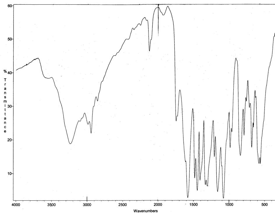
Appendix 3-2: IR spectrum of 2-diethylmalonateazo-sulphadoxine V
