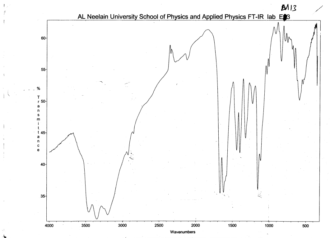
Appendix 3- 11: IR spectrum of 5-barbitric acid azo-4-aminosalicylic acid XIII
