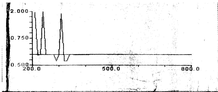
Appendix 3-24: UV spectrum of 2-diethylmalonateazo-4-sulphanilamide I
