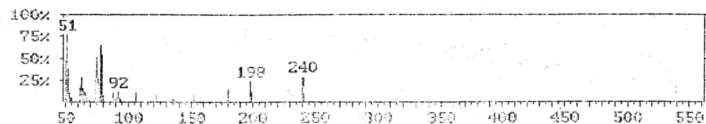
Appendix 31: MS spectrum of 1-(2,4-dinitrobenzenepyrazol-3,5-dione) azo-4-sulphaadoxine VIII
