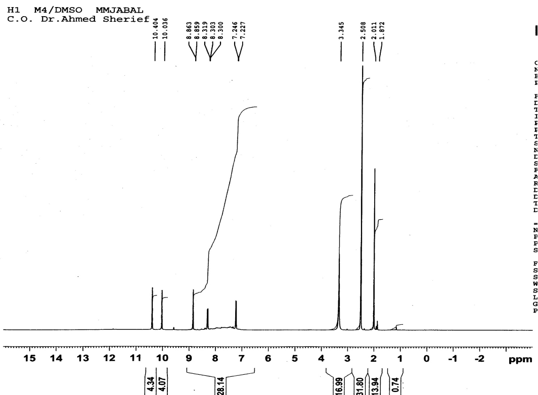
Appendix 3-21: NMR spectrum of 1-(2,4-dinitrobenzene pyrazol-3,5-dione) azo-4-sulphanilamide IV
