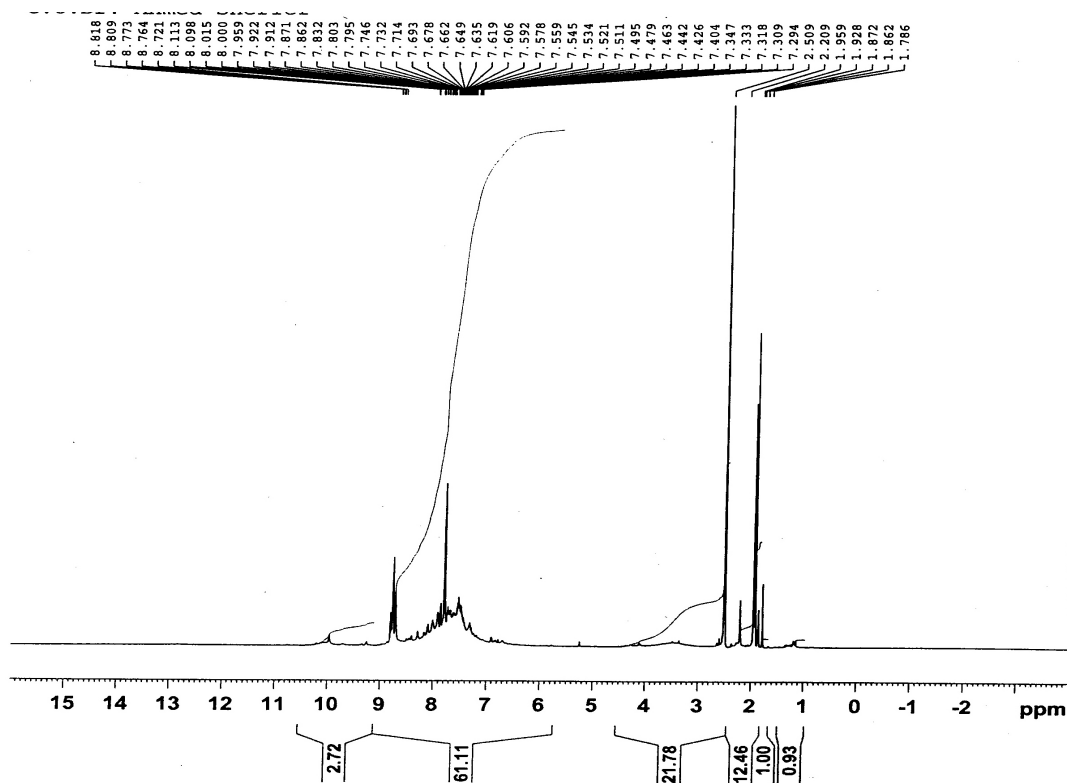
Appendix 3-19: NMR spectrum of 1-(4-carboxypyridine pyrazol-3,5-dione) azo-aminosalicylic acid XI
