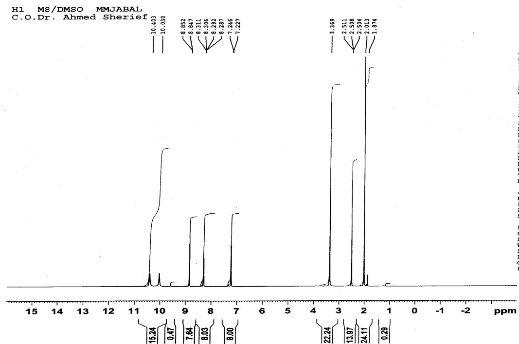
Appendix 3-19: NMR spectrum of 1-(4-carboxypyridine pyrazol-3,5-dione) azo-aminosalicylic acid XI
