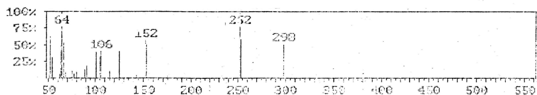
Appendix 30: MS spectrum of 2-diethylmalonate azo-1-naphthylamine XX .
