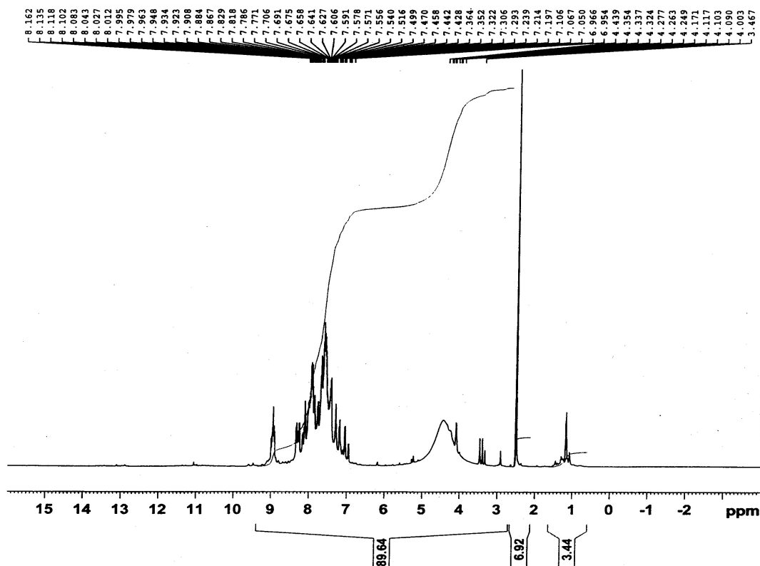
Appendix 3-15: NMR spectrum of 2-diethylmalonateazo-4-amino salicylic acid X
