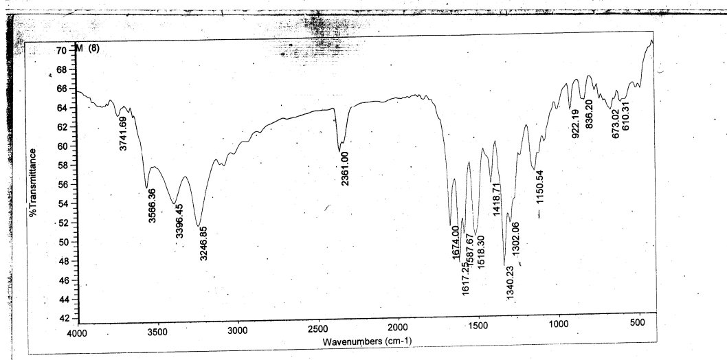
Appendix 3- 7: IR spectrum of 1-(2,4-dinitrobenzene pyrazol-3,5-dione) azo-4-sulphadoxine IV
