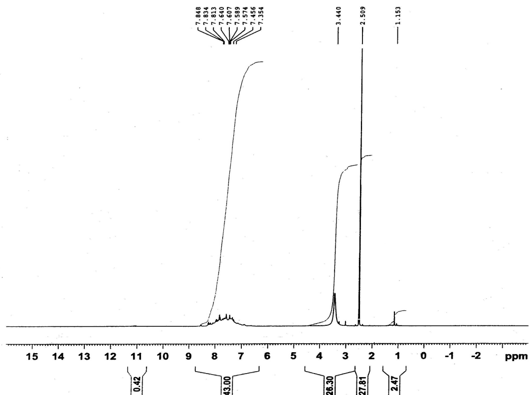
Appendix 3- 13: NMR spectrum of 2-diethylmalonateazo-4-sulphanilamideI
