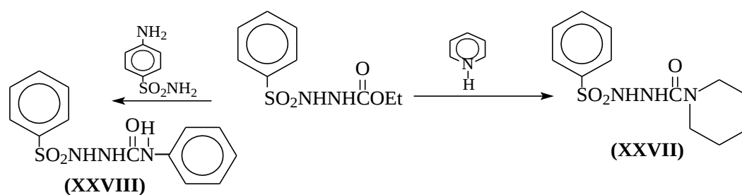
Scheme 2-9: Chemical structure of prepared
