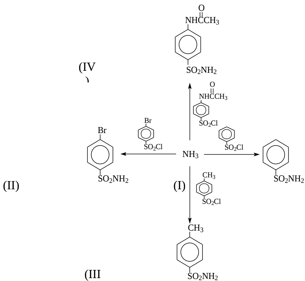
Scheme 2-1: Chemical Structure of the prepared sulphonamide
