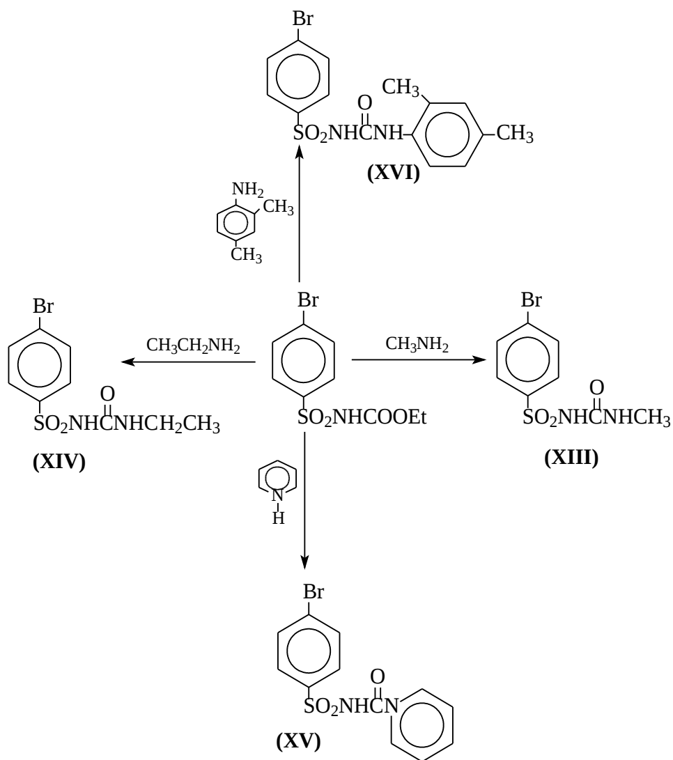
Scheme 2-4: Chemical structure of prepared p-Bromobenzene sulphonyl ureas
