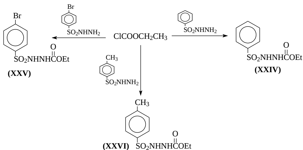
Scheme 2-8: Chemical structure of prepared sulphonyl carbazate
