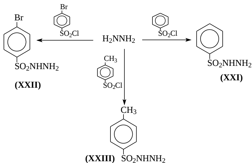
Scheme 2-7: Chemical structure of prepared sulphonyl hydrazide
