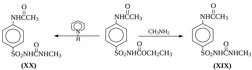
Scheme 2-6: Chemical structure of prepared p-acetamidobenzene sulphonyl ureas
