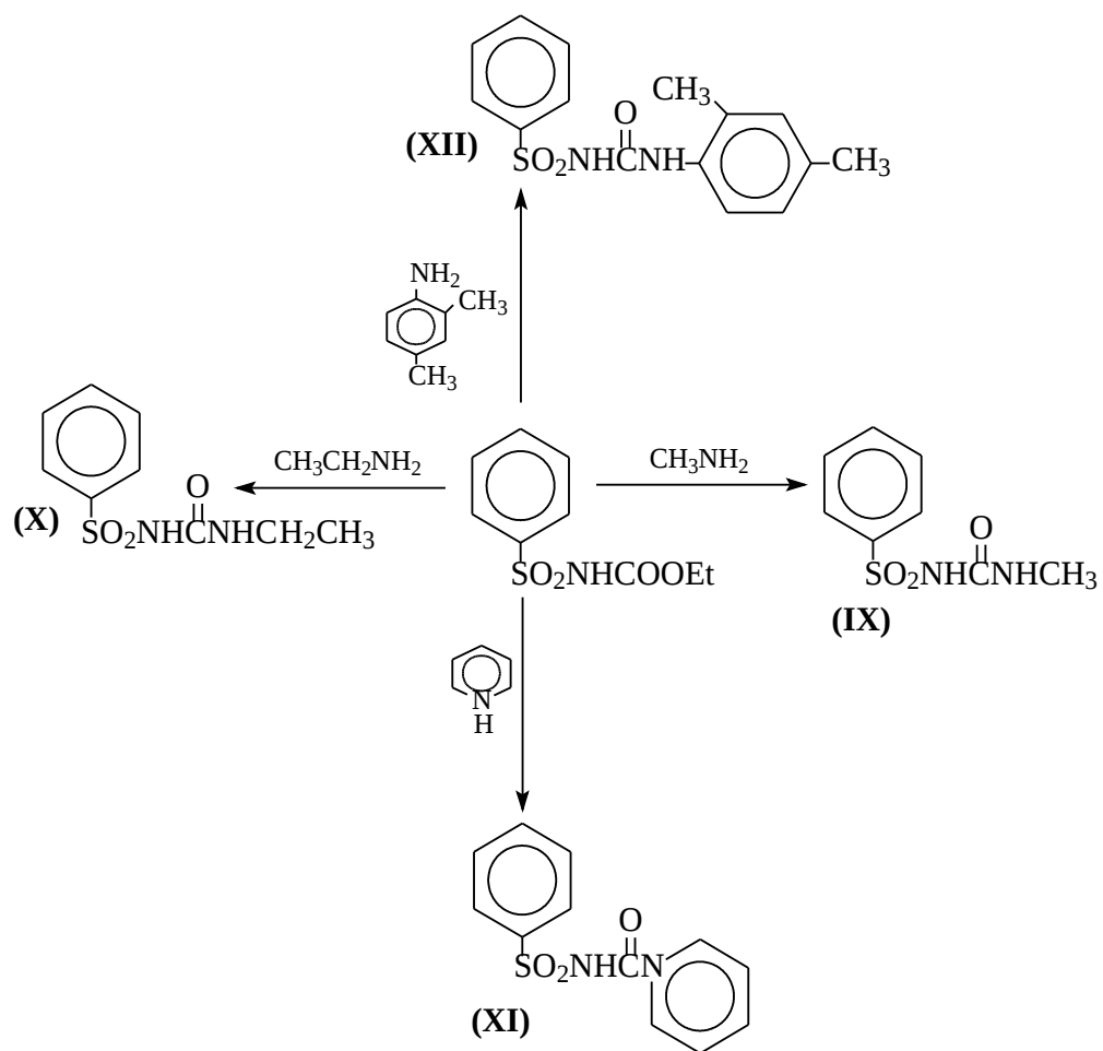
Scheme 2-3: Chemical structure of prepared benzene sulphonyl ureas
