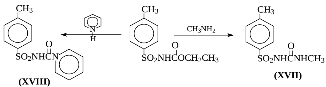
Scheme 2-5: Chemical structure of prepared toluene sulphonyl ureas
