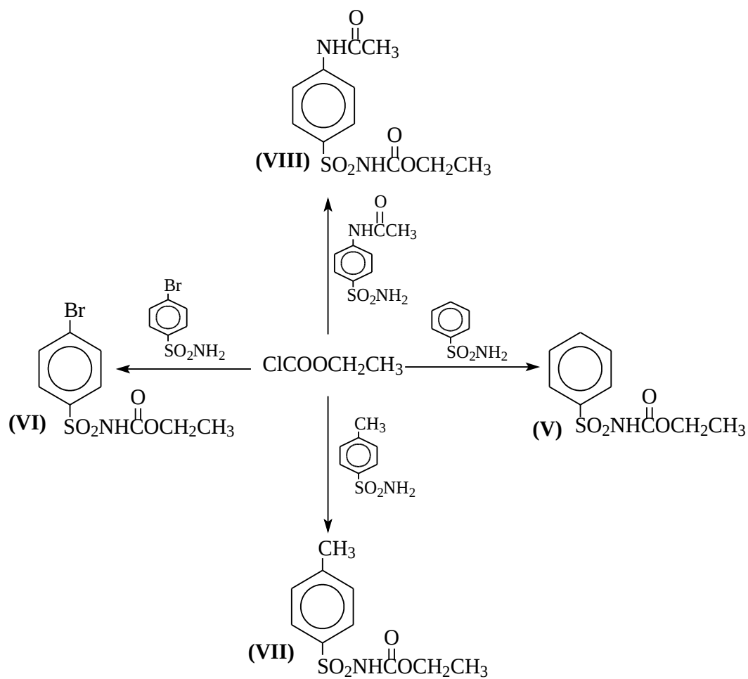
Scheme 2-2: Chemical Structure of the prepared carbamate
