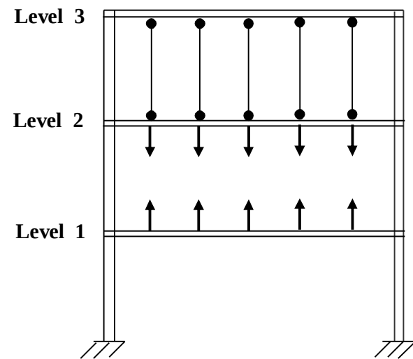
(c) Step 7 : Removal of Shores Under Level 2
