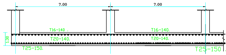
COLUMN STRIP
