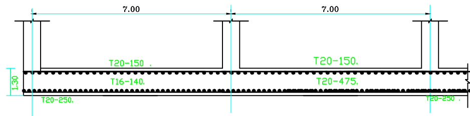
MIDDLE STRIP
