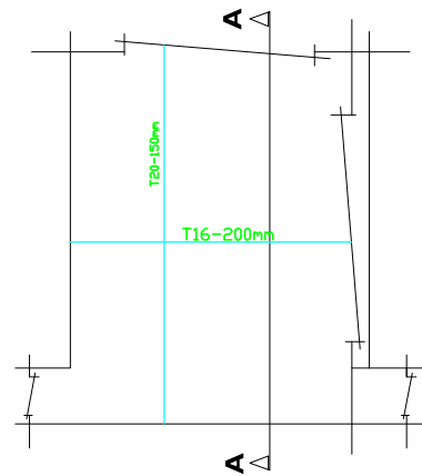
shear wall
