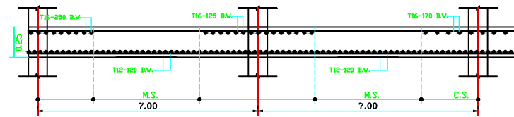
SEC M-M AT COLUMN STRIP
