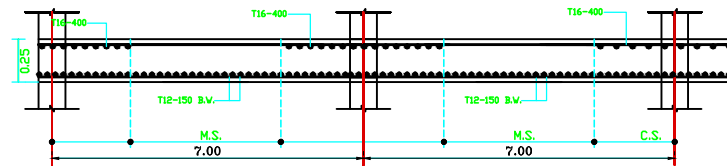
SEC N-N AT MIDDLE STRIP
