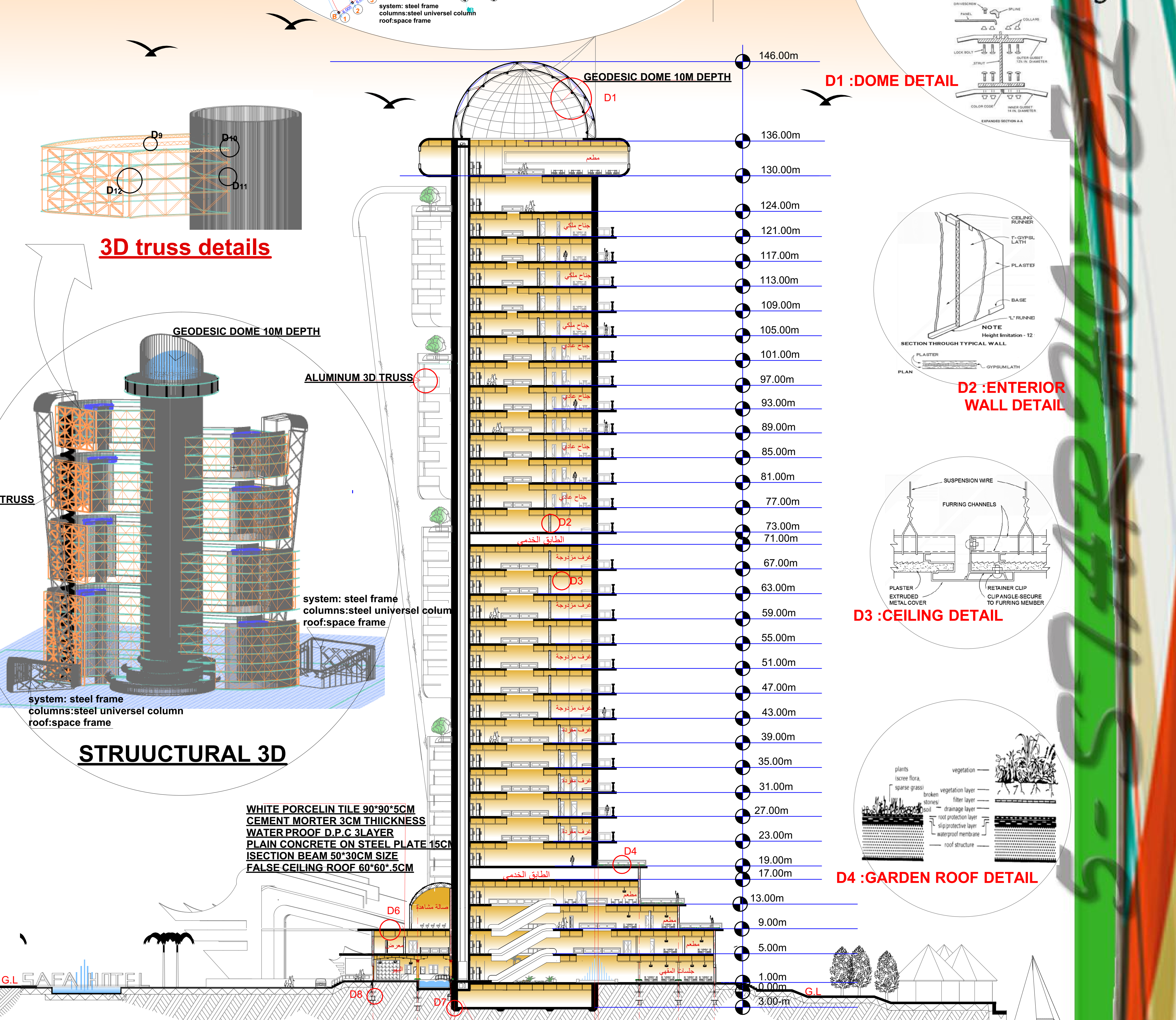
SECTION B-B -- scale (1:300)
