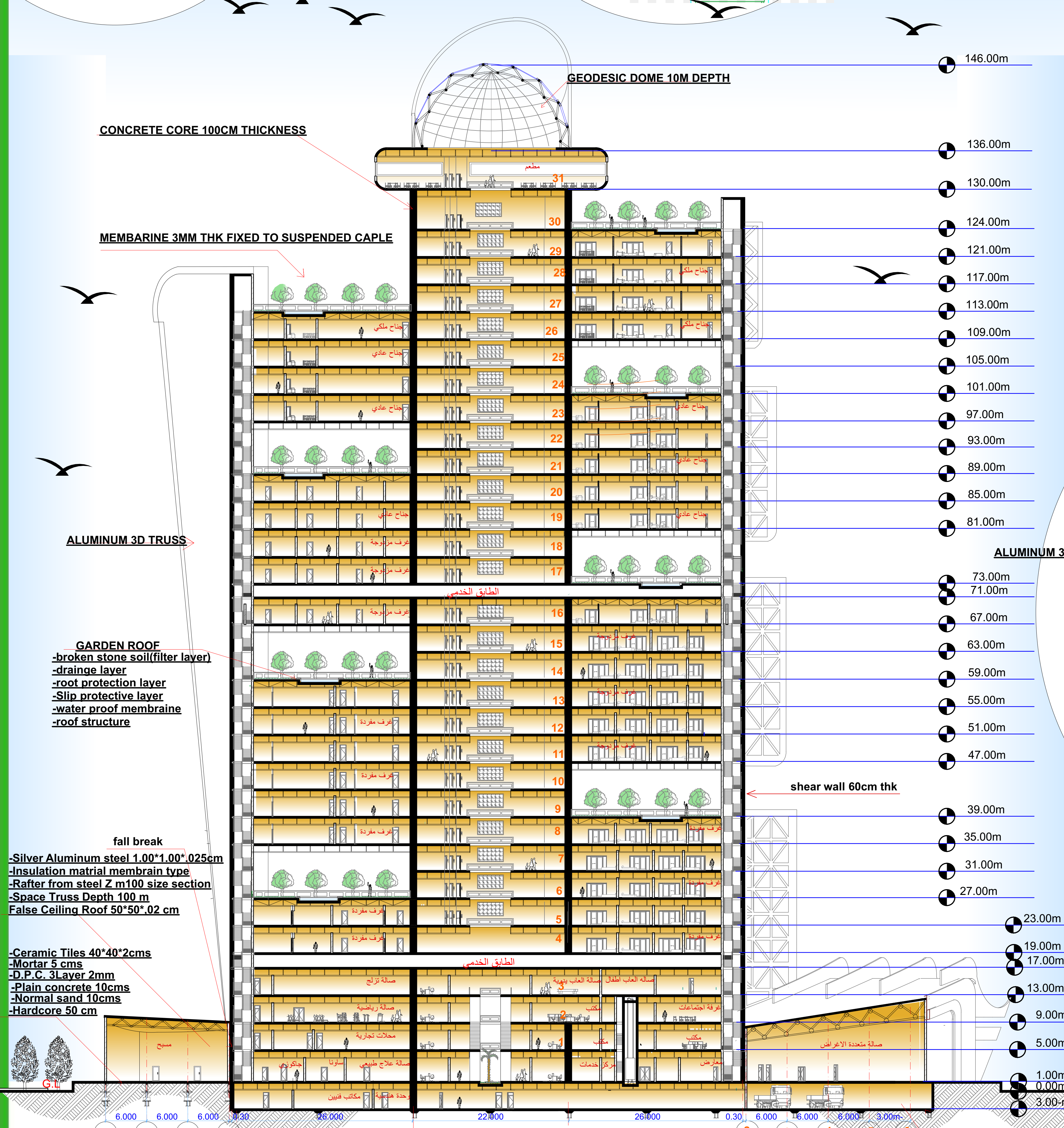
SECTION A-A -- scale (1:300)
