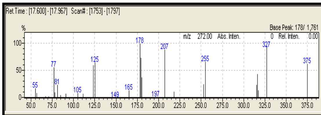
Appendix D.1: MS spectrum of 2,3-Diphenyl-6-(5,6-dimethoxy-4-sulphamido-pyrimidine)-quinoline-4-carboxylic acid (XXIII).
