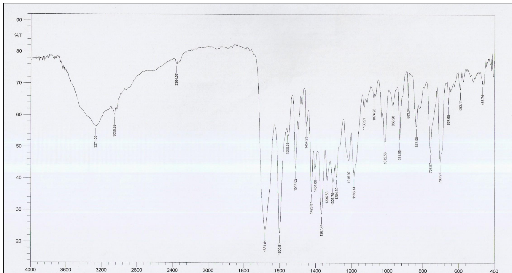
Appendix A.3: IR spectrum of 2,3-Diphenyl-6-(5-furyl-oxazole-3-yl)-quinoline-4-carboxylic acid ( XIII ).
