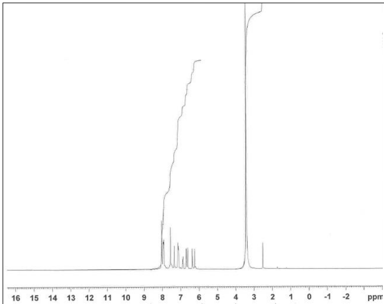
Appendix B.2: ^1\text{H} NMR spectrum of 2-Furyl-3-phenyl-6-(3-furyl-prop-2-en-1-one-1-yl)-quinoline-4-carboxylic acid ( VIII ).
