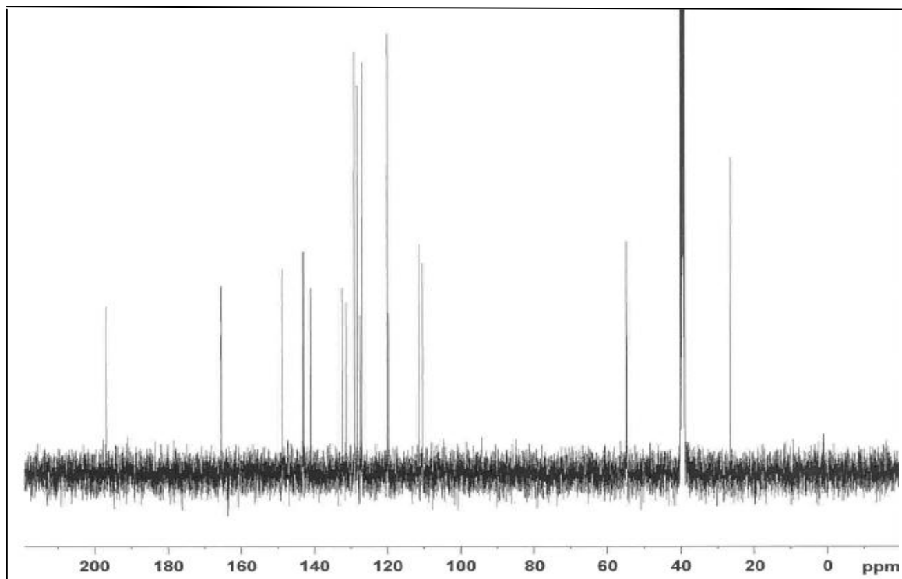
Appendix C.1: ^{13}\text{C} NMR spectrum of 2-Furyl-3-phenyl-6-acetyl-quinoline-4-carboxylic acid ( II ).
