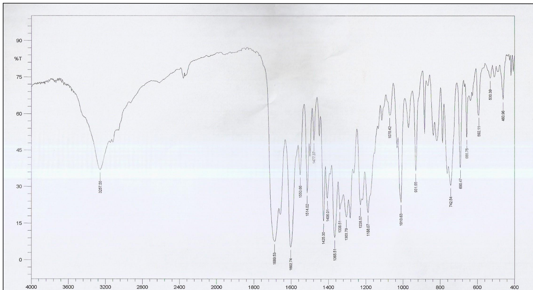
Appendix A.4: IR spectrum of 2-Furyl-3-phenyl-6-(5-furyl-oxazole-3-yl)-quinoline-4-carboxylic acid ( XVII ).
