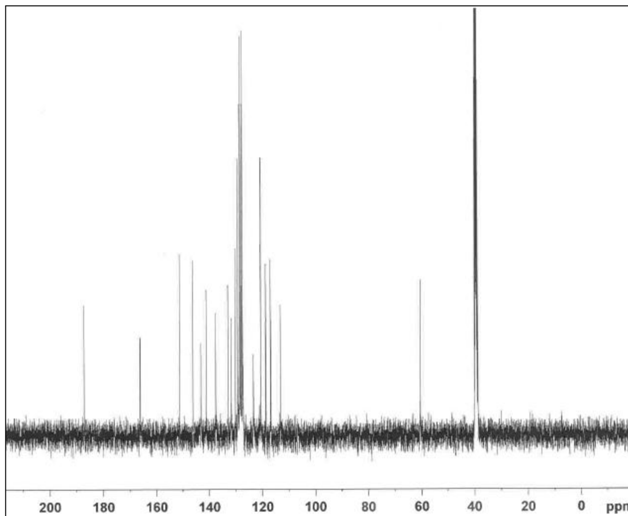
Appendix C.3: ^{13}\text{C} NMR spectrum of 2,3-Diphenyl-6-(5-furyl-oxazole-3-yl)-quinoline-4-carboxylic acid ( XIII ).
