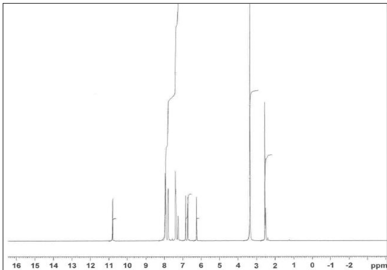
Appendix B.1: ^1\text{H} NMR spectrum of 2-Furyl-3-phenyl-6-acetyl-quinoline-4-carboxylic acid ( II ).
