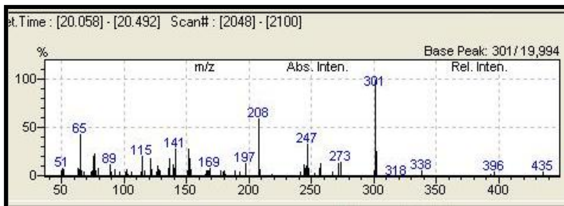
Appendix D.2: MS spectrum of 2,3-Diphenyl-6-(3-furyl-prop-2-en-1-one-1-yl)-quinoline-4-carboxylic acid (IV).
