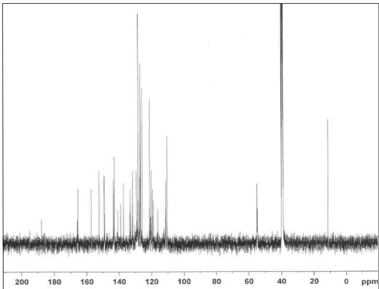
Appendix C.5: ^{13}\text{C} NMR spectrum of 2-Furyl-3-phenyl-6-(5-[2-hydroxyphenyl]-oxazole-3-yl)-quinoline-4-carboxylic acid ( XX ).
