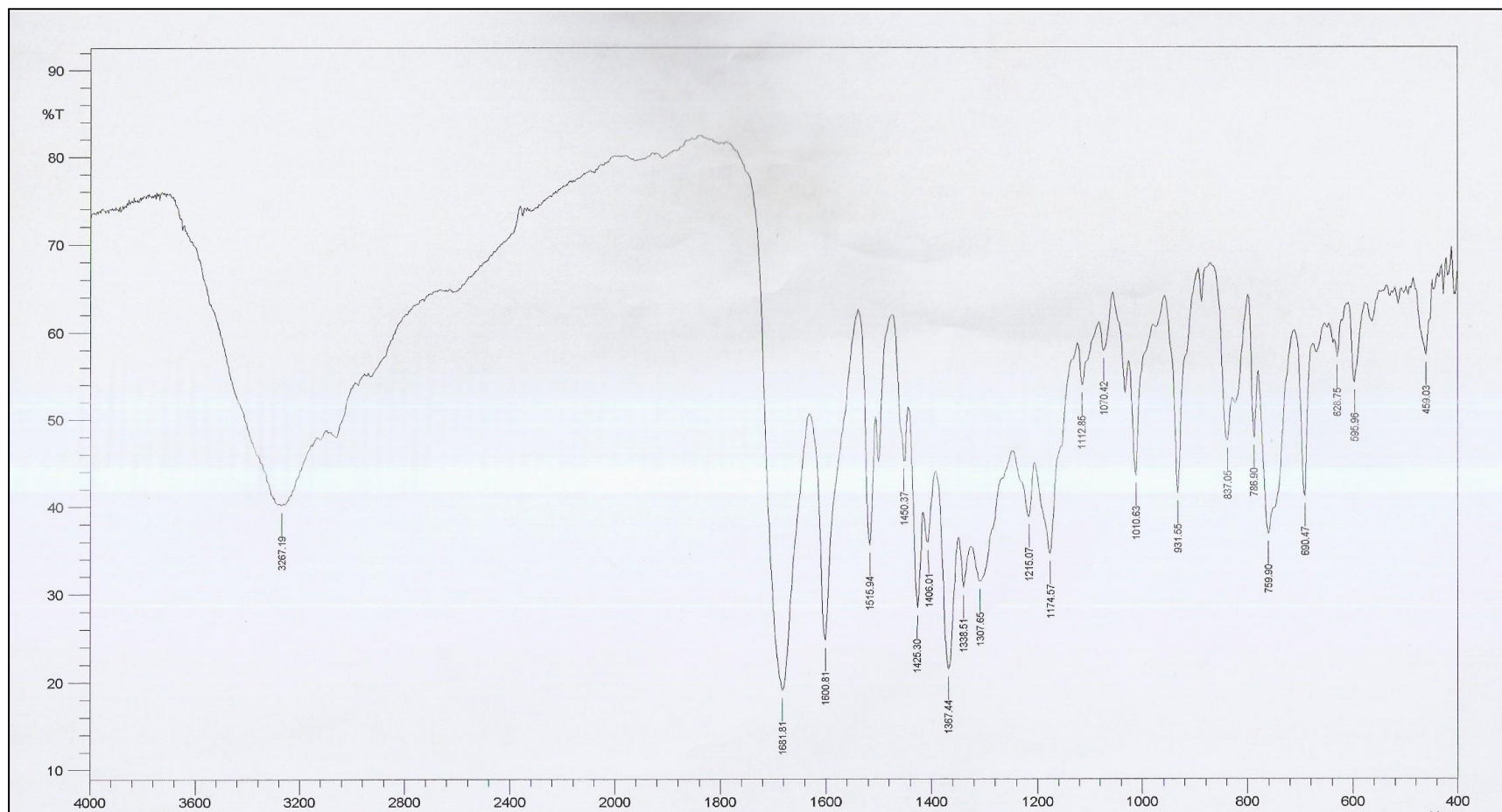
Appendix A.5: IR spectrum of 2-Furyl-3-phenyl-6-(5-[2-hydroxyphenyl]-oxazole-3-yl)-quinoline-4-carboxylic acid (XX).
