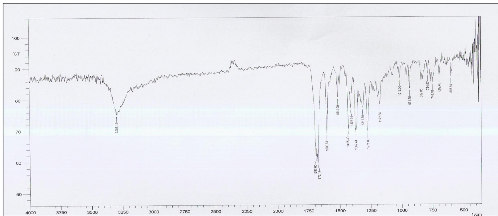
Appendix A.1: IR spectrum of 2-Furyl-3-phenyl-6-acetyl-quinoline-4-carboxylic acid ( II ).
