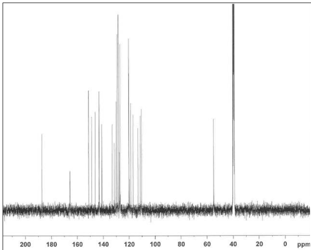
Appendix C.4: ^{13}\text{C} NMR spectrum of 2-Furyl-3-phenyl-6-(5-furyl-oxazole-3-yl)-quinoline-4-carboxylic acid ( XVII ).
