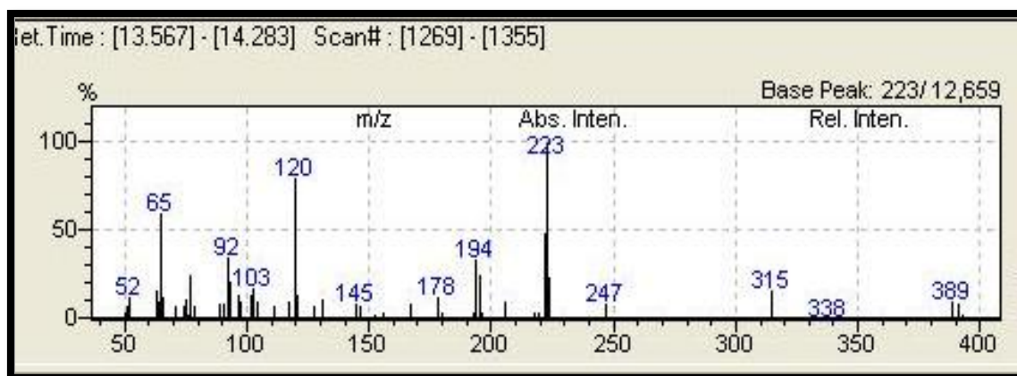
Appendix D.3: MS spectrum of 2,3-Diphenyl-6-(3-[3-N,N-dimethylamino phenyl]-prop-2-en-1-one-1-yl)-quinoline-4-carboxylic acid ( VI ).
