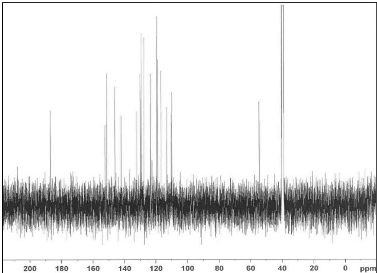
Appendix C.2: ^{13}\text{C} NMR spectrum of 2-Furyl-3-phenyl-6-(3-furyl-prop-2-en-1-one-1-yl)-quinoline-4-carboxylic acid ( VIII ).
