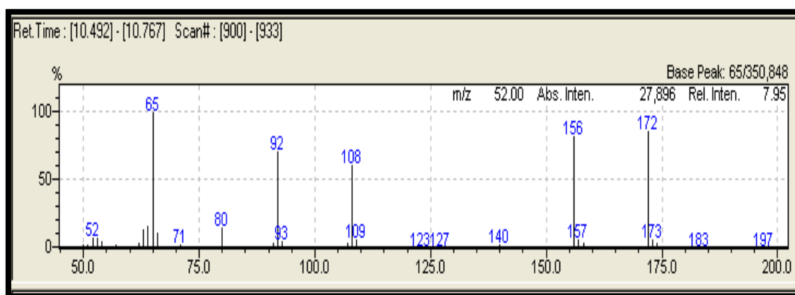
Appendix D.4: MS spectrum of 2,4-Dimethyl quinoline-6-sulphamide ( XXIV ).
