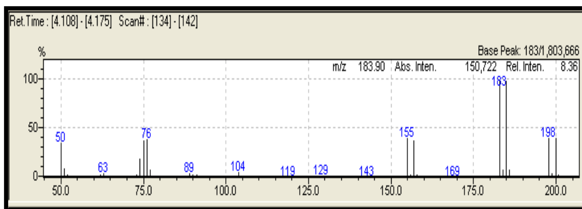
Appendix D.5: MS spectrum of 4-Methyl-2-hydroxyquinoline-6-sulphamide ( XXV ).
