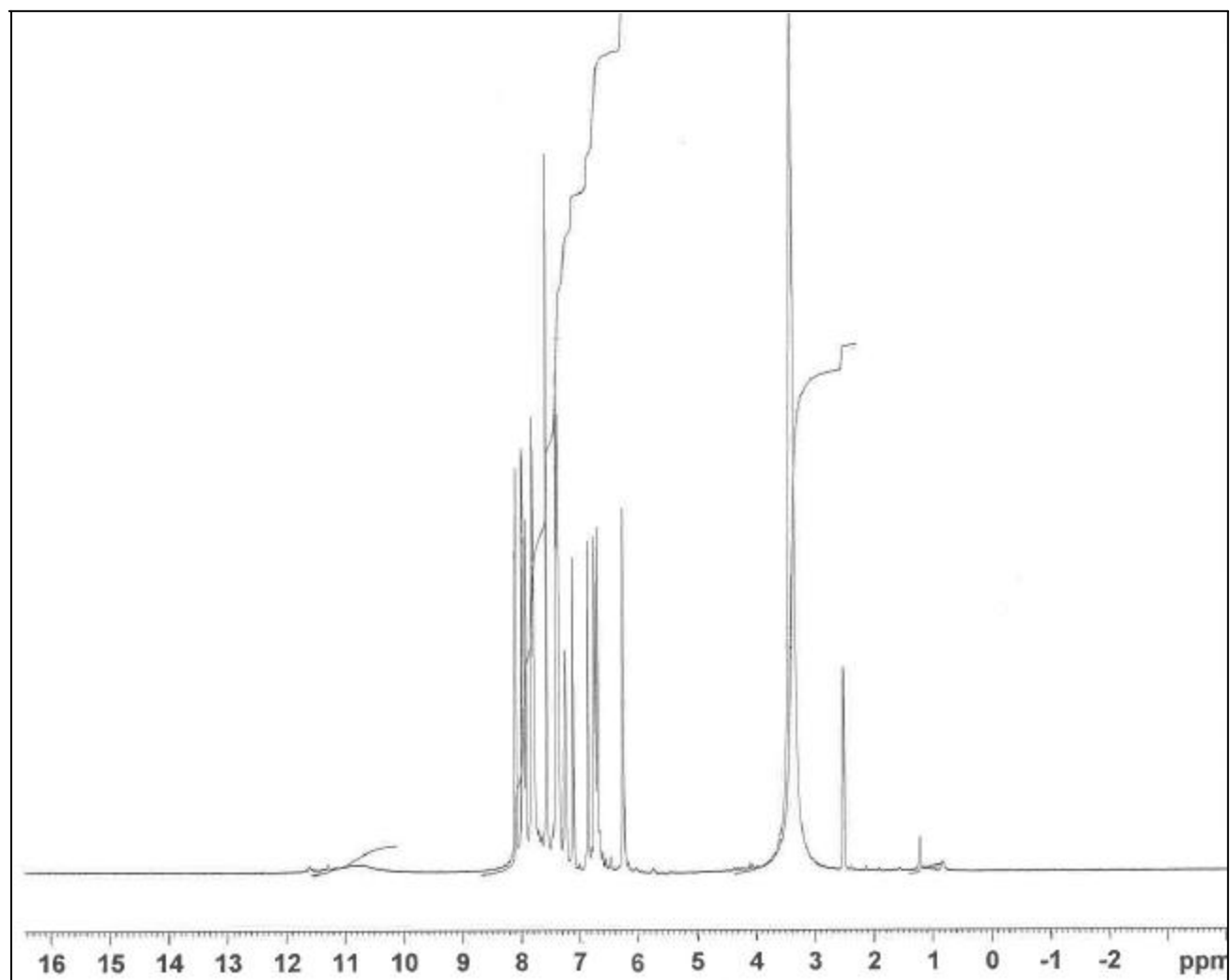
Appendix B.4: ^1\text{H} NMR spectrum of 2-Furyl-3-phenyl-6-(5-furyl-oxazole-3-yl)-quinoline-4-carboxylic acid ( XVII ).
