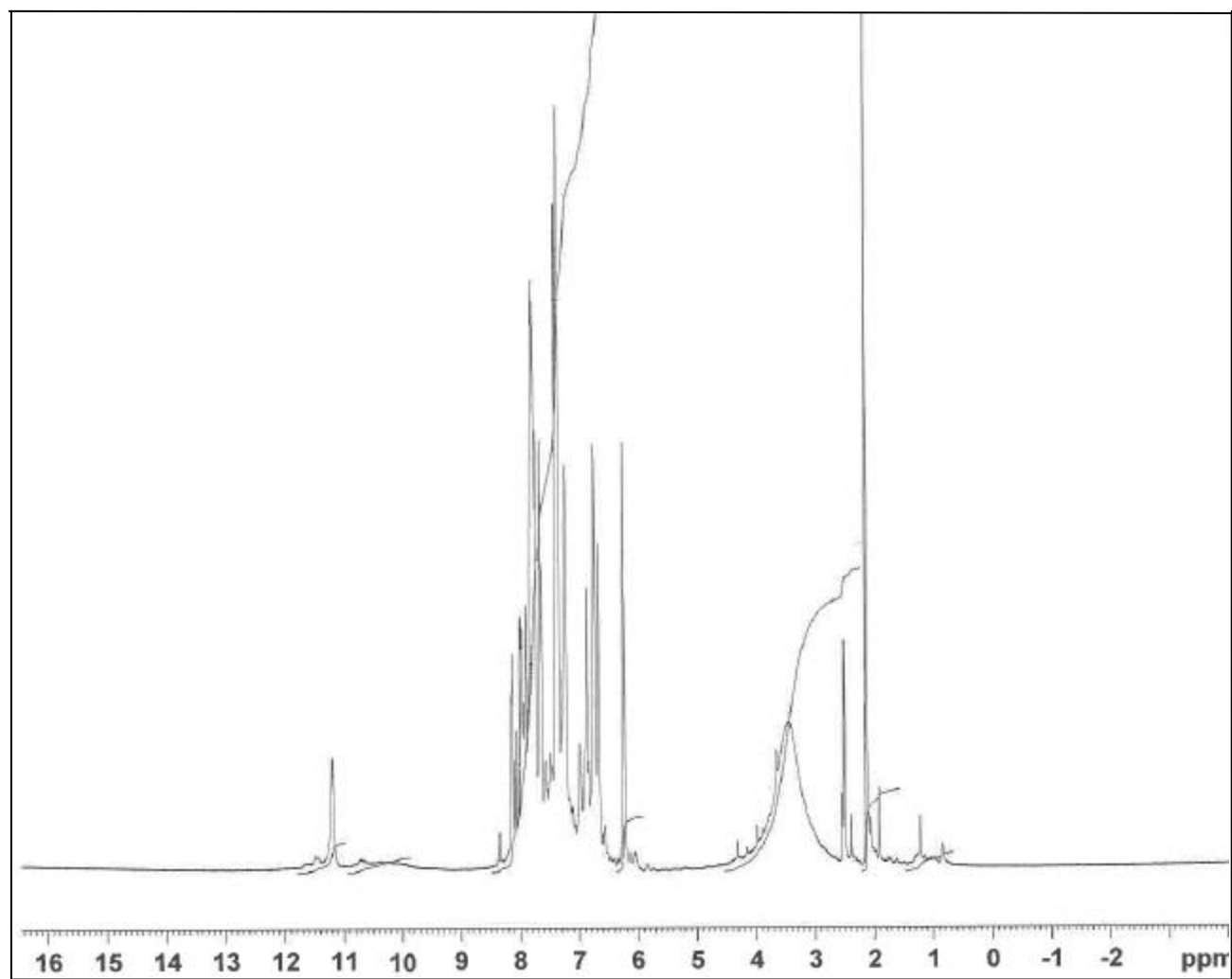
Appendix B.5: ^1\text{H} NMR spectrum of 2-Furyl-3-phenyl-6-(5-[2-hydroxyphenyl]-oxazole-3-yl)-quinoline-4-carboxylic acid ( XX ).
