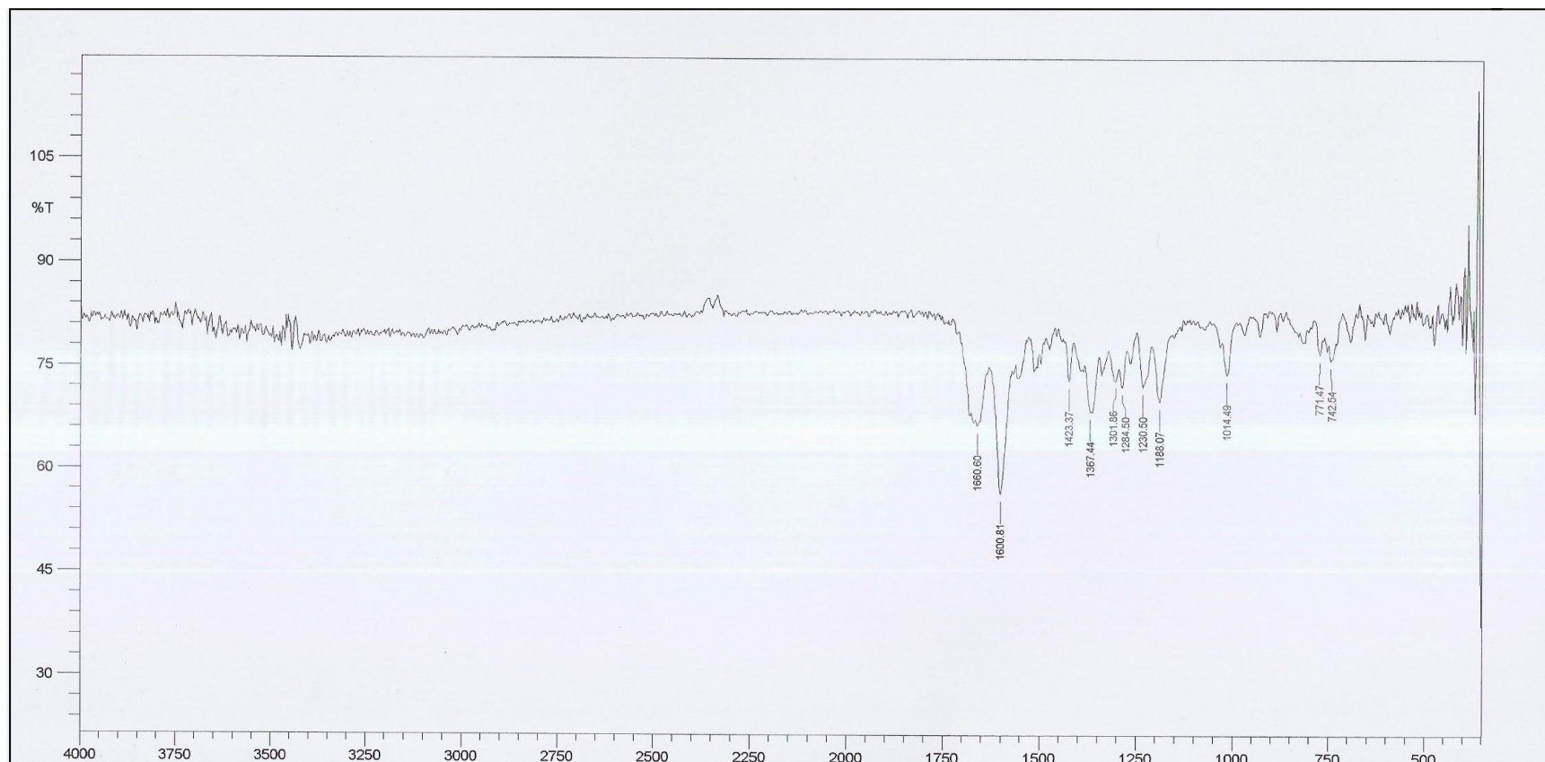
Appendix A.2: IR spectrum of 2-Furyl-3-phenyl-6-(3-furyl-prop-2-en-1-one-1-yl)-quinoline-4-carboxylic acid (VIII).
