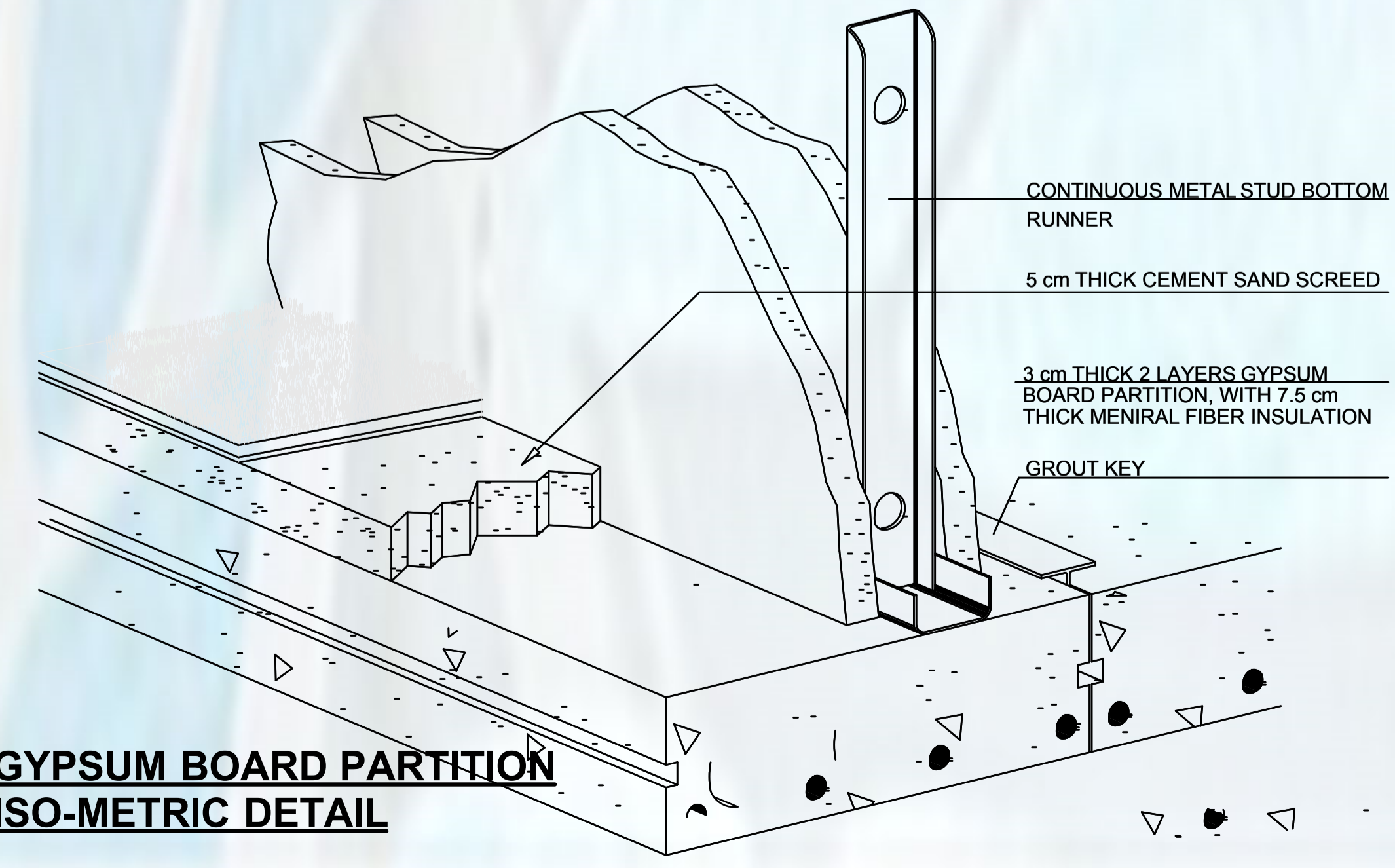
GYPSUM BOARD PARTITION DETAIL SCALE 1:10
