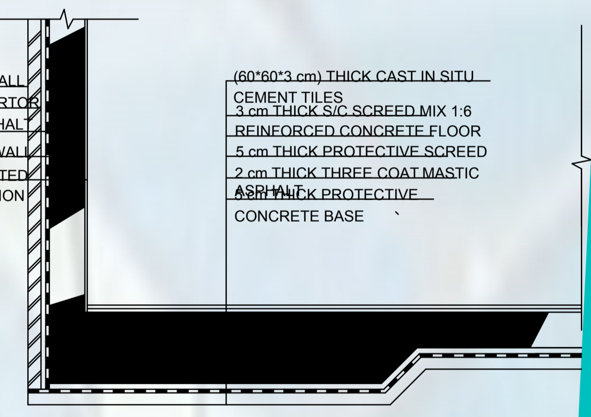
DETAIL 1
