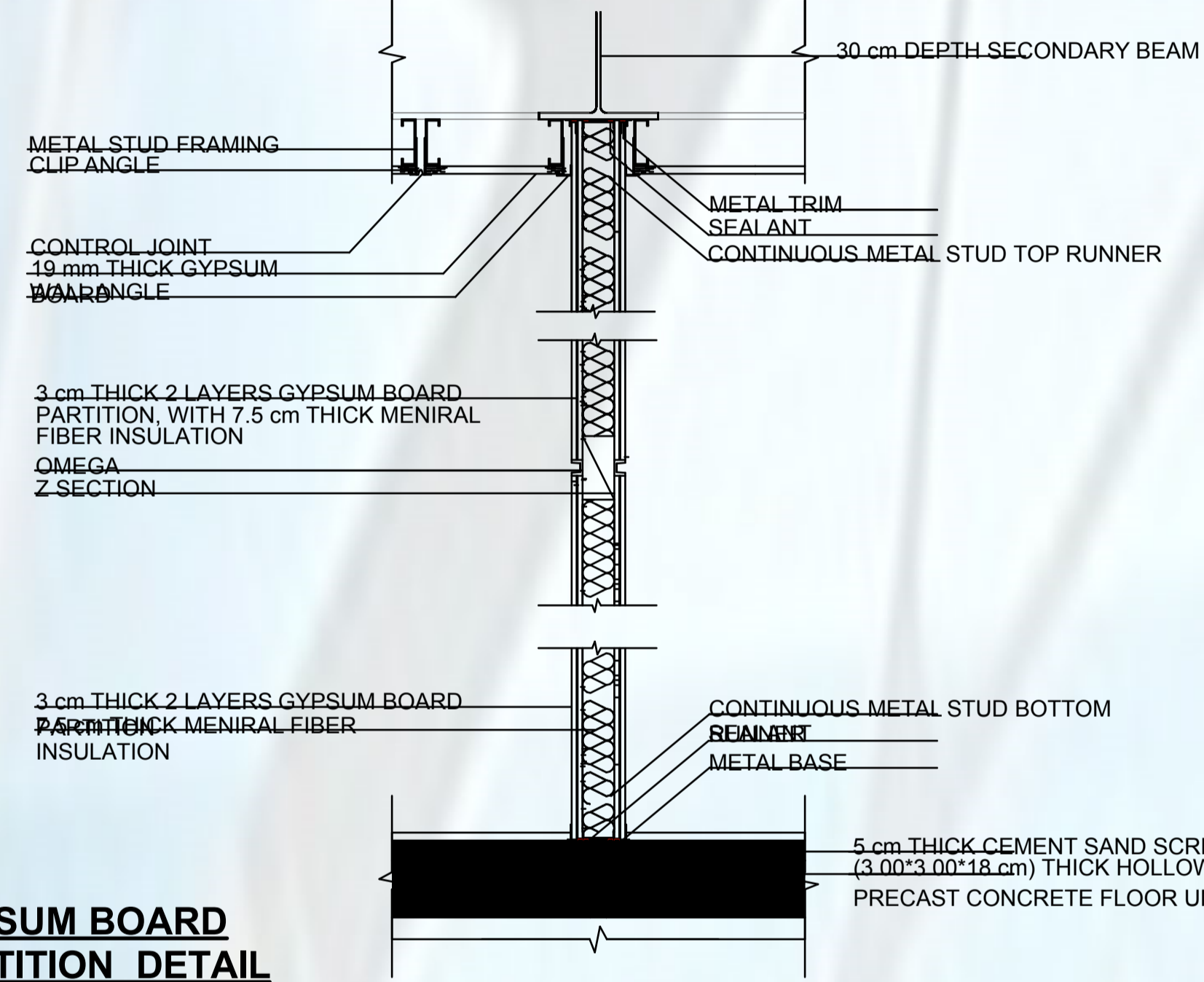
DETAIL 1
