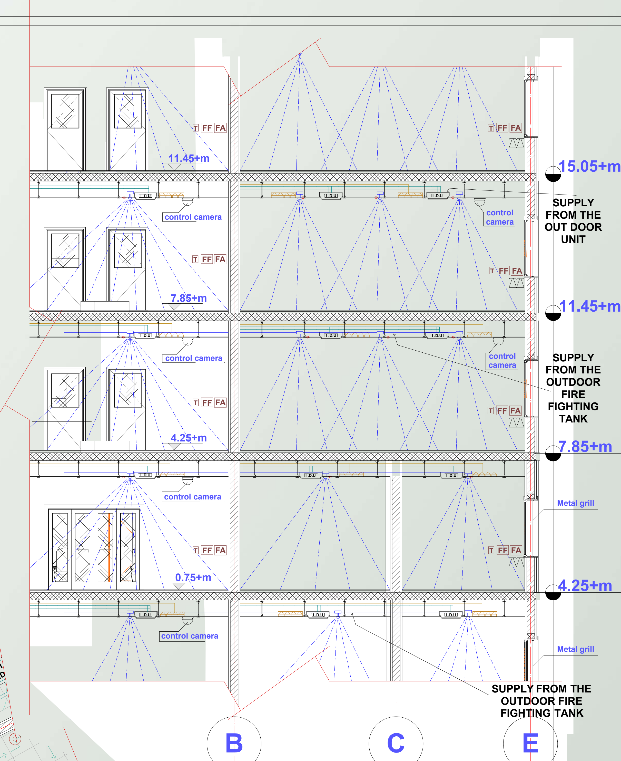
PART SECTION C-C : Four Bedded Wards Scale : 1:50
