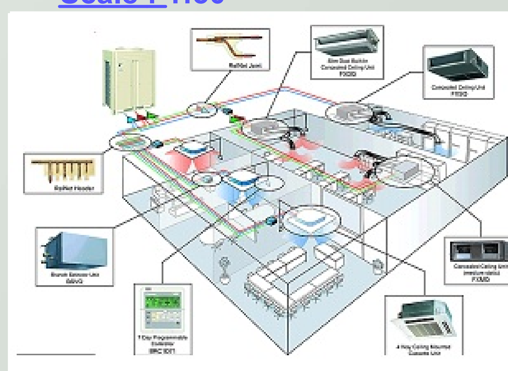
PART PLAN : Four Bedded Wards Scale : 1:50
