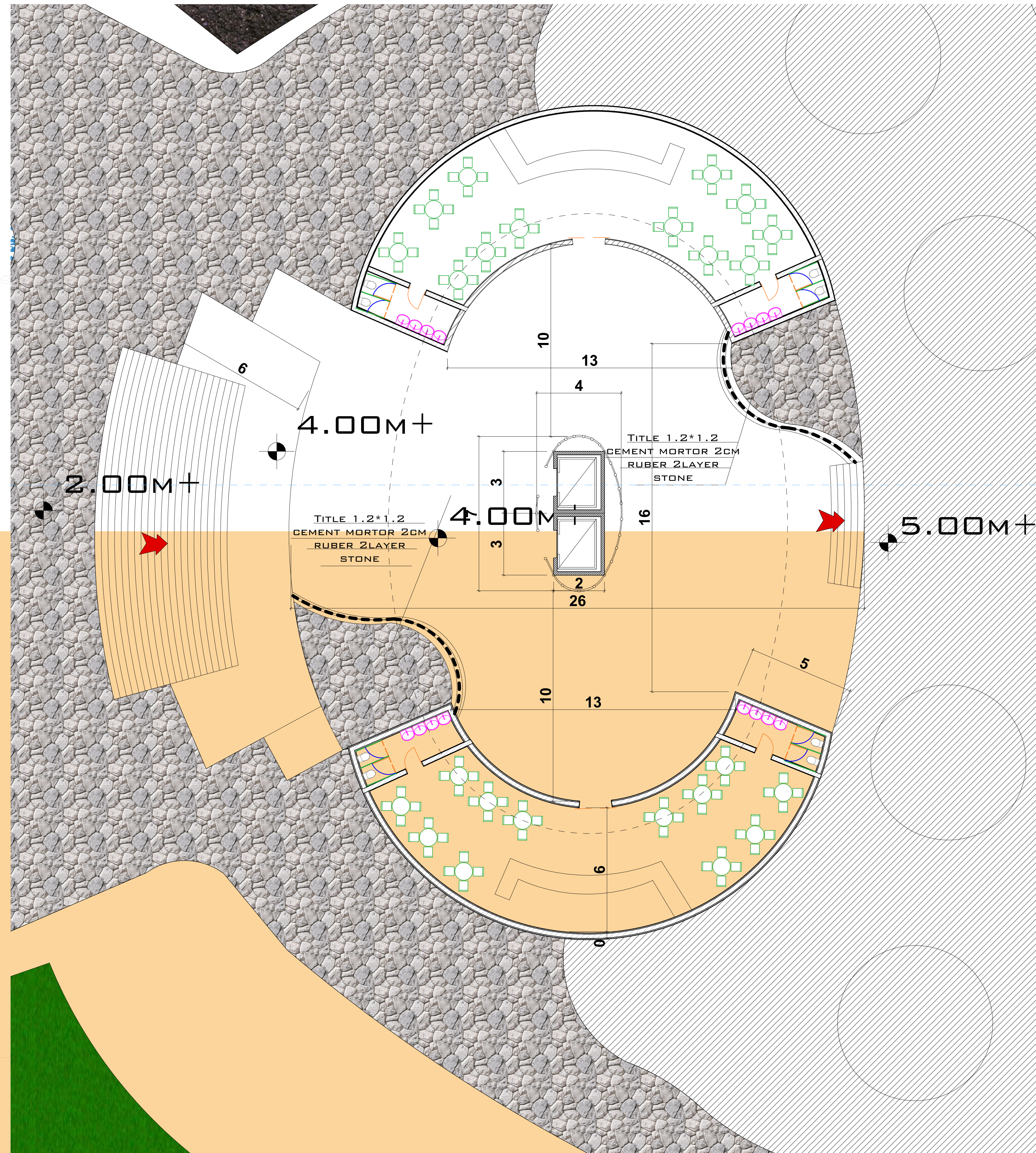
PART PLAN SCALE 1:100
