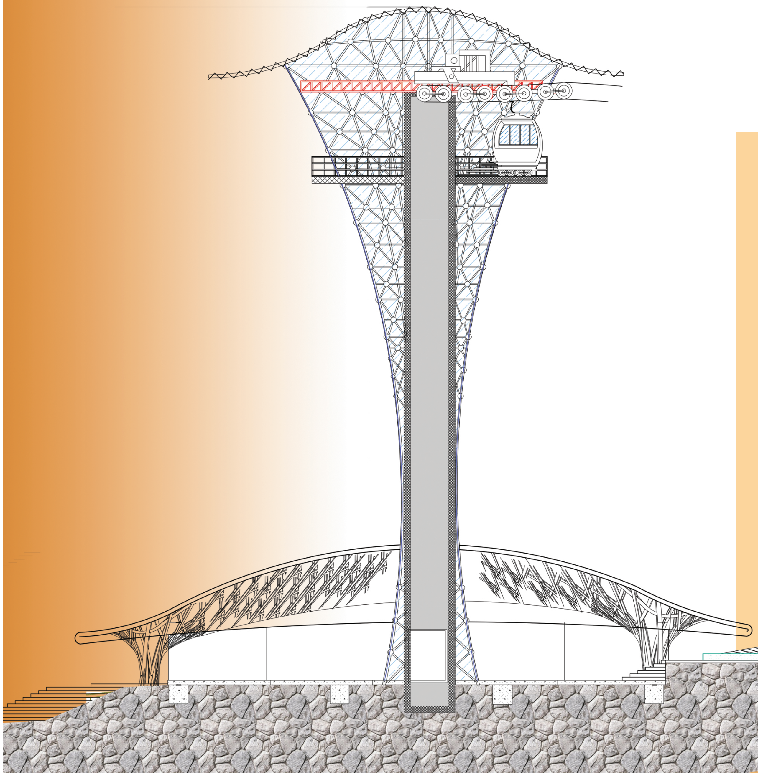
PART SECTION SCALE 1:100
