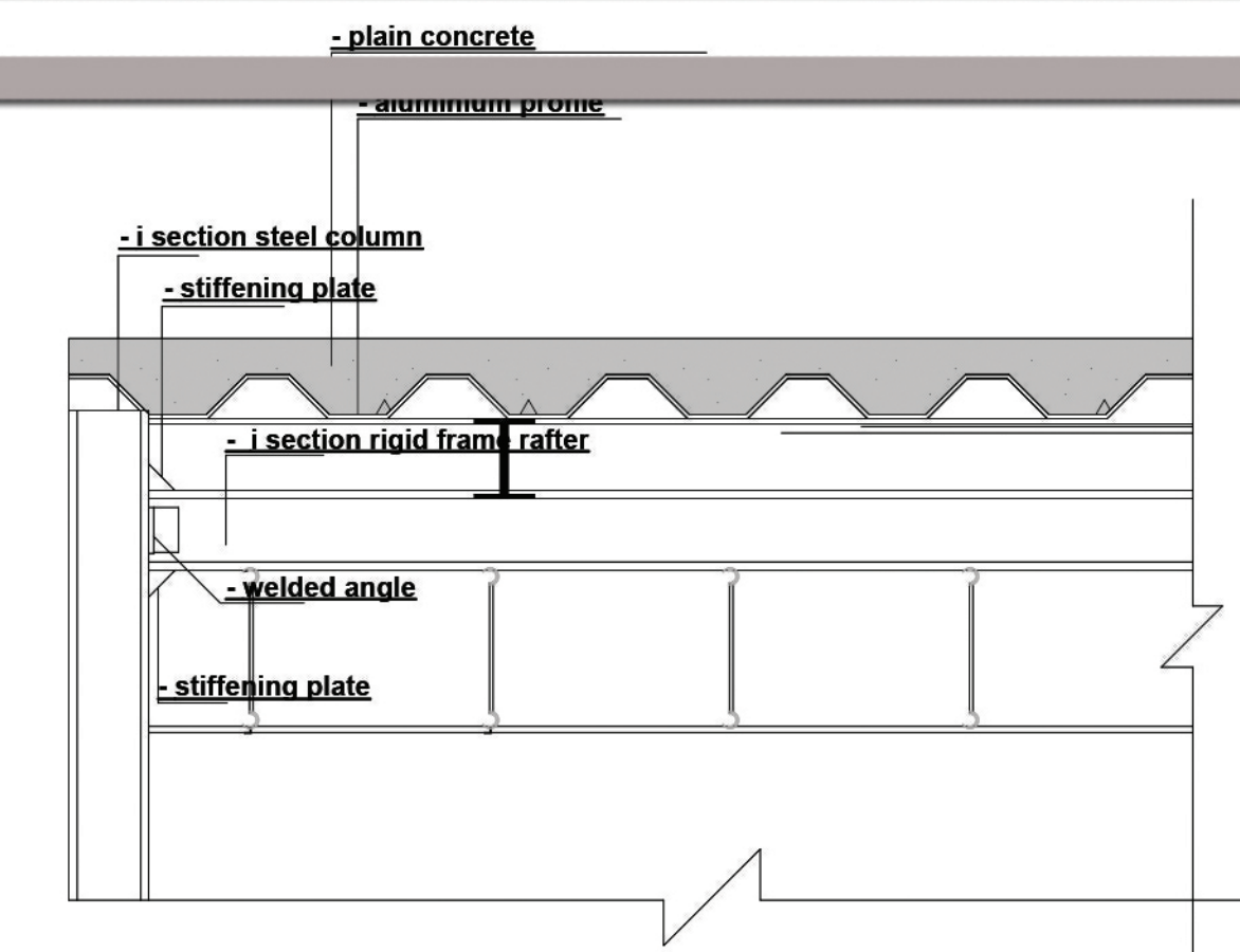
column joint with beam scale 1: 20
