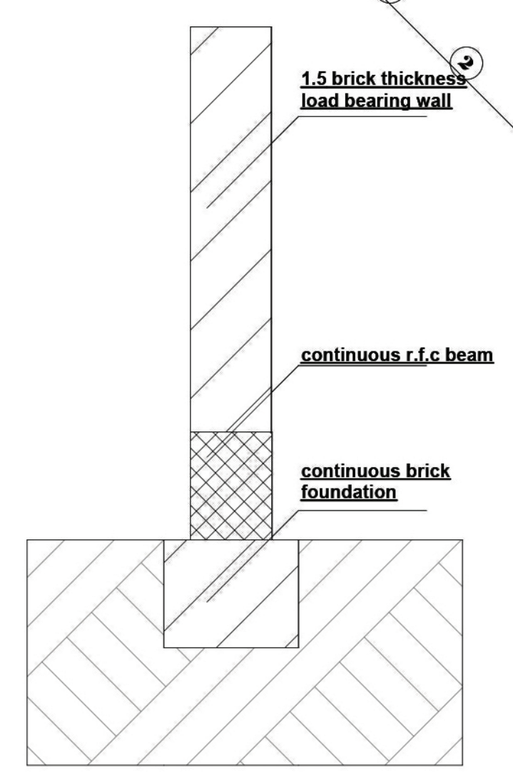
- load bearing wall detail no.3 - scale 1: 20
