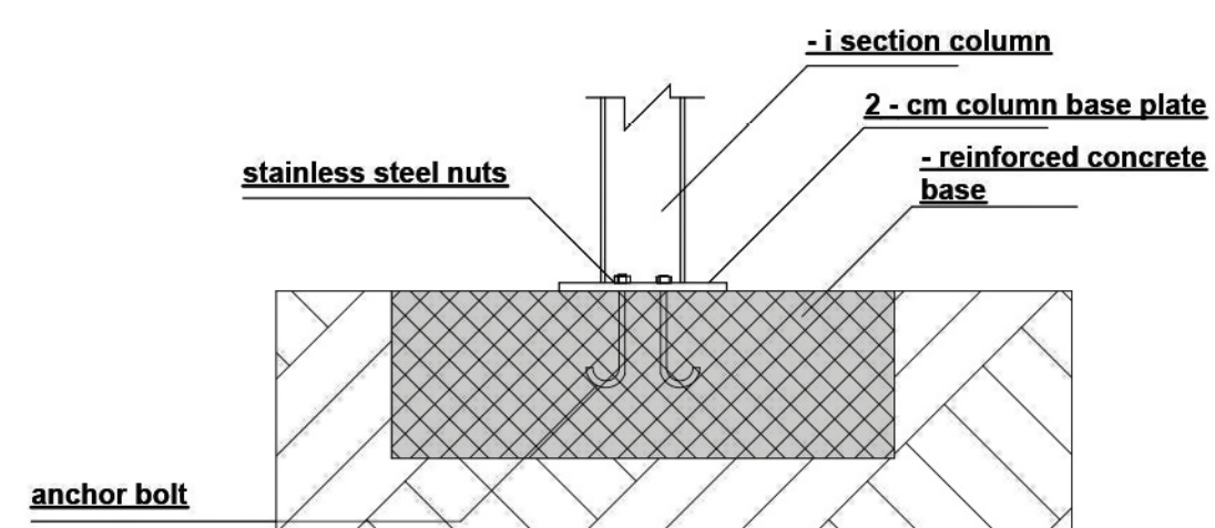
column base detail scale 1: 20
