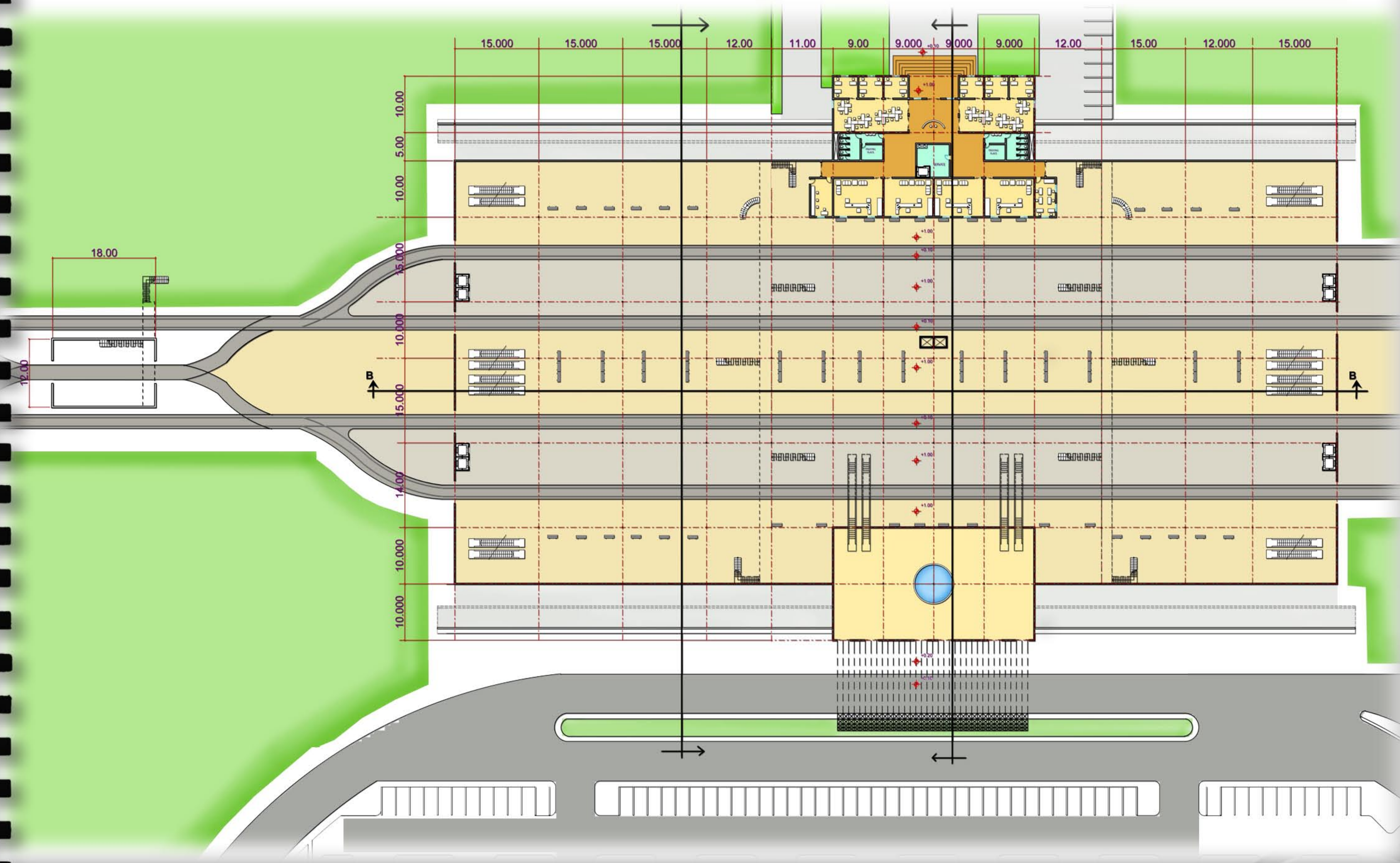
GROUND FLOOR PLAN SCALE 1:300
