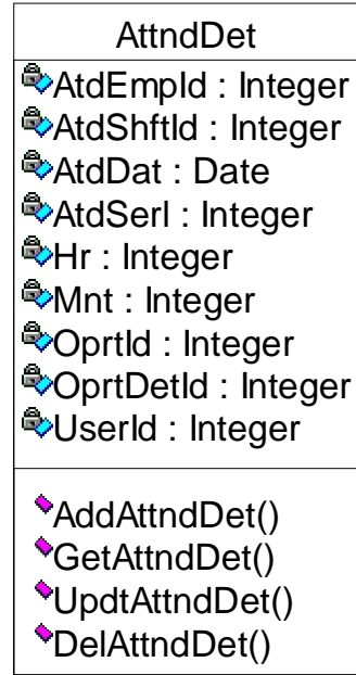
شکل ب.23: Attendance Detail Class
