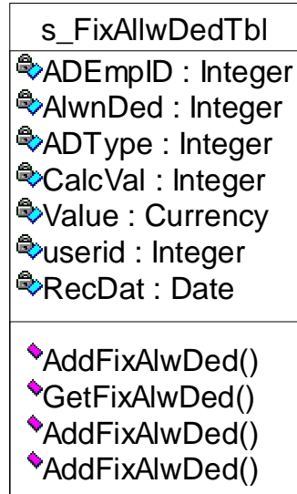
شکل ب.29: Fix Salary Allowances Class
