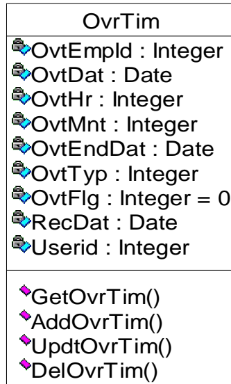
شکل ب.28: OverTime Class
