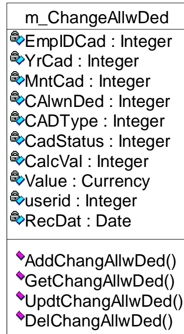
شکل ب.36: Change Allowances Class
