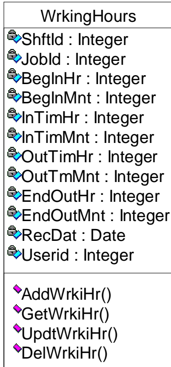
Working Hour Class :40. شکل ب.
