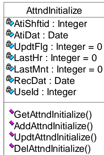
شکل ب.27: Attendance Initialize Class
