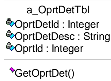
شکل ب.25: Operate Detail Class
