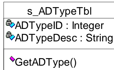
شکل ب.31: Allowances Type Class
