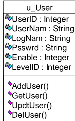
User Class :39. شکل ب.
