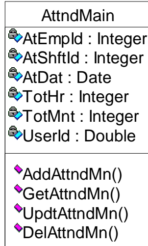
شکل ب.24: Attendance Main Class
