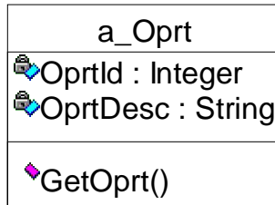
شکل ب.26: Operate Class
