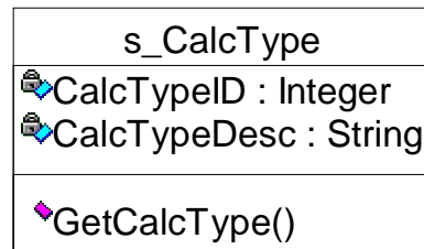
شکل ب.32: Salary Calculate Type Class
