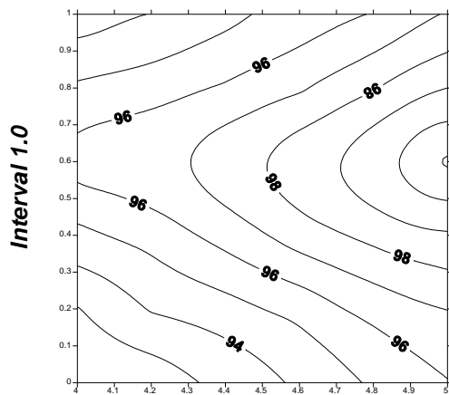
Fig (B.7): Contour map of the third test area (1×1km)
