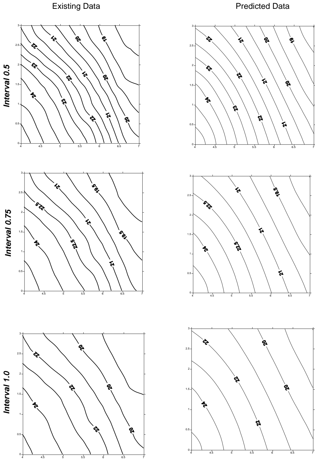
Fig (B.6): Contour map of the second test area (3×3km)
