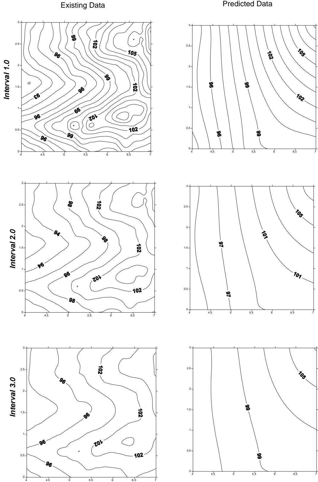
Fig (B.9): Contour map of the third test area (3×3km)
