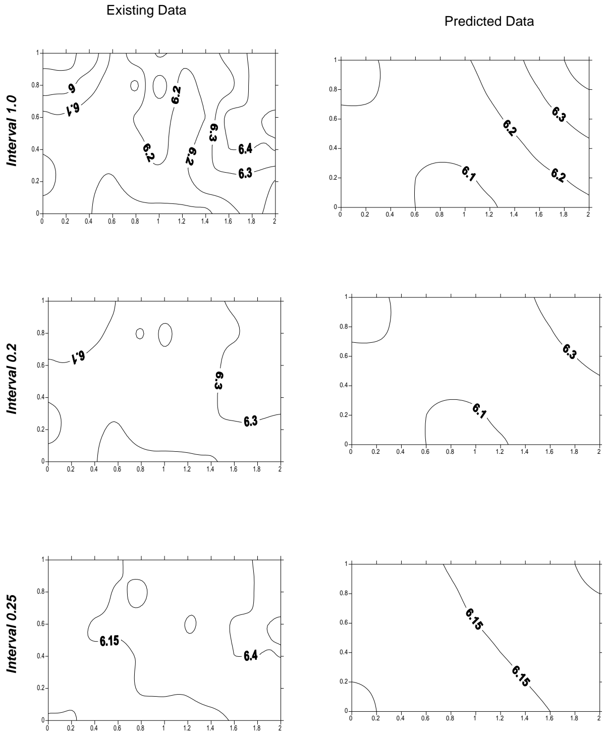
Fig (B.2): Contour map of the first test area (2×1 km)
