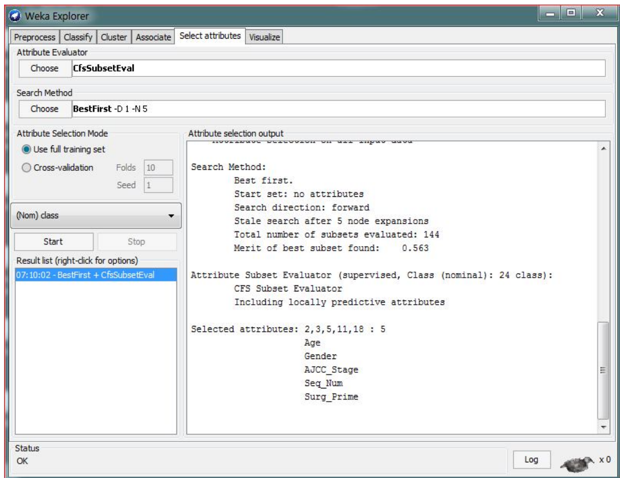
Figure A.1 Features Selected by CFS Method
