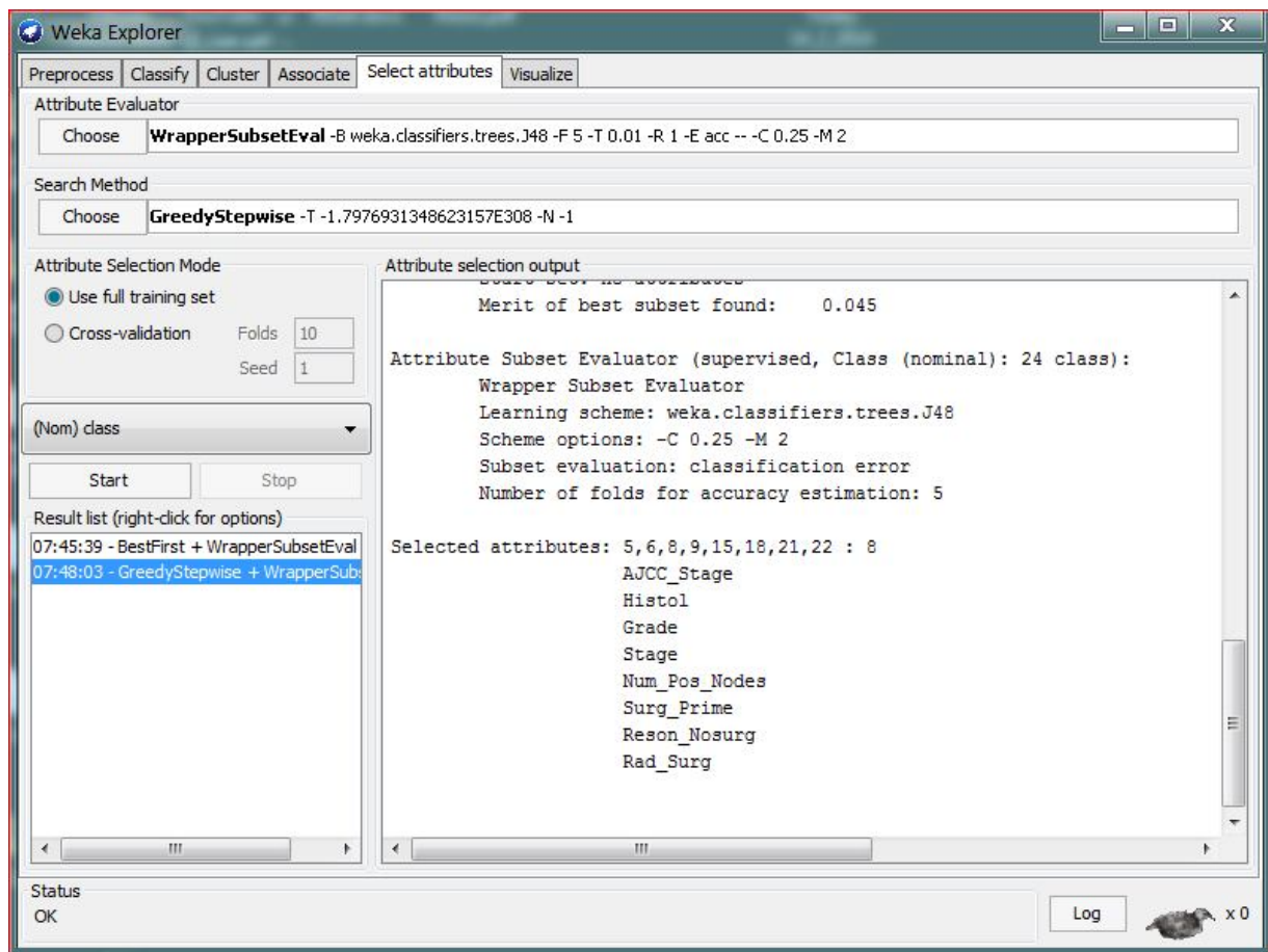
Figure A.2 Features Selected by Wrapper Method
