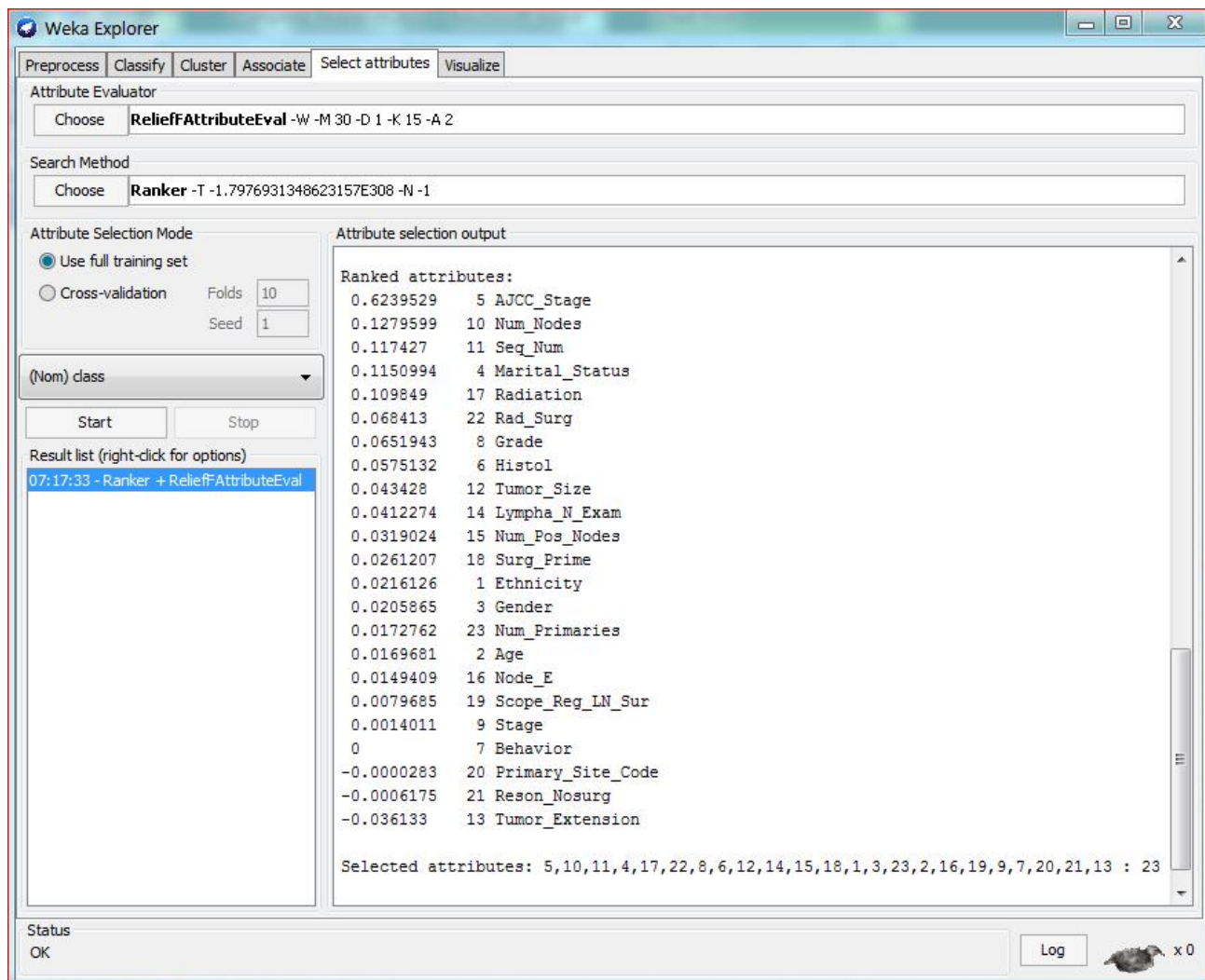
Figure A.3 Features Ranked by Relief Method
