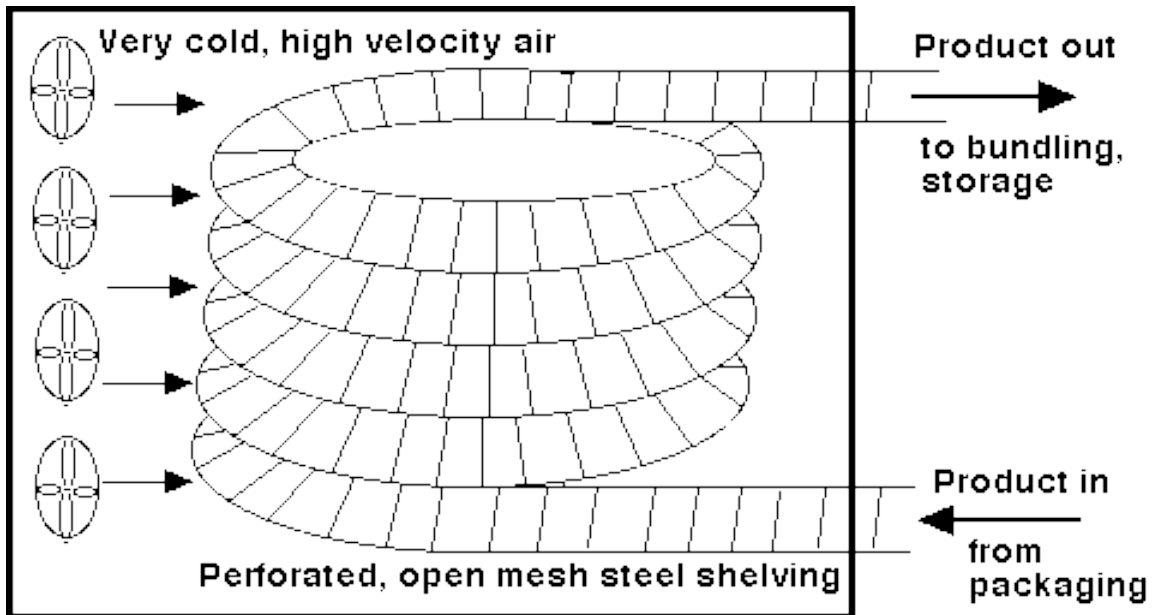
Spiral, wind tunnel freezer
