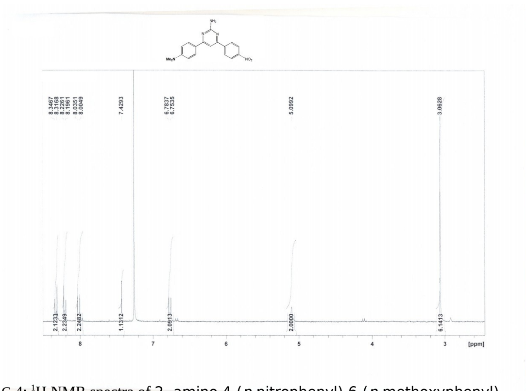
C.4: ^1\text{H} NMR spectra of 2- amino 4-( p -nitrophenyl)-6-( p -methoxyphenyl)pyrimidine [XXIII]
