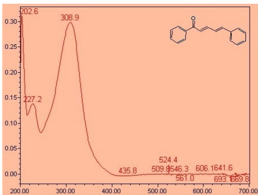
D.1: UV-Vis spectra of 1,5-diphenyl-(2E,4E)-pentadiene-1-one [IV]
