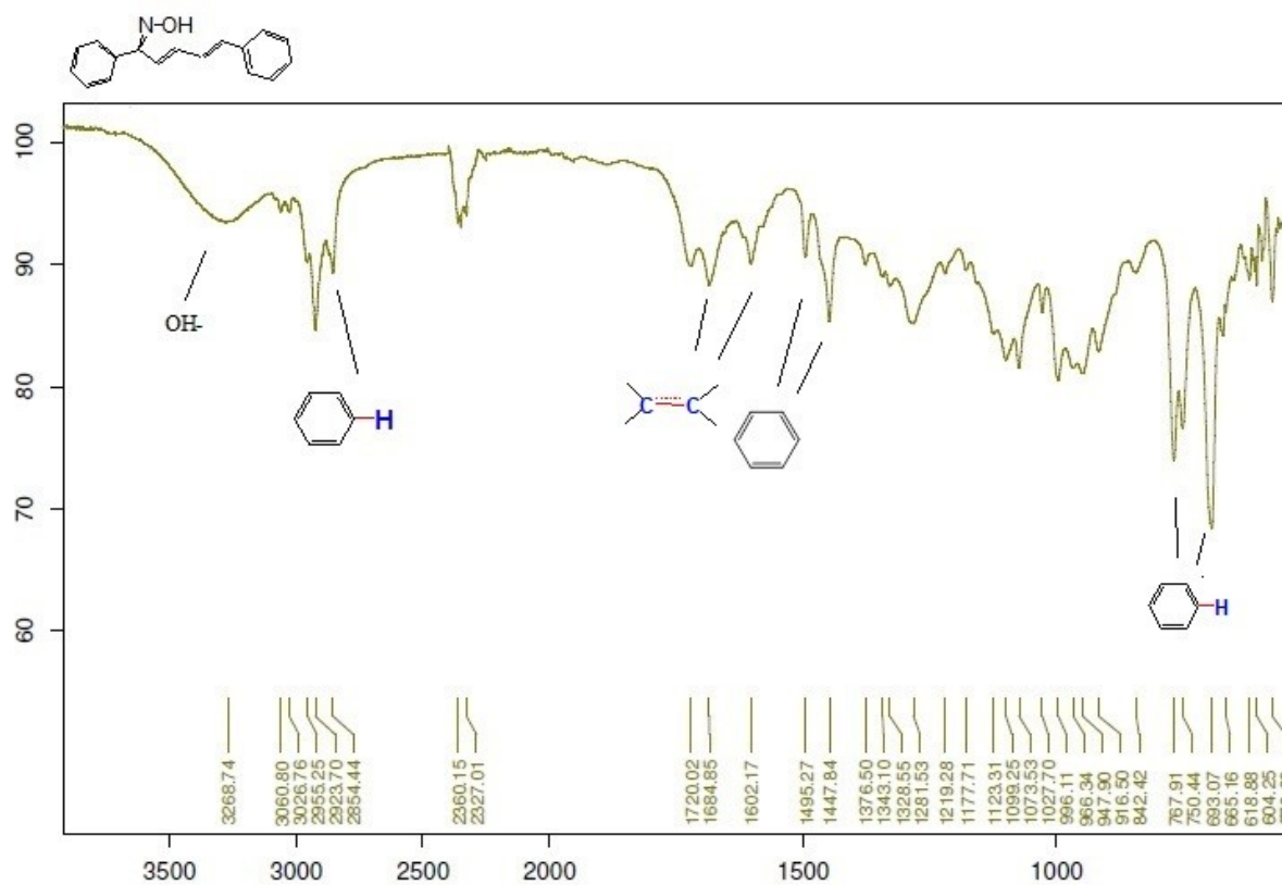
A.8: IR spectra of 1,5-diphenylpenta-(2E,4E)-dien-1 oxime [XXXVII-b]
