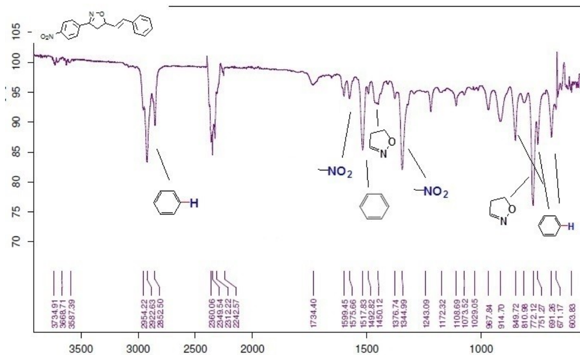
A.8: IR spectra of 1,5-diphenylpenta-(2E,4E)-dien-1 oxime [XXXVII-b]
