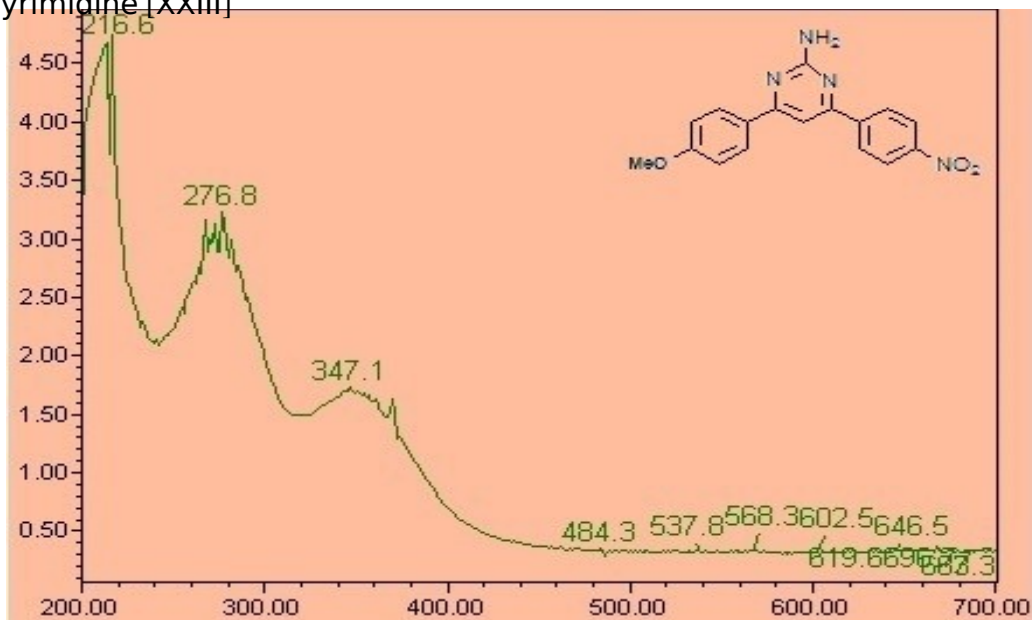
D.4: UV-Vis spectra of 2- amino 4-( p -nitrophenyl)-6-( p -methoxyphenyl) pyrimidine [XXIII]
