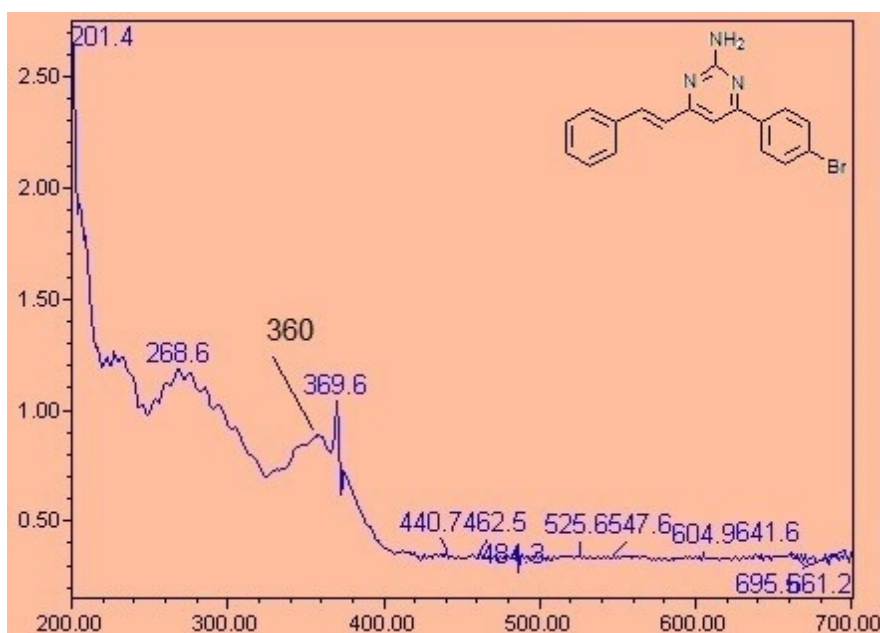
D.3: UV-Vis spectra of 2- amino 4-( p -bromophenyl) 6-(ethenyl-2-phenyl) pyrimidine [XXI]
