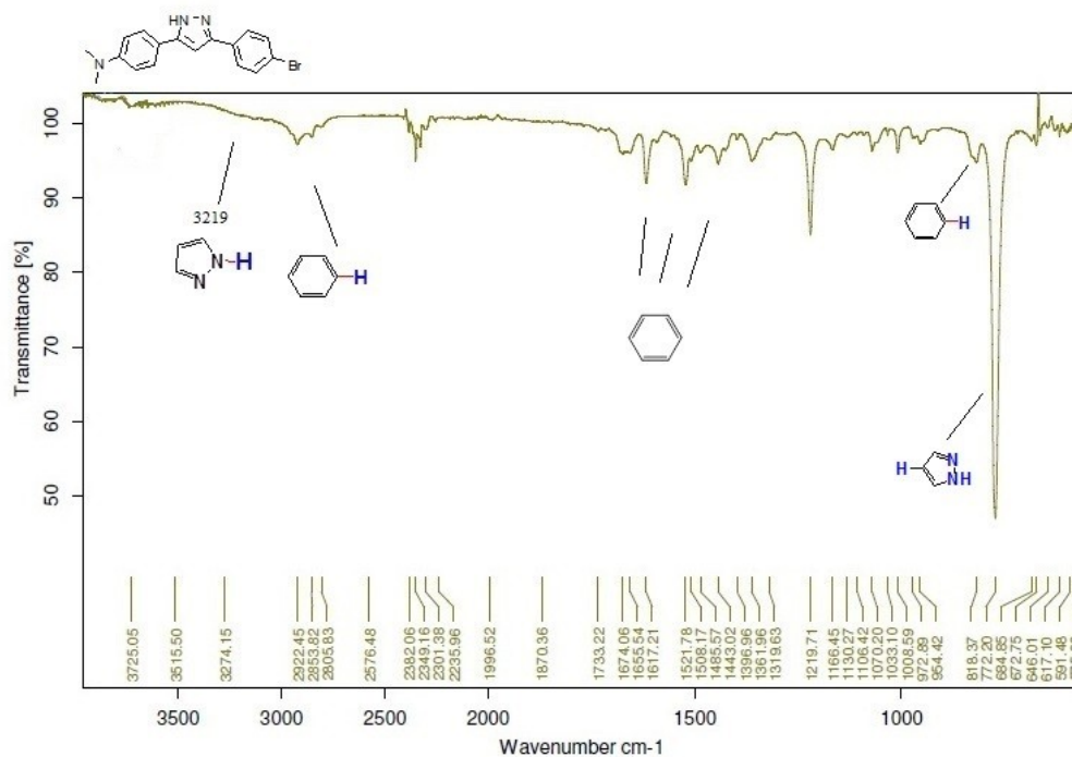
A.6: IR spectra of 3-( p -nitrophenyl)-5-(ethenyl-2-phenyl)-pyrazole [XXXIII]
