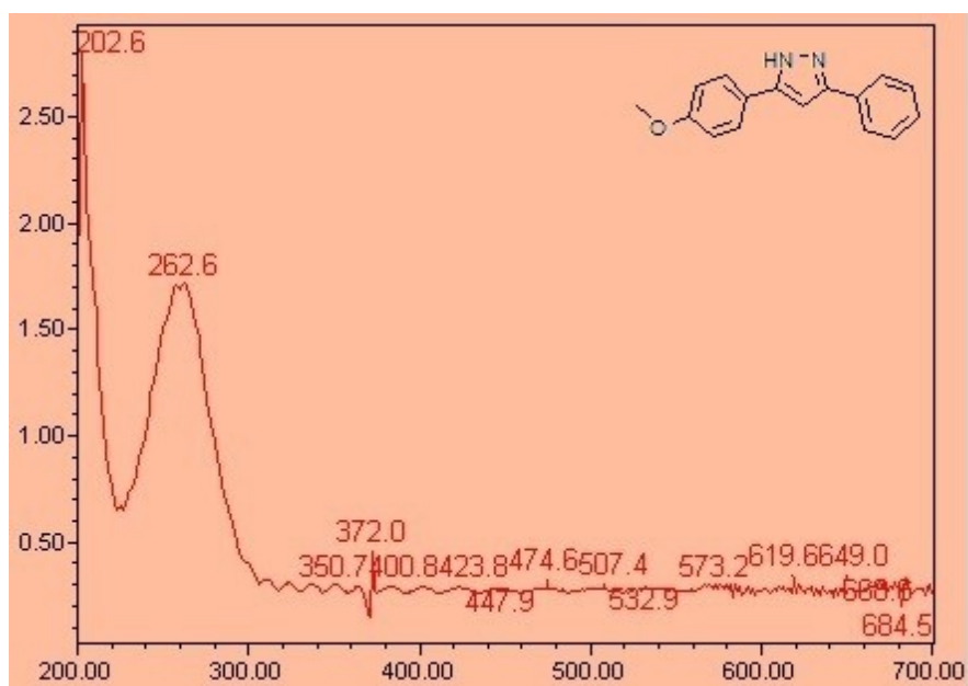
D.6: UV-Vis spectra of 3-phenyl-5-( p -methoxyphenyl)- pyrazole [XXVII]
