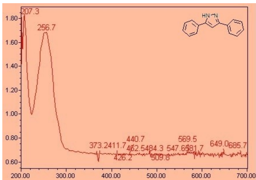
D.5: UV-Vis spectra of 3,5-diphenyl-pyrazole [XXV]
