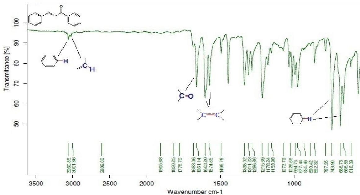
A.1: IR spectra of 1,3-diphenyl-(2E)-propen-1-one [I]
