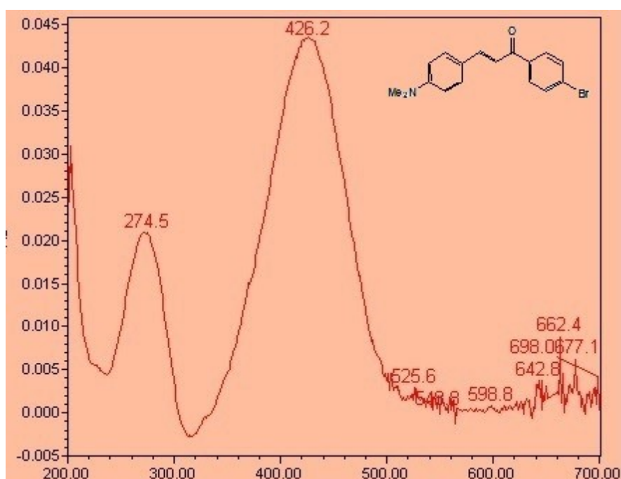
D.2: UV-Vis spectra of 1-( p -bromophenyl)-3-( p -N,N dimethylaminophenyl)-(2E)-propen-1-one [VI]
