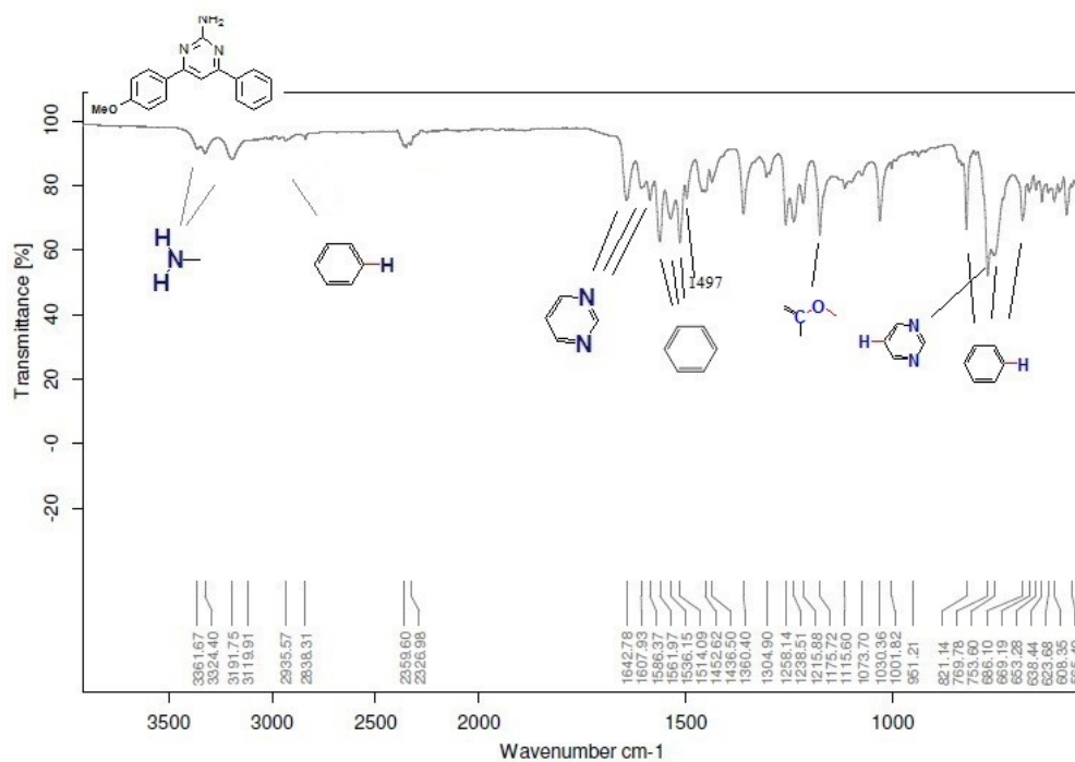
A.3: IR spectra of 2- amino 4-( p -methoxyphenyl) 6-phenyl pyrimidine [XVII]
