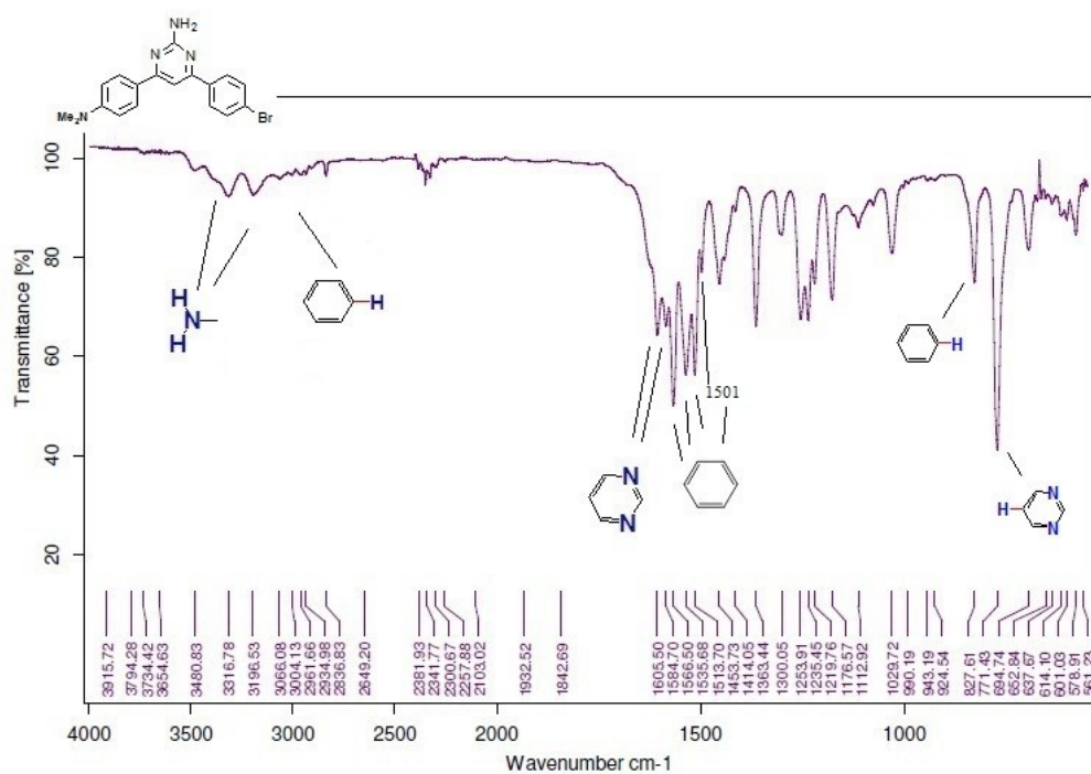
A.4: IR spectra of 2- amino 4-( p -methoxyphenyl) 6-phenyl pyrimidine [XVII]
