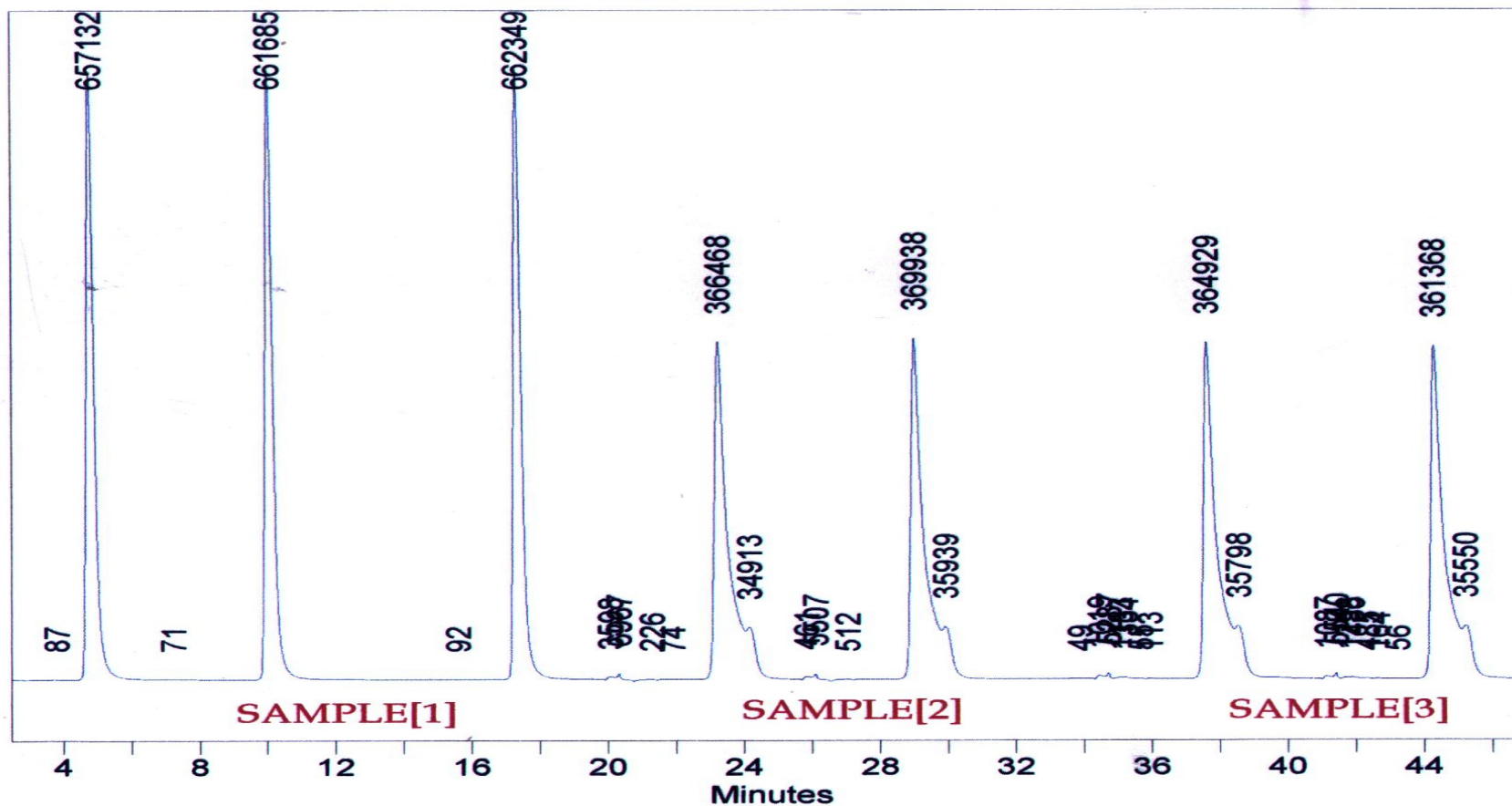
Figure: 3.26 HPLC. Chromatogram of Metronidazole benzoate in methanol. The effect of temperature (50 °C) on the stability thermostated and dissolved in methanol/water.
