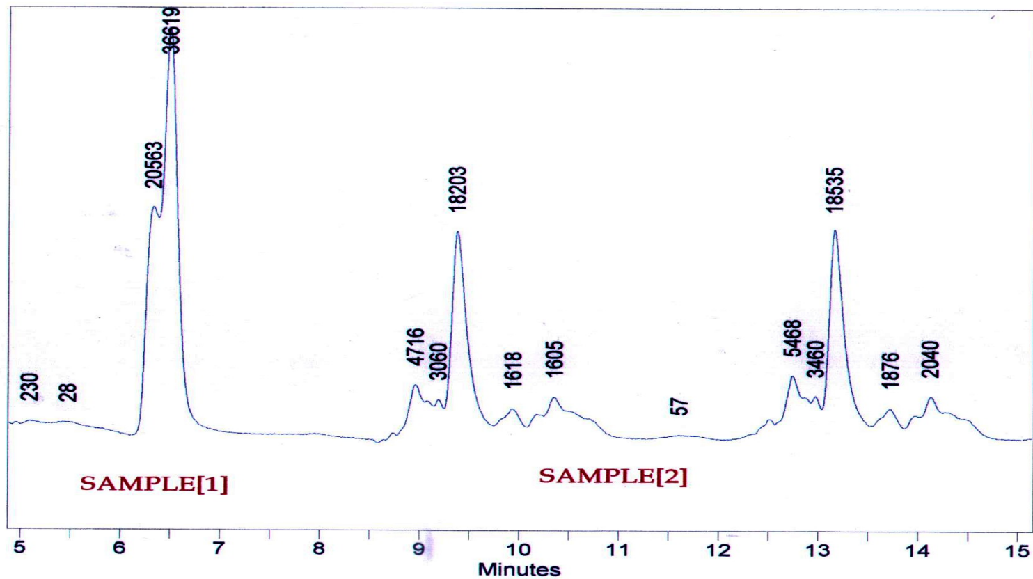
Figure: 3.20 HPLC. Chromatogram of Metronidazole benzoate. The effect of acid media (1MHCl) on photo degradation.
