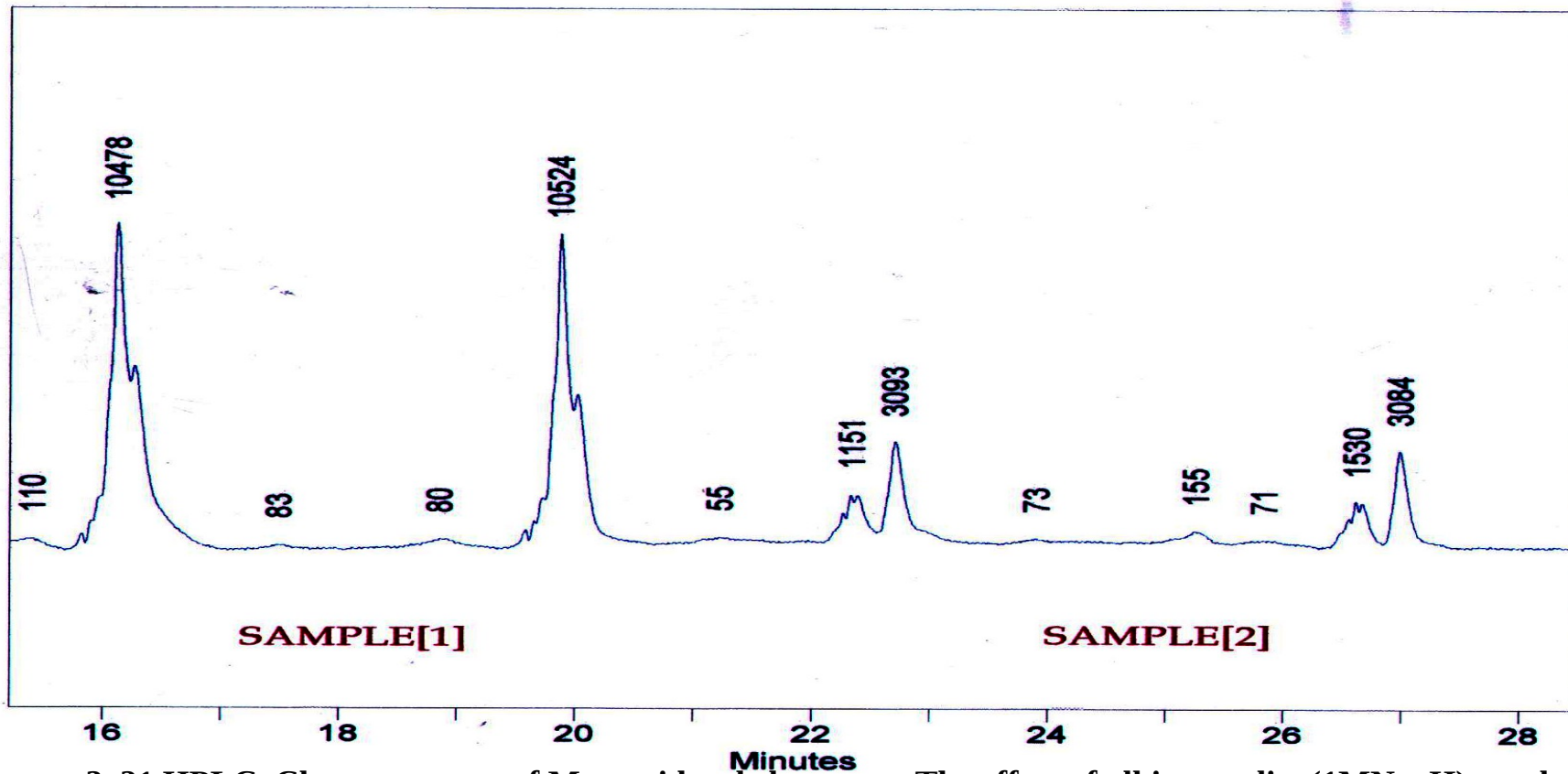
Figure: 3. 21 HPLC. Chromatogram of Metronidazole benzoate. The effect of alkine media (1MNaOH) on photo degradation.
