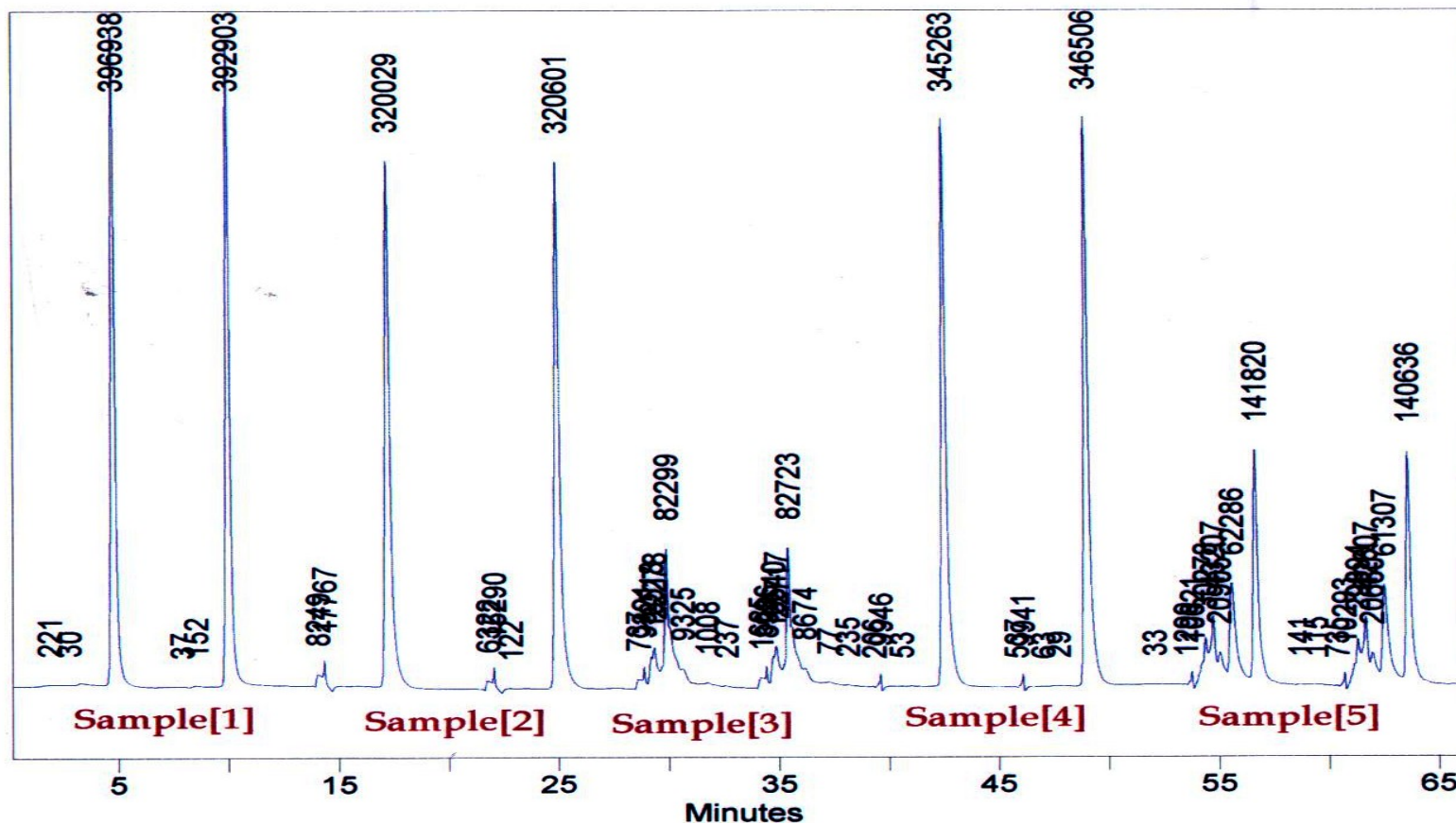
Figure: 3. 17.HPLC. Chromatogram of Metronidazole benzoate. The effect of concentration (0.1% and 0.5%) dissolved in methanol on the photo degradation.
