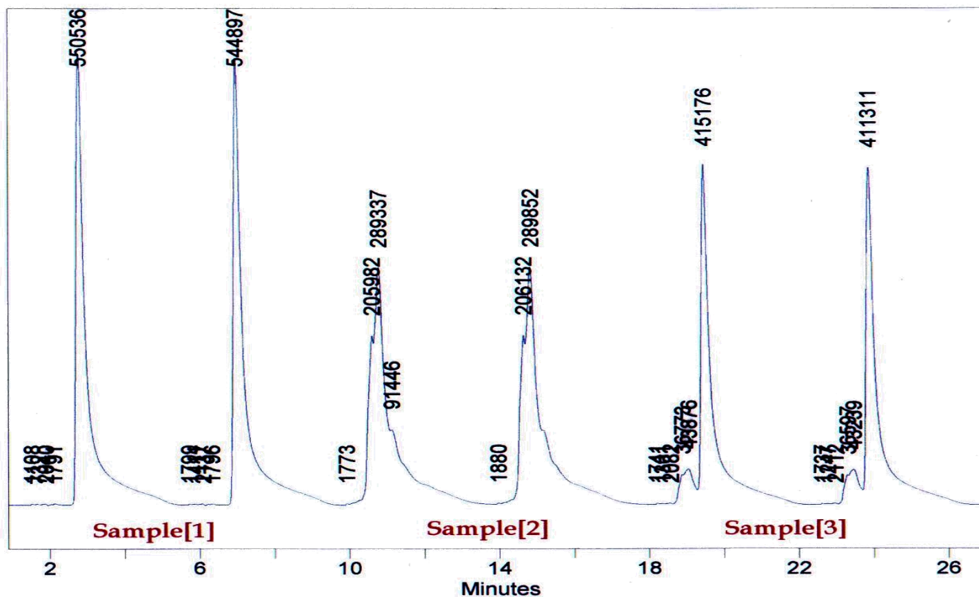
Figure: 3. 16. HPLC Chromatogram of Metronidazole benzoate. The effect of concentration (0.1% 1.0%) dissolved in methanol on the photo degradation.
