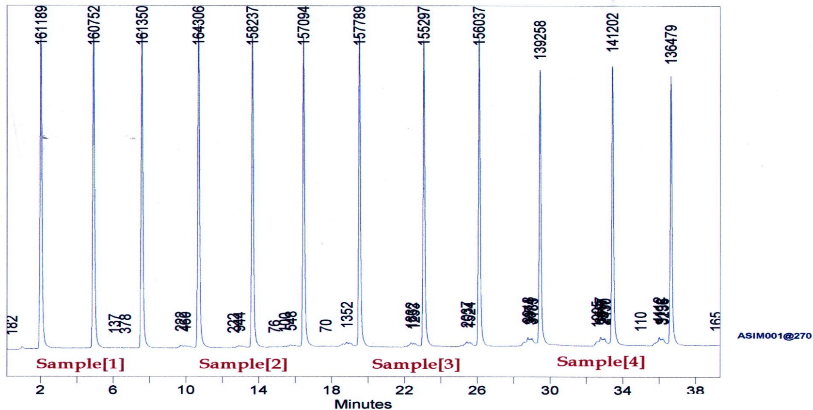
Figure: 3.15 HPLC. Chromatogram of Metronidazole benzoate powder decomposed samples.
