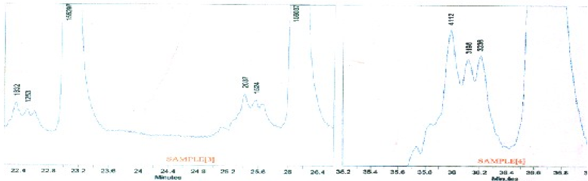
Figure: 3.14 HPLC. Chromatogram of Metronidazole benzoate powder decomposed samples
