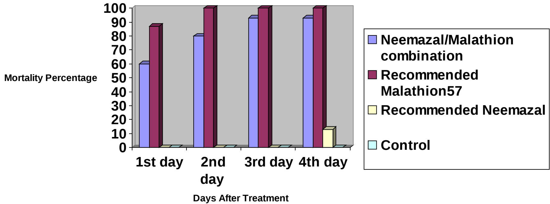
(Figure 7: the effect of NeemAzal-T/S and Malathion57 combination against the Adults of Tribolium castaneum Var. (herbst
