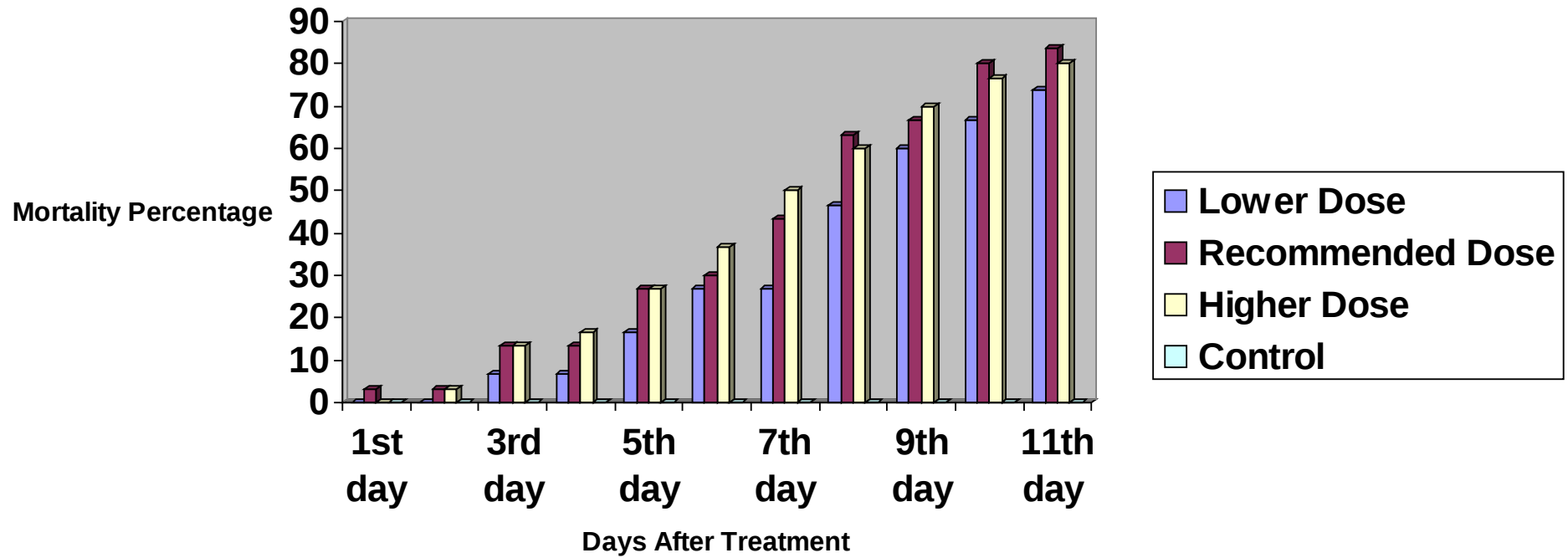
(Figure 2: the effects of NeemAzal T-/S against the larvae of Tribolium Castaneum Var. (herbst
