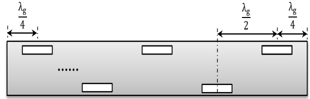
Fig. 1. Structure of the resonating vertically polarized SWAA.
