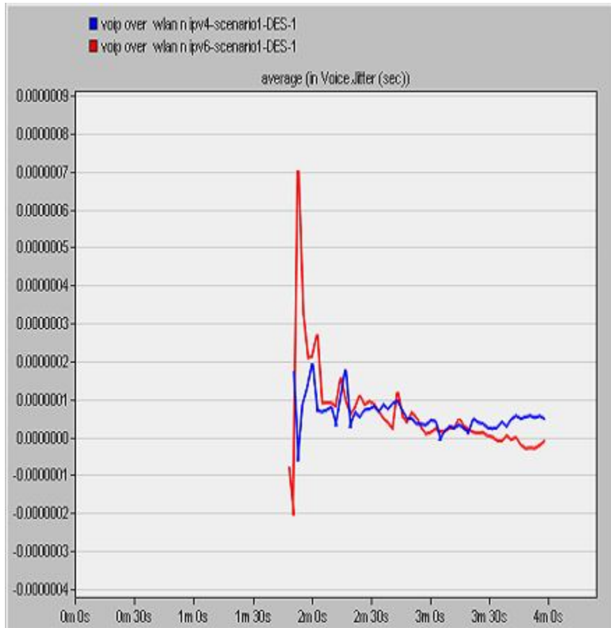
Figure (4.10) Jitter 802.11 n_ipv4, 6
