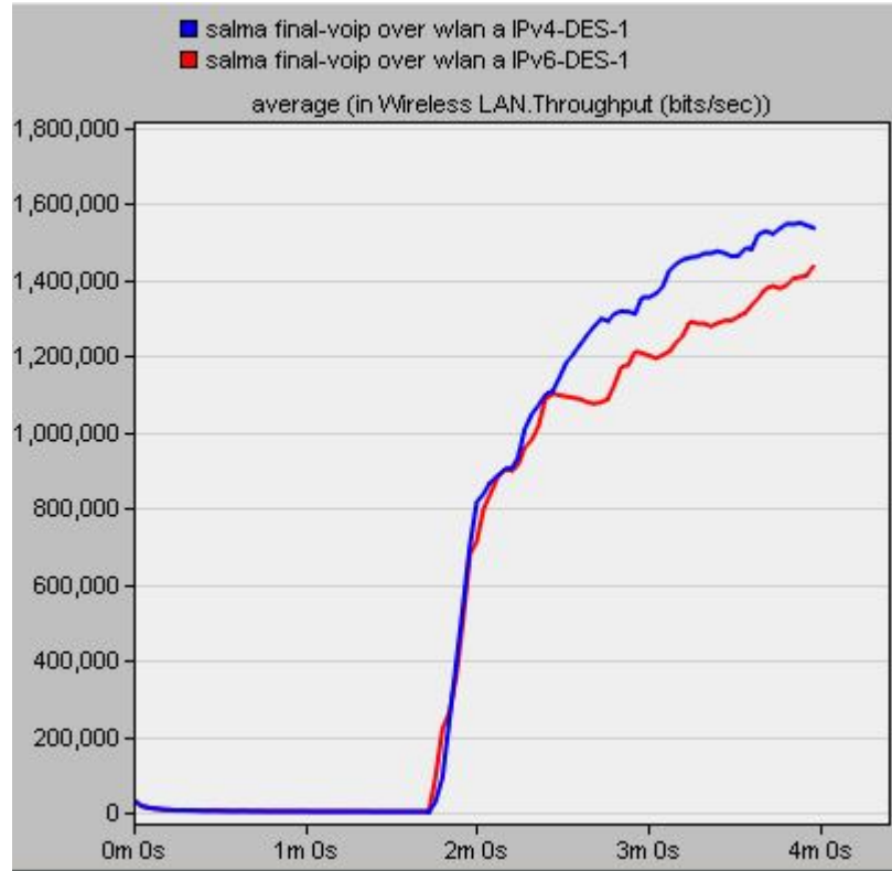
Figure (4-3) Throughput 802.11a_ipv4 , 6
