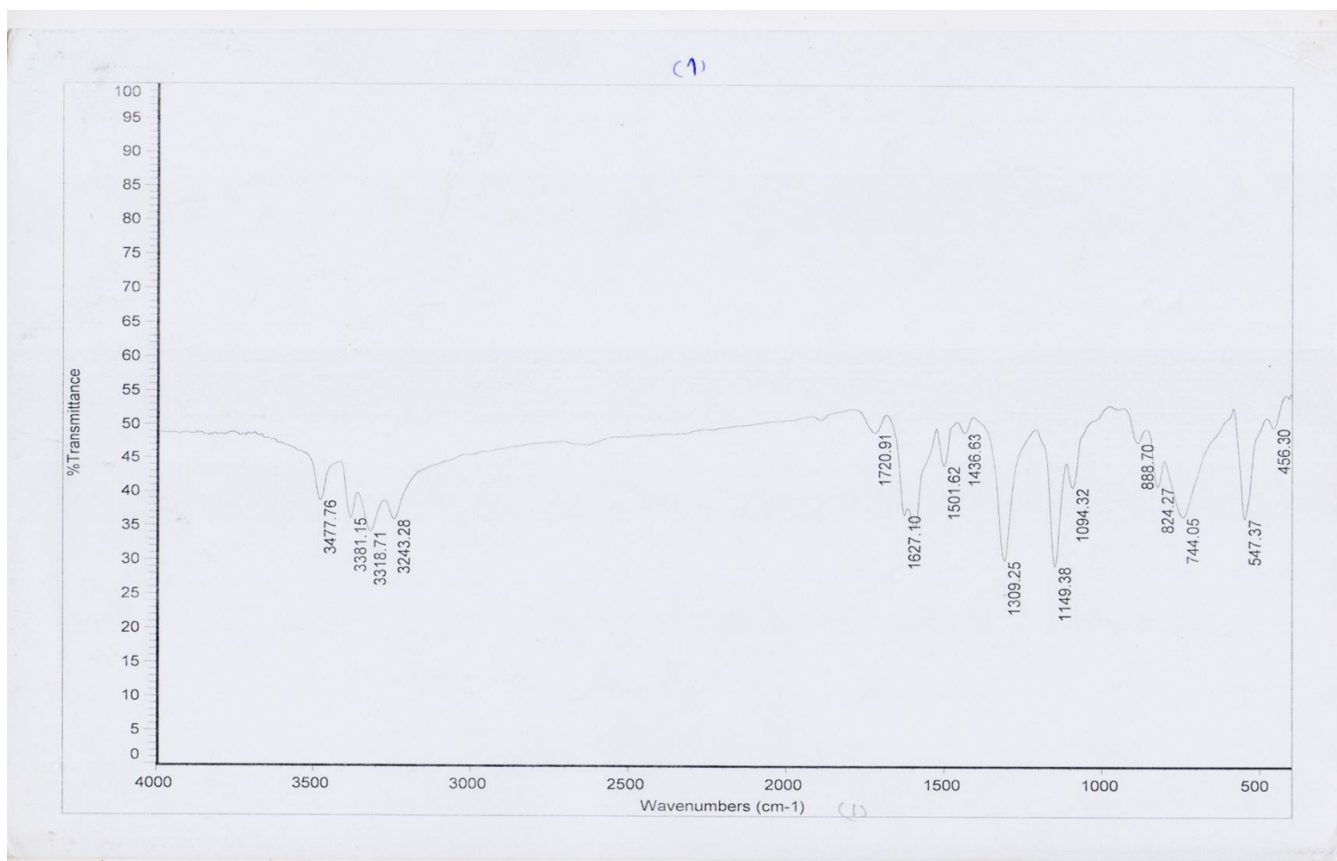
I diethyl 2,6-dimethyl-1-(4-nitrophenyl)-1,4-dihydropyridine-3,5-dicarboxylate
