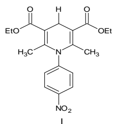
I diethyl 2,6-dimethyl-1-(4-nitrophenyl)-1,4-dihydropyridine-3,5-dicarboxylate
