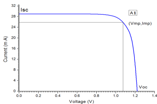
Figure 13: The IV curve for sample A1.
