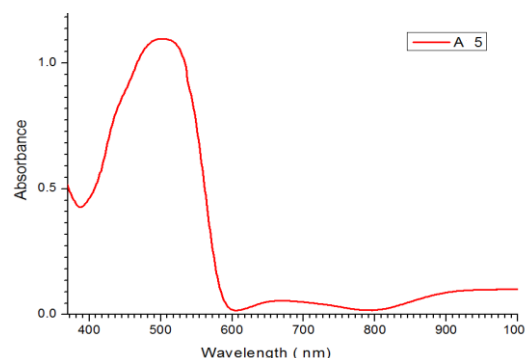
Figure 11: The absorbance measured of sample A5.
