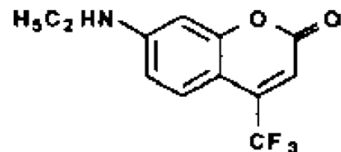
Figure 3: The structure of Coumarin 500.
