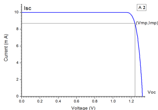
Figure 14: The IV curve for sample A2.
