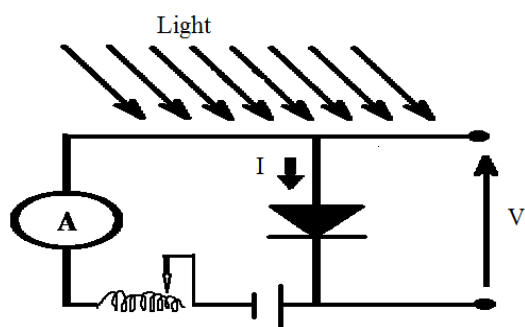
Figure 6: The setup for measuring the IV characteristics of solar cells.
