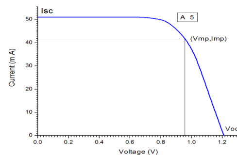
Figure 17: The IV curve for sample A5.
