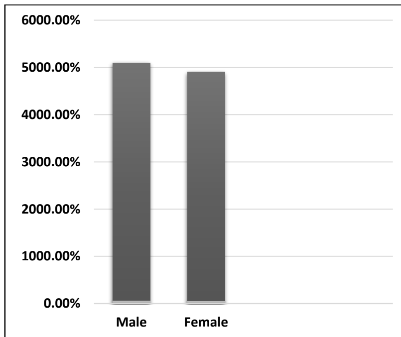
Figure 4.1 Gender distribution.
