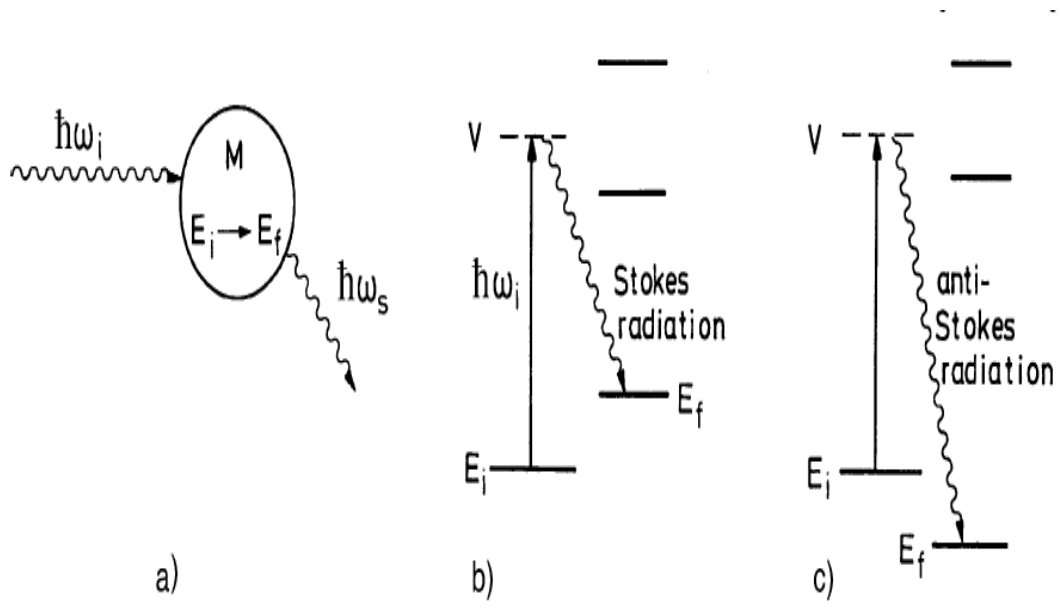
1.5: Schematic level diagram of Raman scattering
