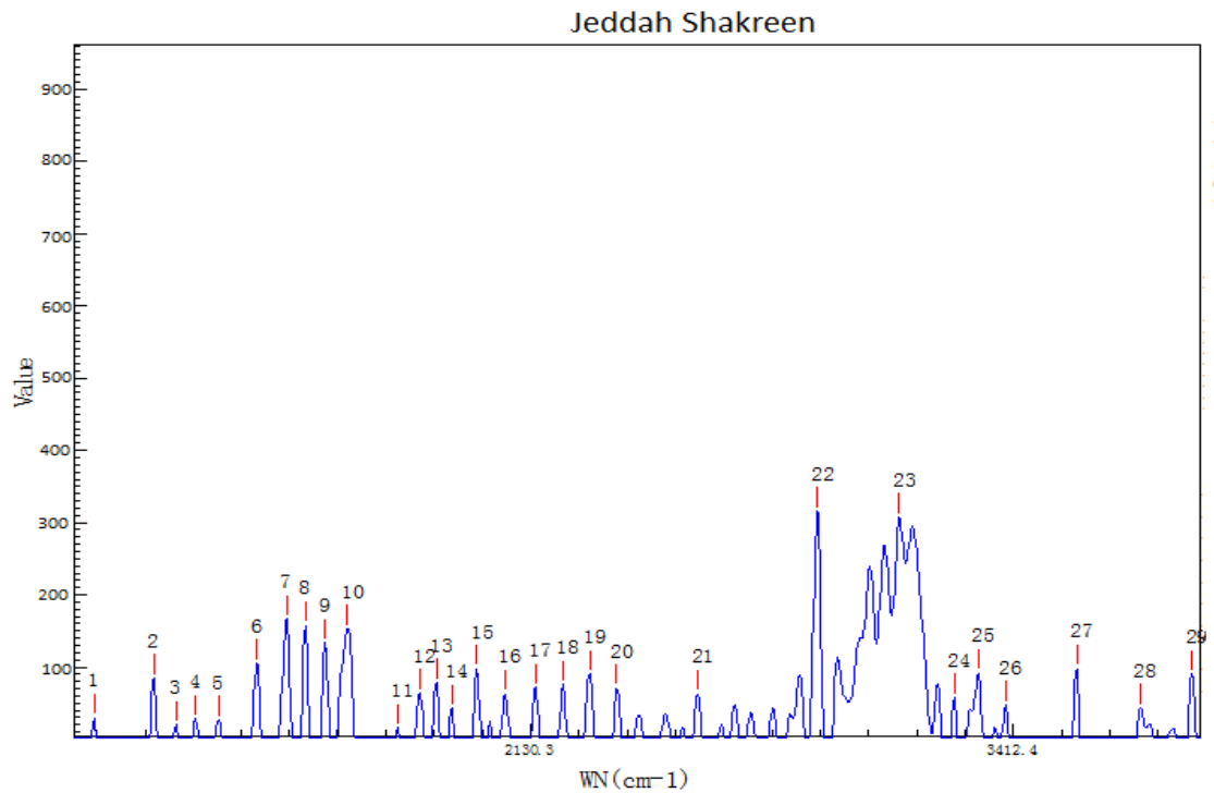
Figure (4.5) Raman spectrum of ground water collected from S 5 (Jeddah Shakreen) in the range from 769.2 to 3838.1 cm -1
