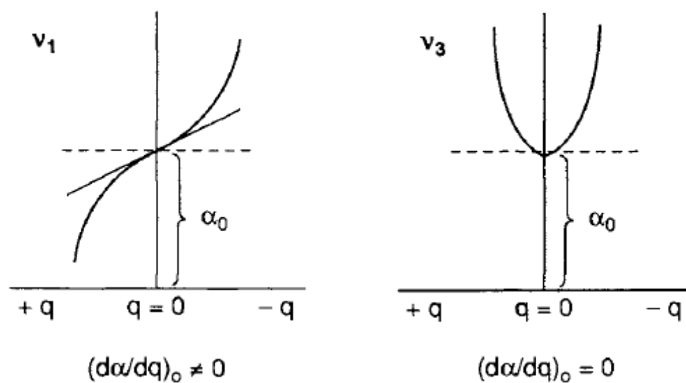
Figure 2.5: Difference between \nu_1 and \nu_3 vibrations in \text{CO}_2 molecule.
