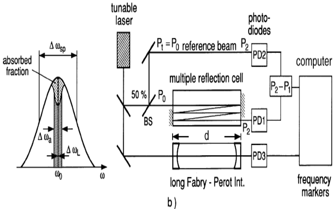
Figure 1.1: Comparison between absorption spectroscopy with a broadband incoherent source (a) and with a tunable single-mode laser (b)
