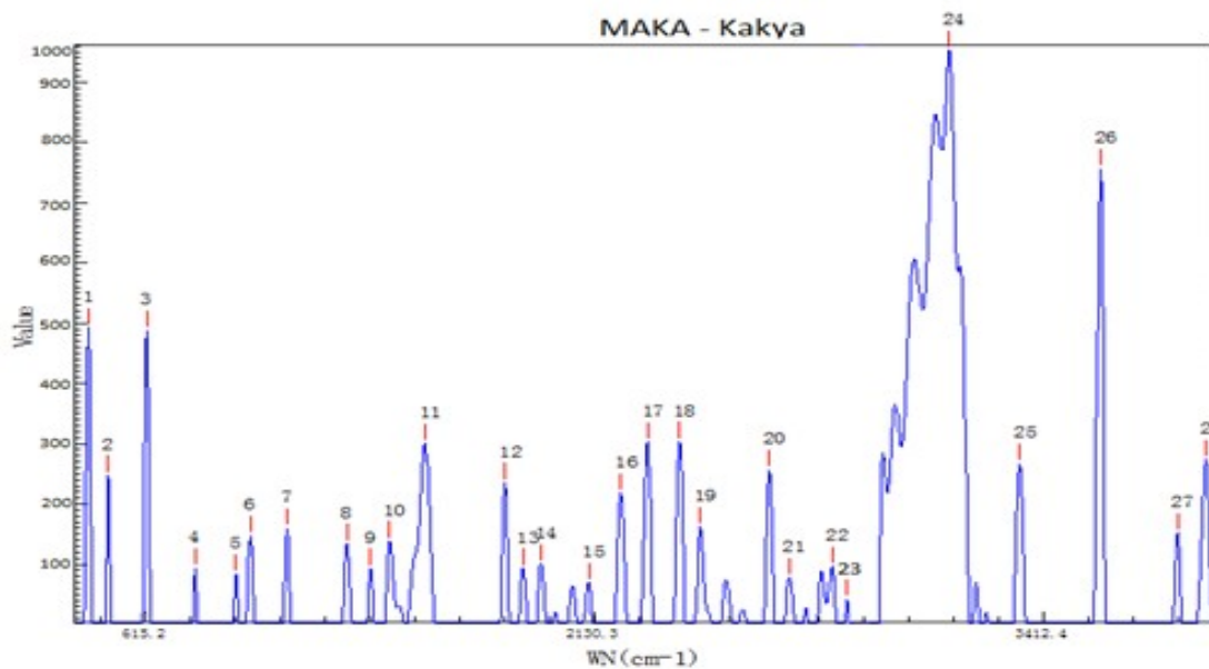
Figure (4.10) Raman spectrum of ground water sample S_{10} collected from (Makah Kakya) in the range from 407.9 to 3831.4 \text{cm}^{-1} .
