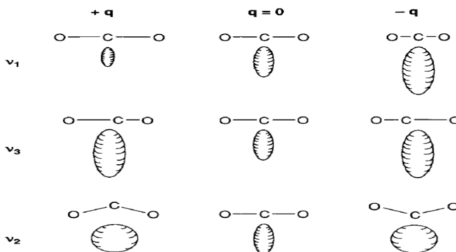
Figure (2.4): Changes in polarizability ellipsoids during vibration of \text{CO}_2 molecule.
