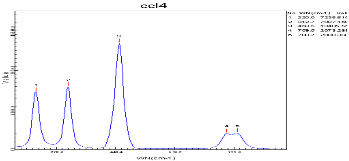
Figure 3.6: Raman spectrum of \text{CCl}_4 sample
