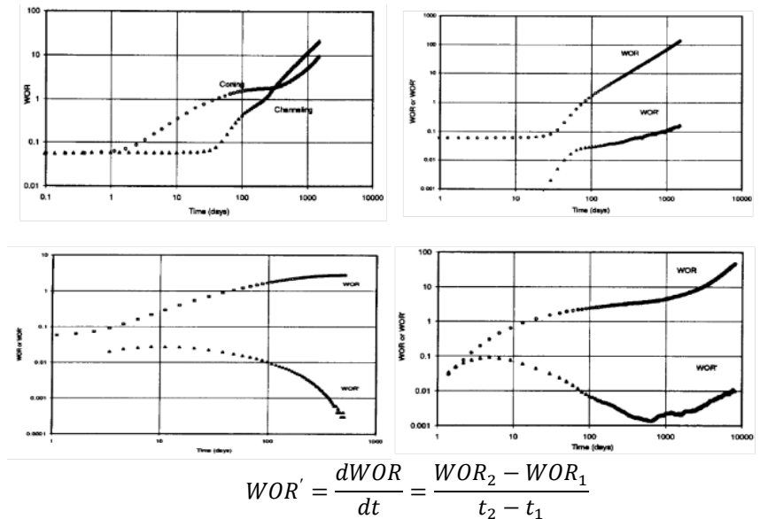
Figure 5: water control Diagnostic plots After [1]
