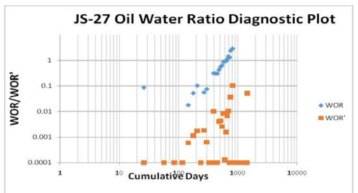
Channeling
