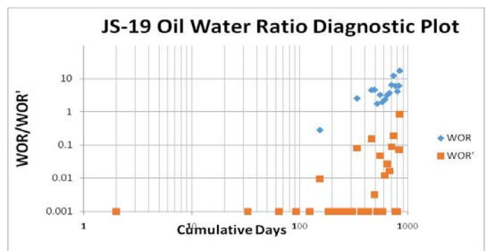
channeling
