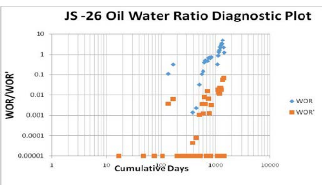
Channeling
