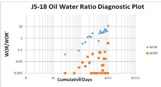
Bottom water conning
