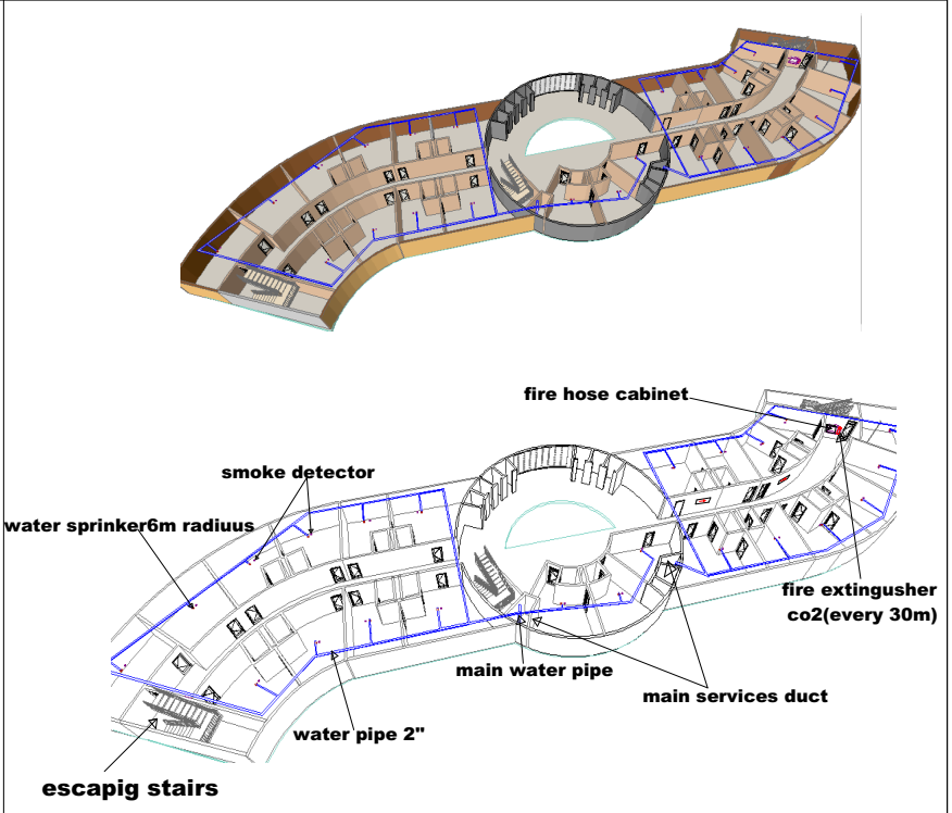
ROOMSPRESEPECTIVE FIRE PROTECTION
