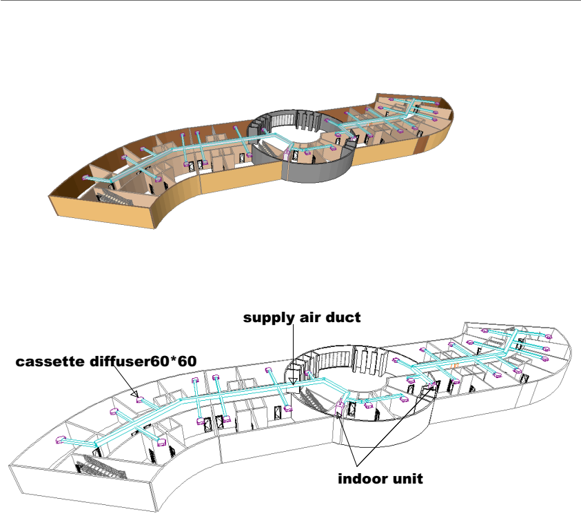
ROOMS PERSPECTIVE HVAC
